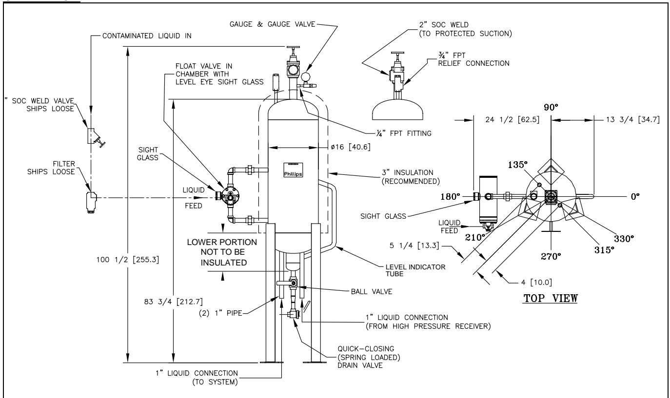
Figure 7: Anhydrator, shown assembled with optional valves
