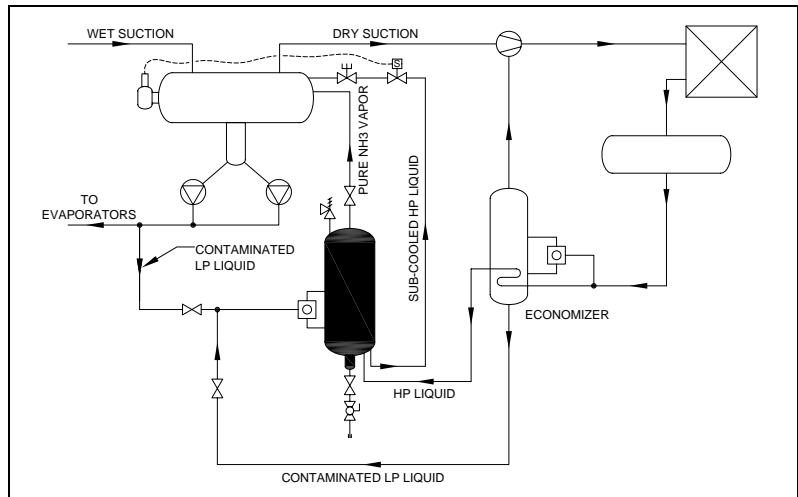
Figure 5: Anhydrator used with Economizer
