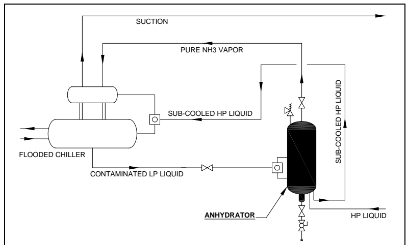
Figure 6: Anhydrator used with Flooded Chiller
