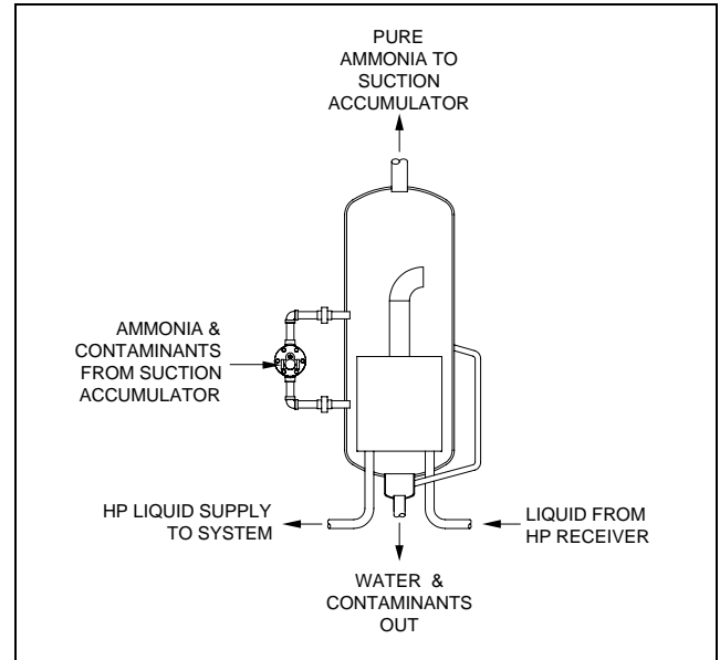
Figure 1: Flow through the Anhydrator (Unit shown with 300HM Float Valve)
