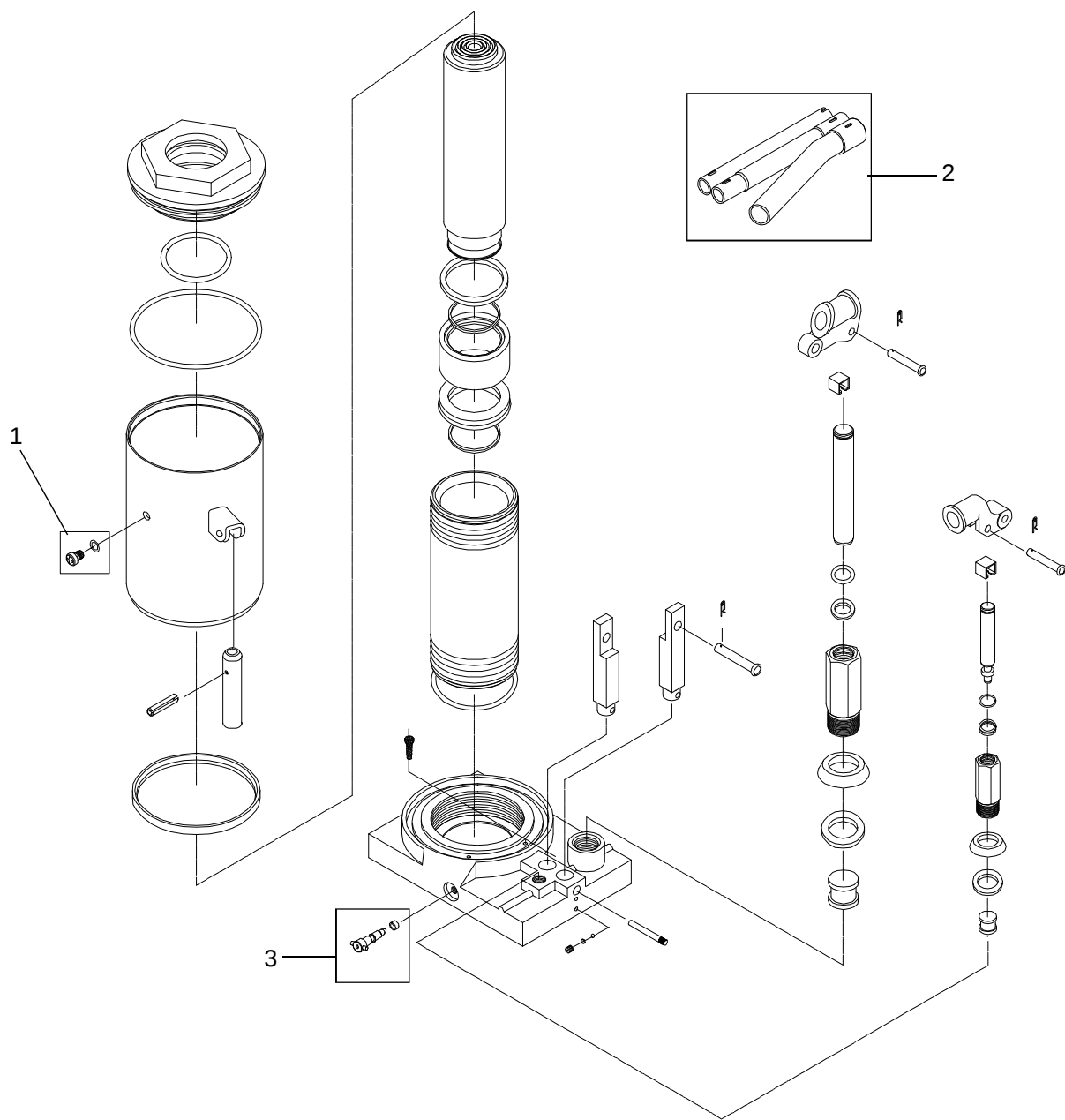
Figure 4 - Model 10500 Replacement Parts Illustration
