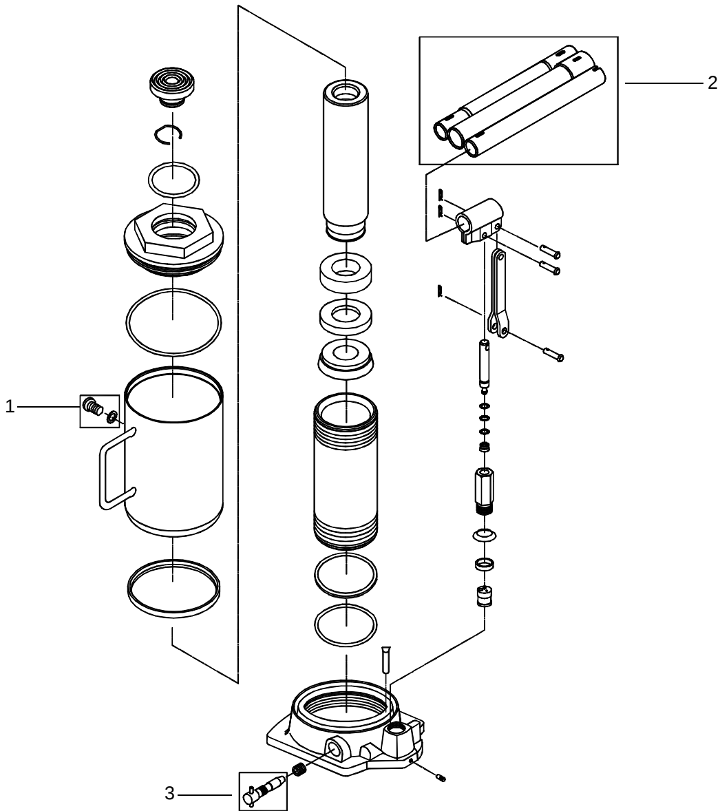
Figure 3 - Model 10300 Replacement Parts Illustration
