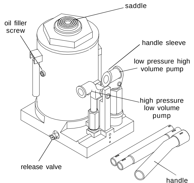
Figure 2 - 10500 Nomenclature
