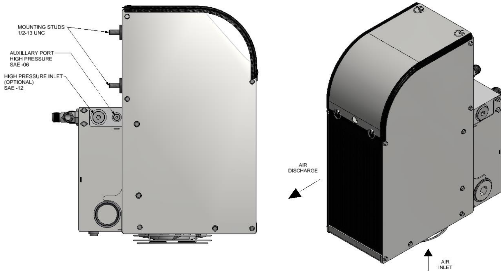
FIGURE 2-2 – AIR FLOW DIRECTION AND OUTLINE
