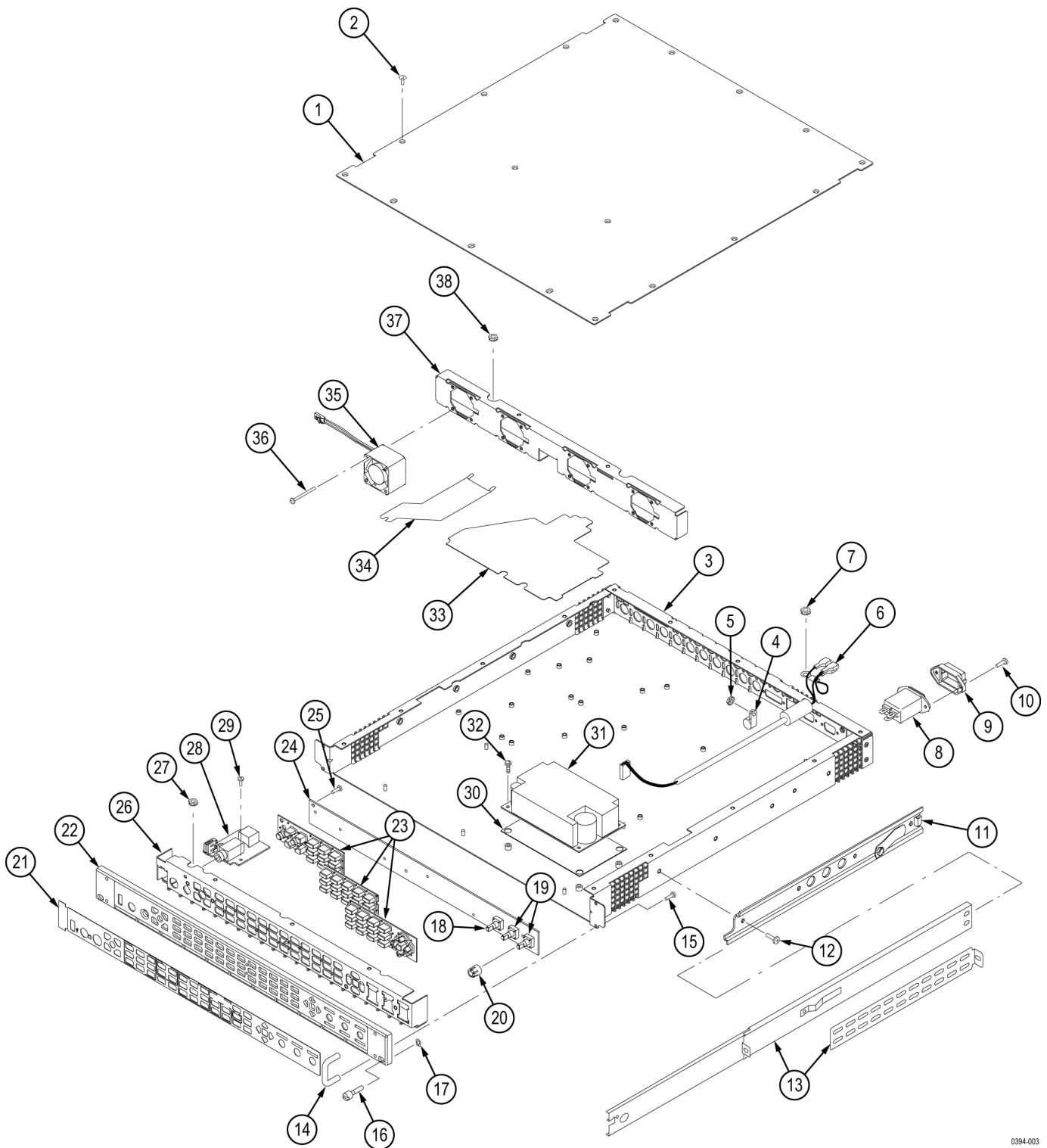
Figure 5-1: Replaceable parts (standard)
