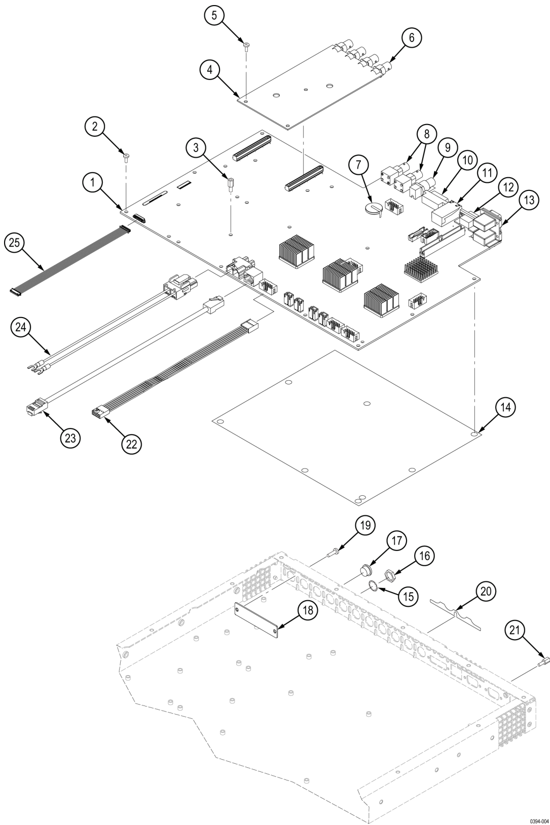
Figure 5-2: Replaceable parts (standard)
