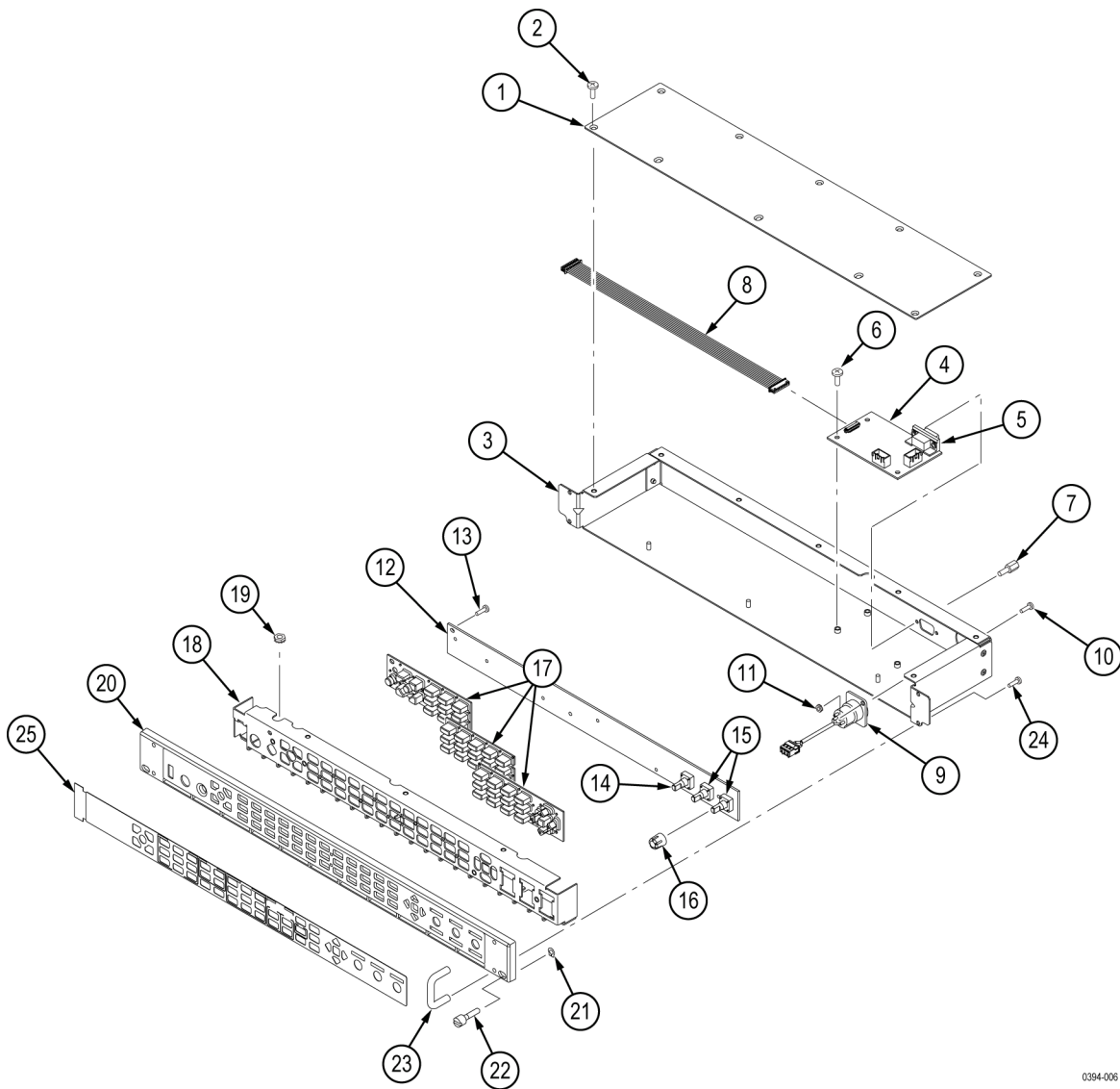
Figure 5-4: Replaceable parts (WVR8RFP Remote Front Panel)
