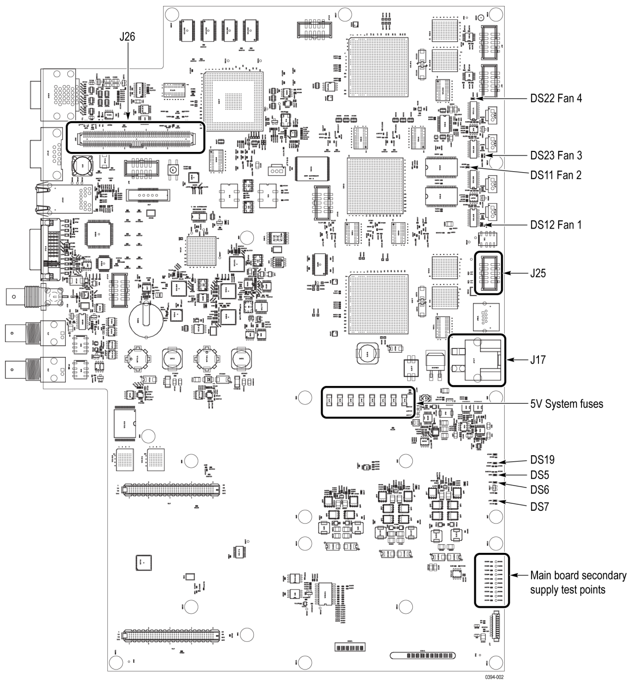
Figure 4-1: Main board indicator LED, connector, and test point locations
