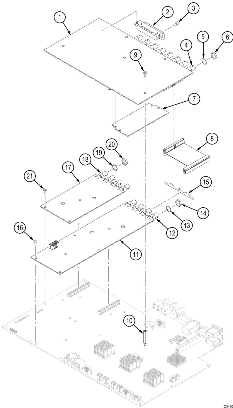
Figure 5-3: Replaceable parts (options)
