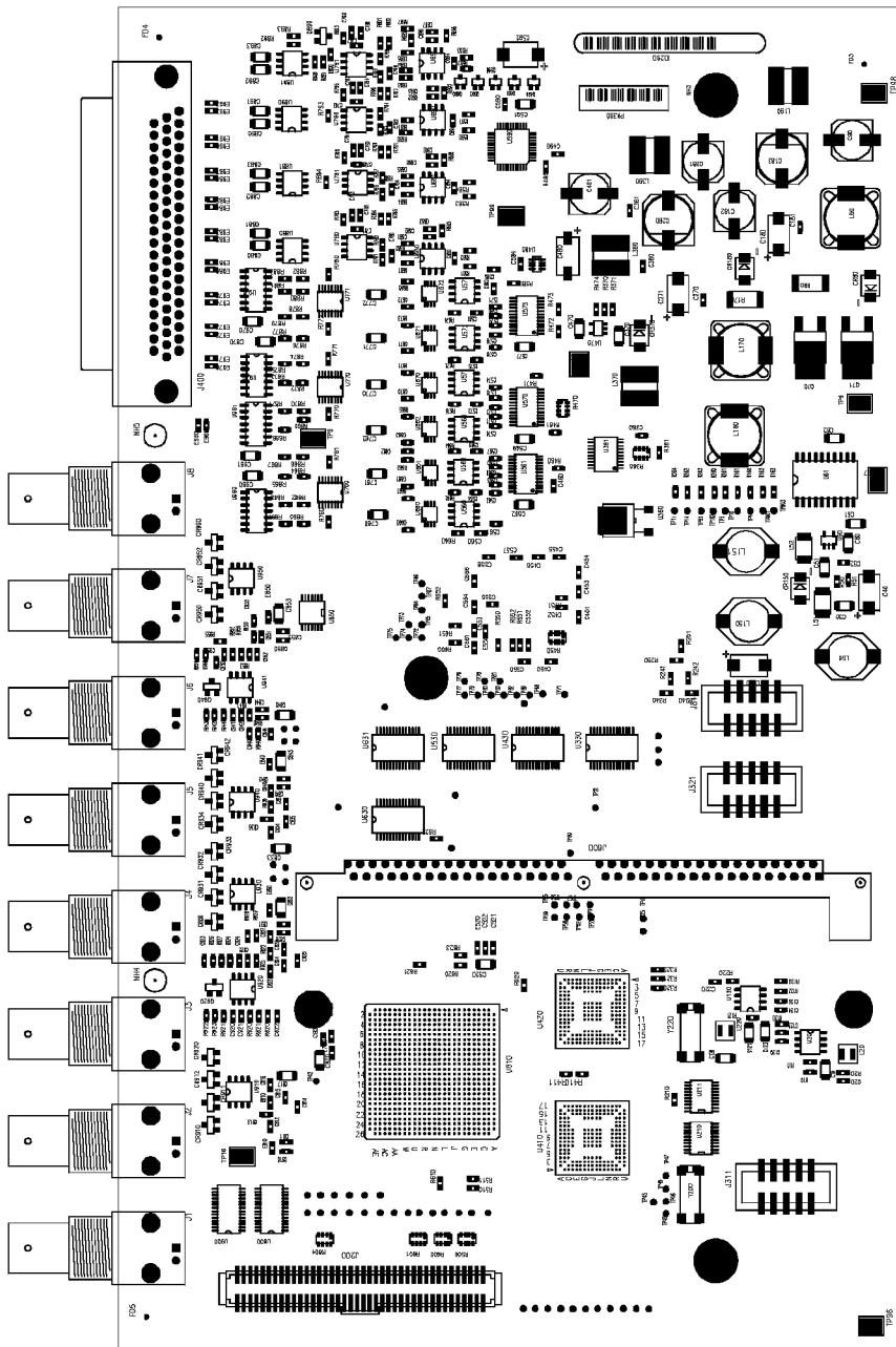
Figure 4-2: Options AD and DPE Audio board, component side
