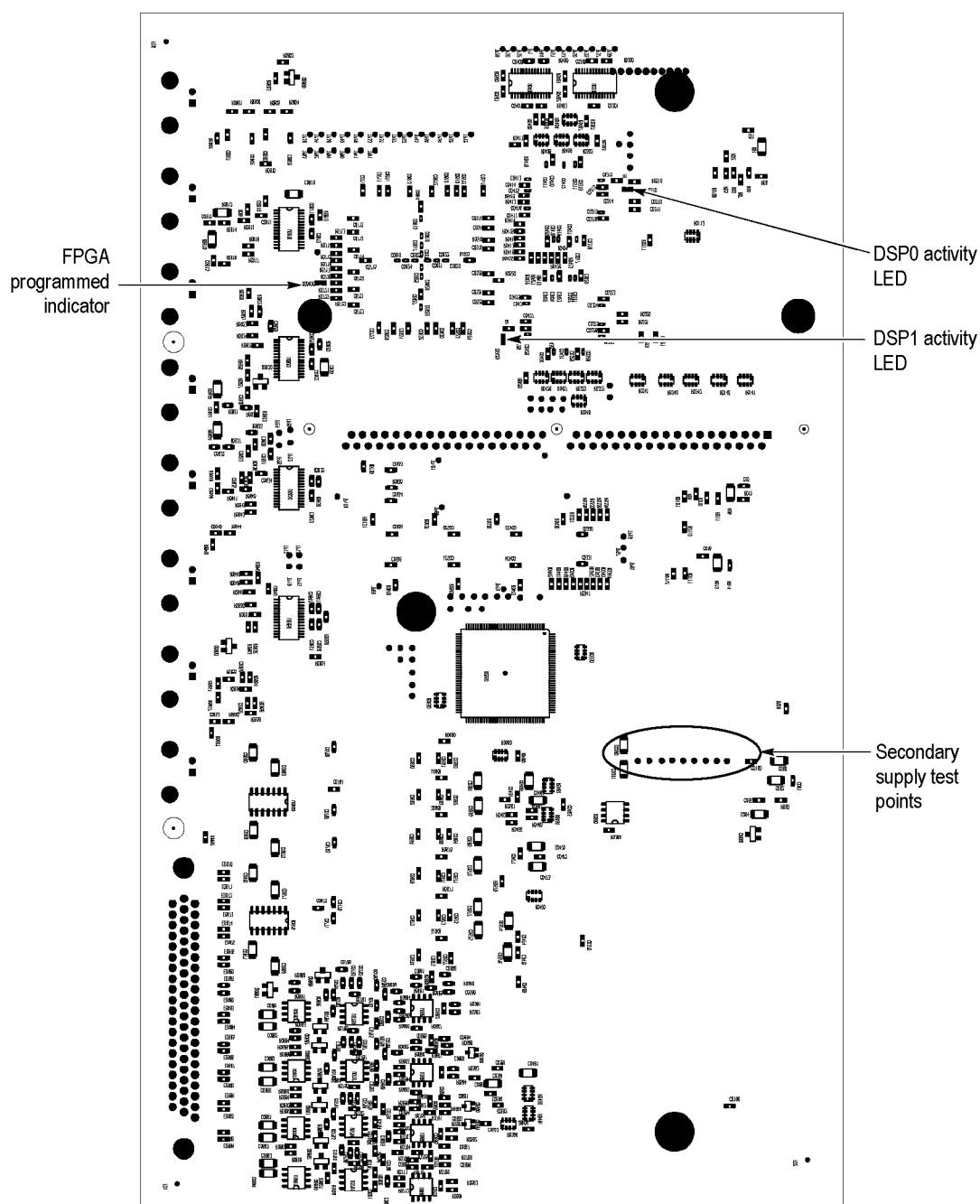
Figure 4-3: Options AD and DPE Audio board back side indicator LED and test point locations
