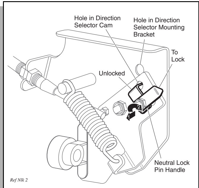
Fig. 14 Neutral Lock on Direction Selector
