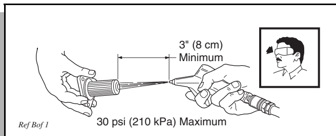
Fig. 24 Blowing Out Oil Filter
