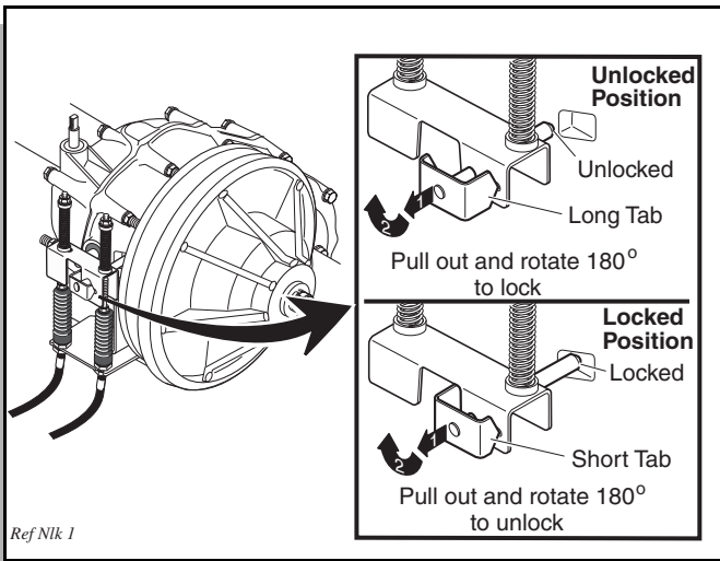
Fig. 13 Neutral Lock on Rear Axle
