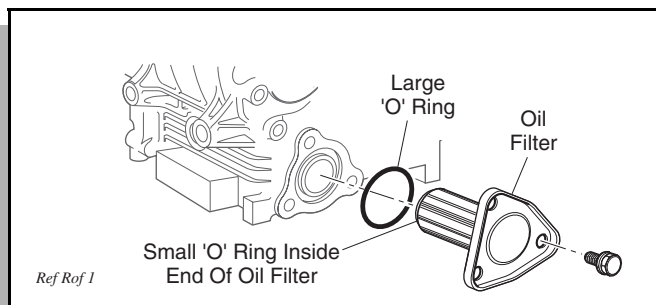
Fig. 22 Remove Oil Filter
