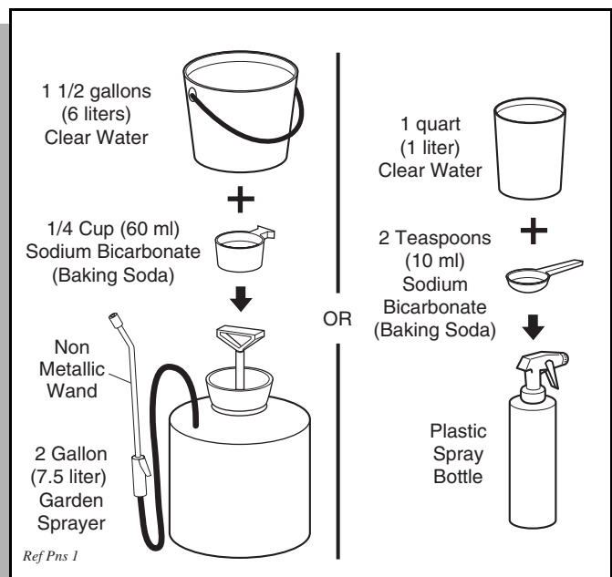
Fig. 29 Preparing Acid Neutralizing Solution
