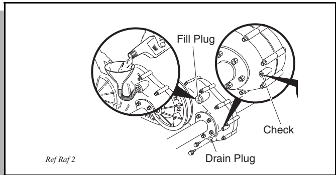
Fig. 33 Add, Check and Drain Rear Axle Lubricant
