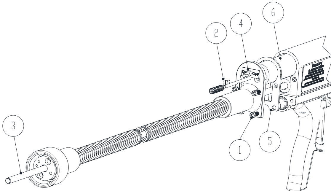
Figure 17: High Voltage Cable and Electric motor Removal Diagram
