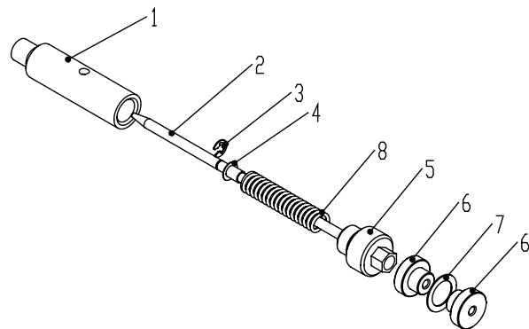
Figure 20: Needle Assembly Diagram
