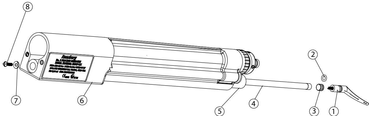
Figure 22: HV Resistor Removal
