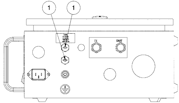
Figure 25: Fuse Location
