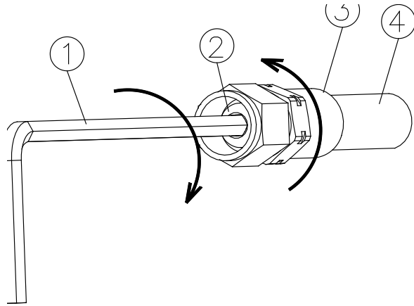
Figure 5: Fluid Fitting Assembly Procedure
