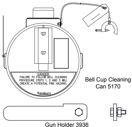
Figure 8: Bell Cleaning Can and Gun Holder
