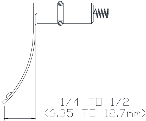
Figure 9-1: Un-Installed Brush Shape
