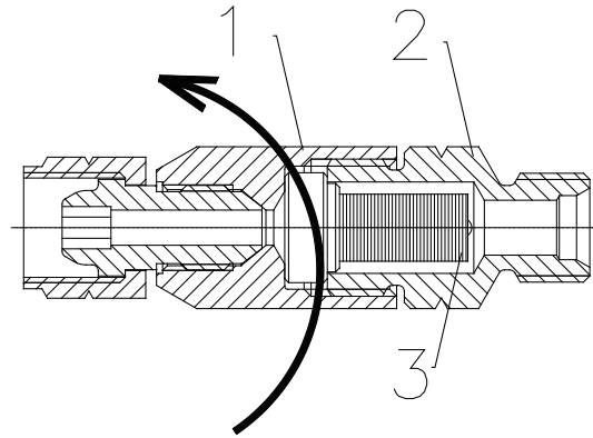
Figure 16: Fluid Filter Replacement
