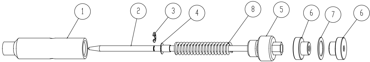
Figure 29: Needle Valve Assembly Parts
