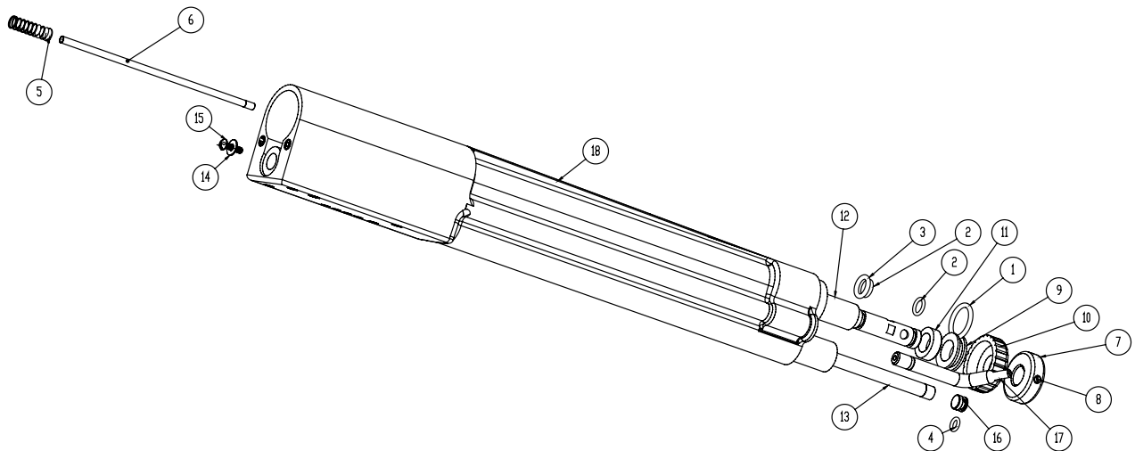
Figure 30: Barrel Parts List
