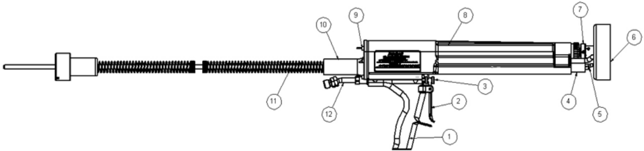
Figure 1: Gun Features / Model 19372-XX
