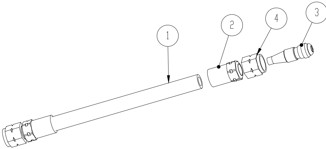
Figure 31: 8340-XX Fluid Hose Parts and Assemblies
