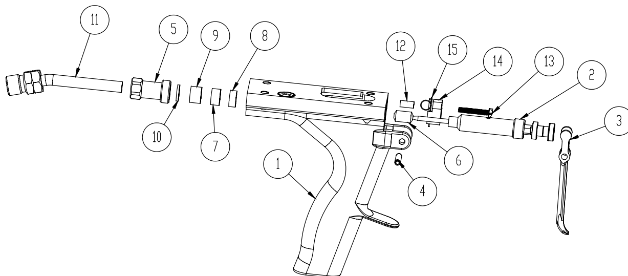
Figure 28: 7233-00 Handle Parts List
