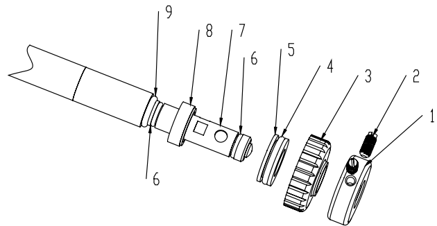
Figure 24: Ceramic Seal Replacement
