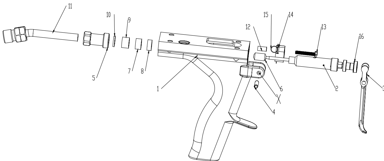
Figure 19: Handle Assembly Diagram
