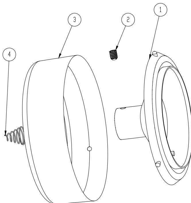
Figure 35: Bell Spare Parts and Assemblies
