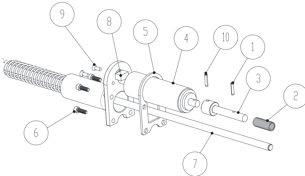
Figure 27: Cable /Motor Parts List
