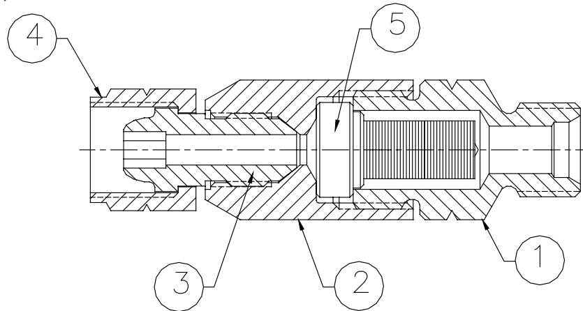
Figure 34: Fluid Filter Parts
