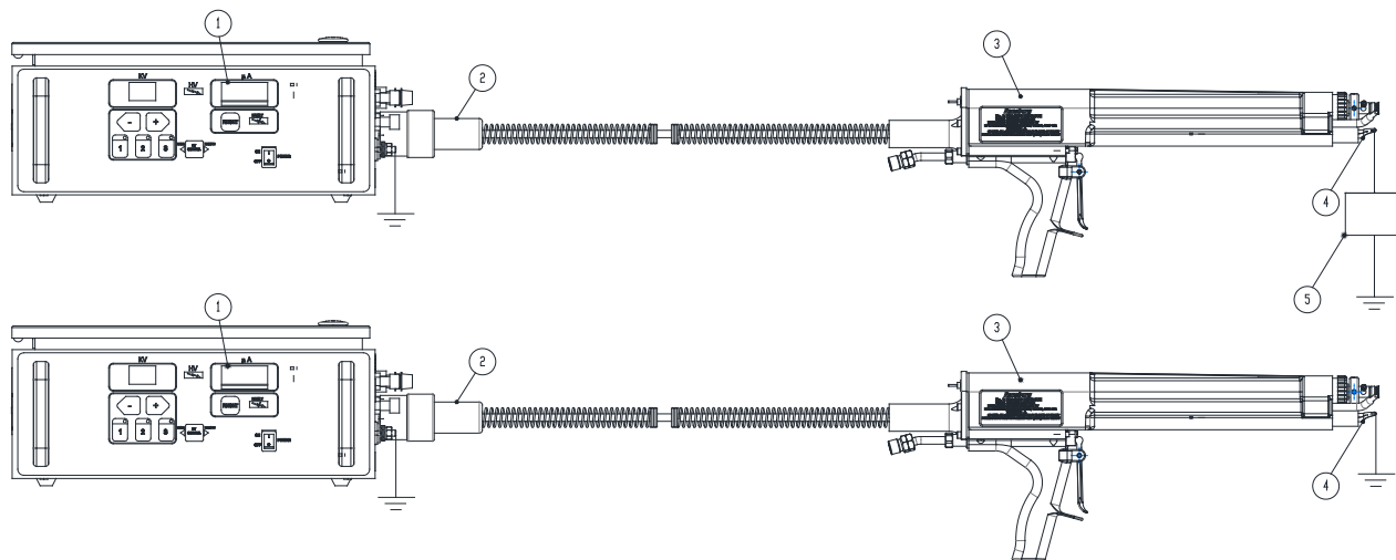
Figure 14: No. 2 Handgun Short Circuit Current Test Diagram
