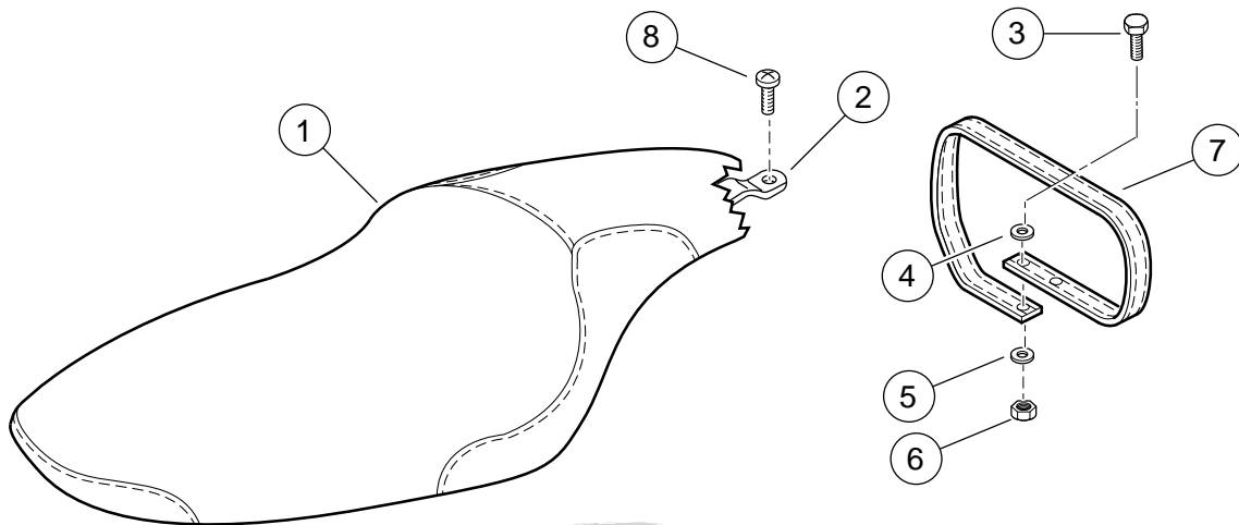
Figure 4. Service Parts: Softtail Seats
