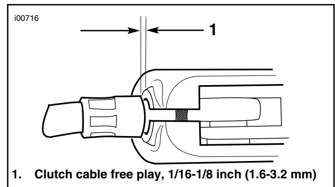
Figure 3. Clutch Cable Adjustment
