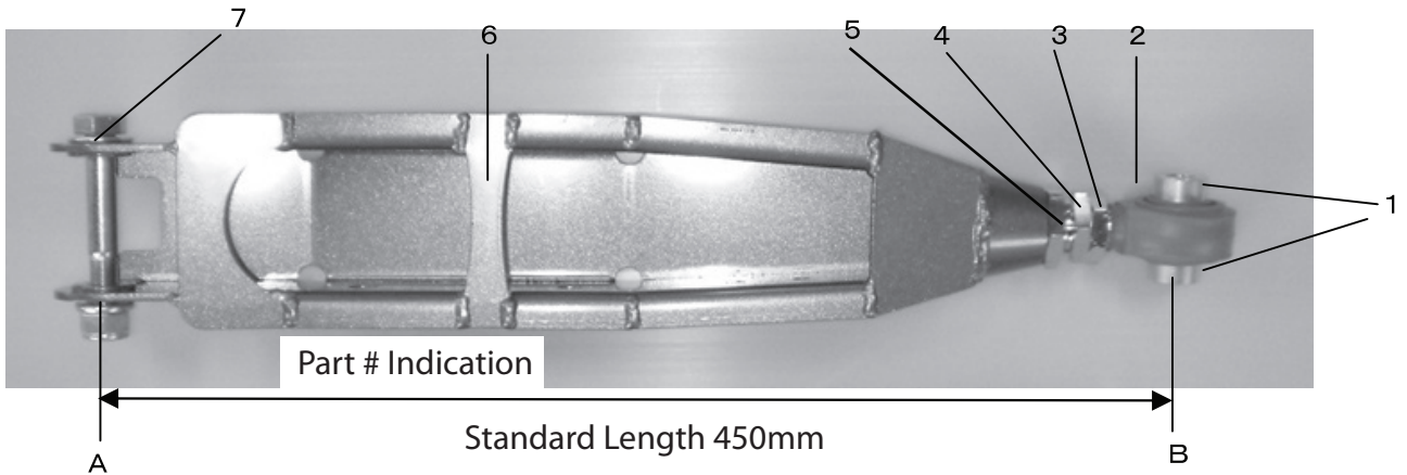
Fig. 1 Assembly
