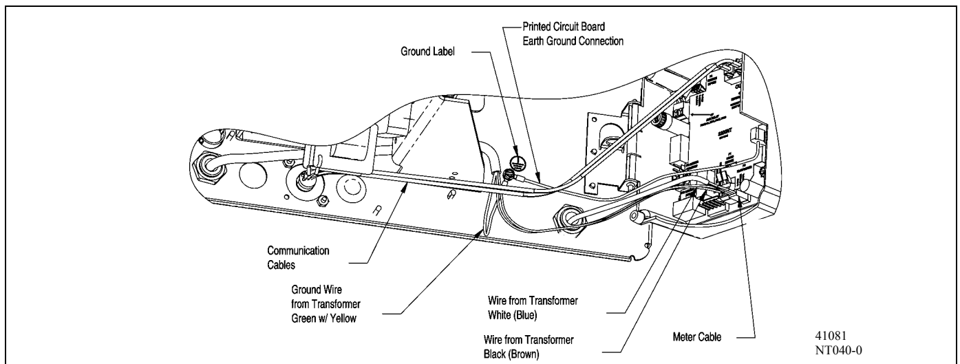
Figure 12: Installing Ground Wire on Transformer, 3150/3900 Valves
