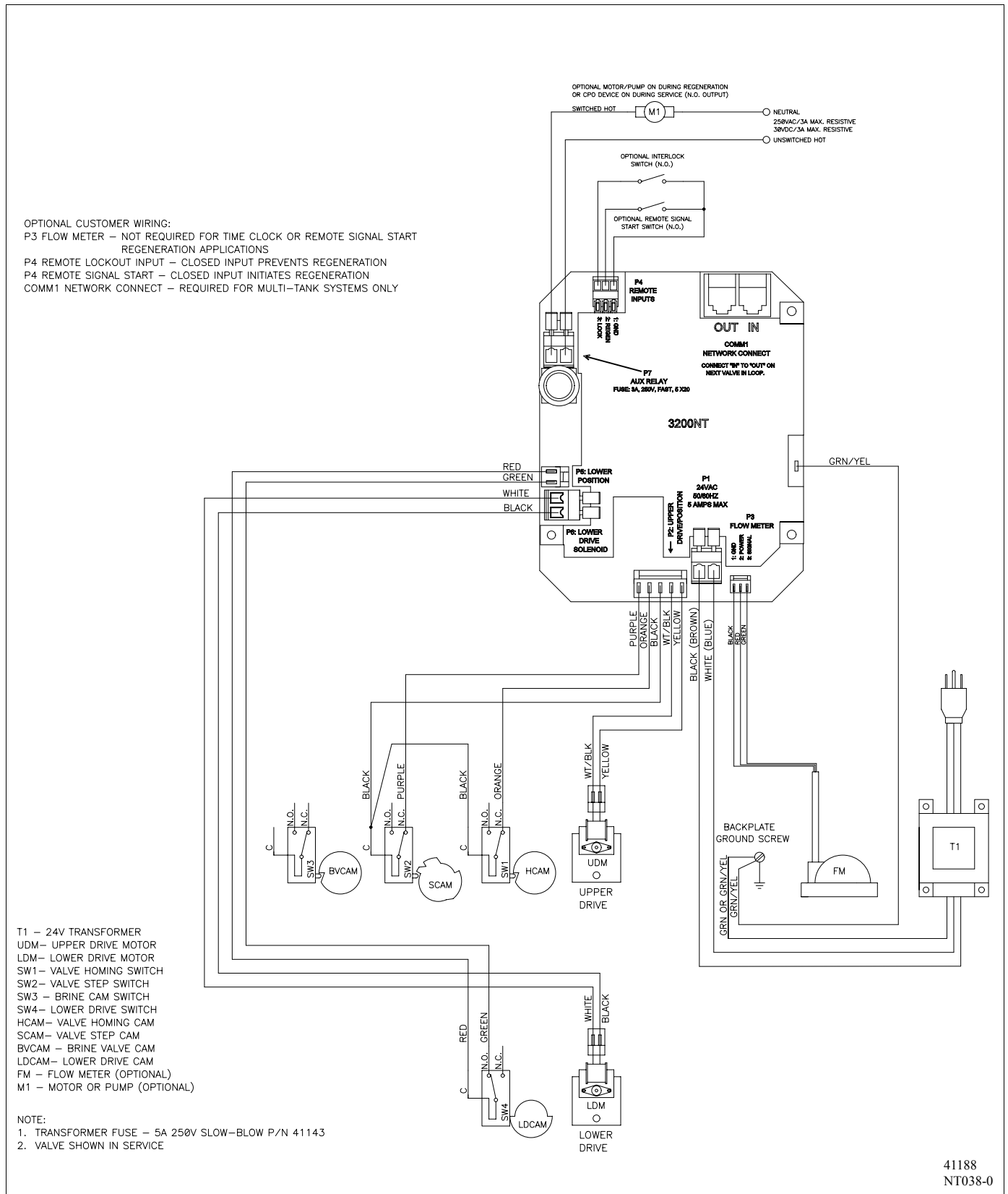
Figure 7: 3900 Timer Wiring Diagram, System #4—Single Valve Regeneration
