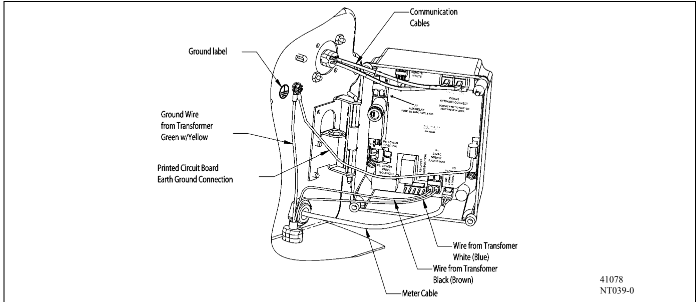
Figure 11: Installing Ground Wire on Transformer, 2750/2850/2900 Valves
