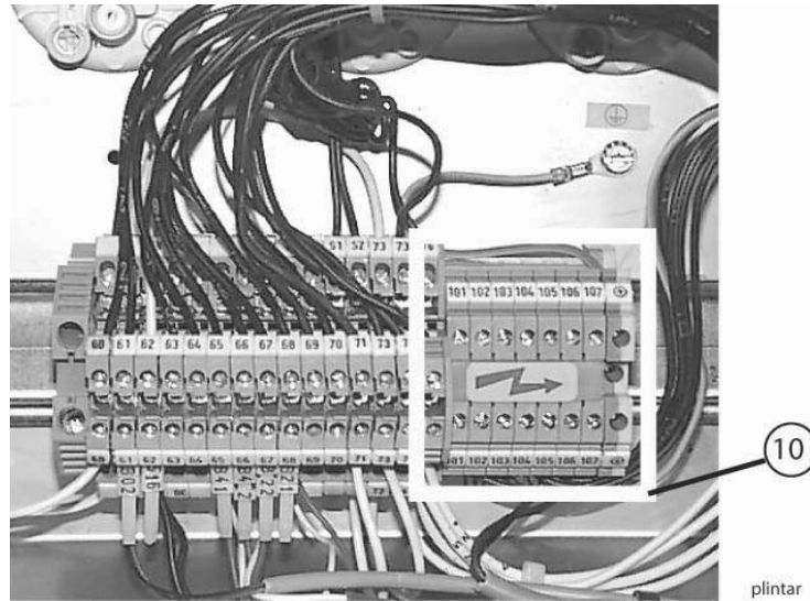
Connections for detergent and drying agent, NOTE: 230V
