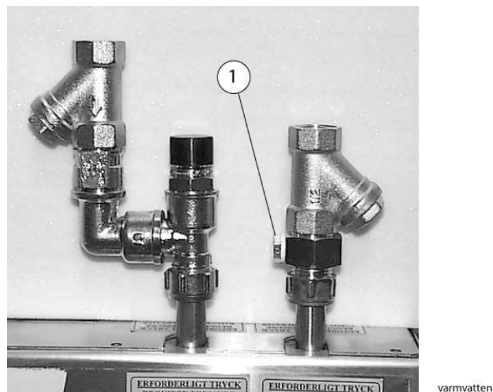
Hot water outlet
