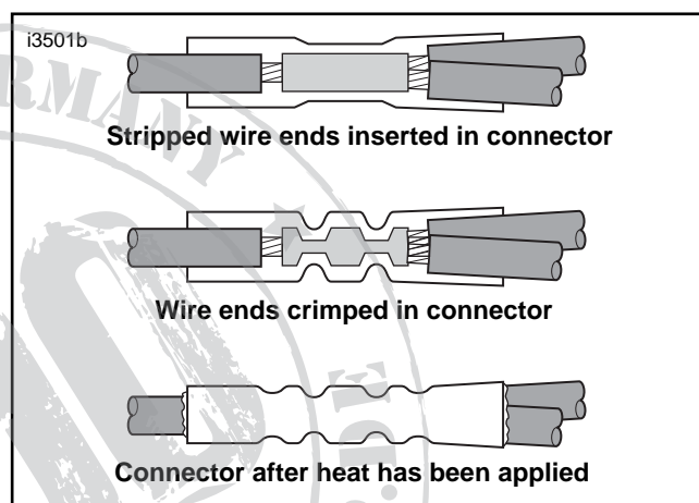
Figure 9. Installing Sealed Butt Splice Connectors
