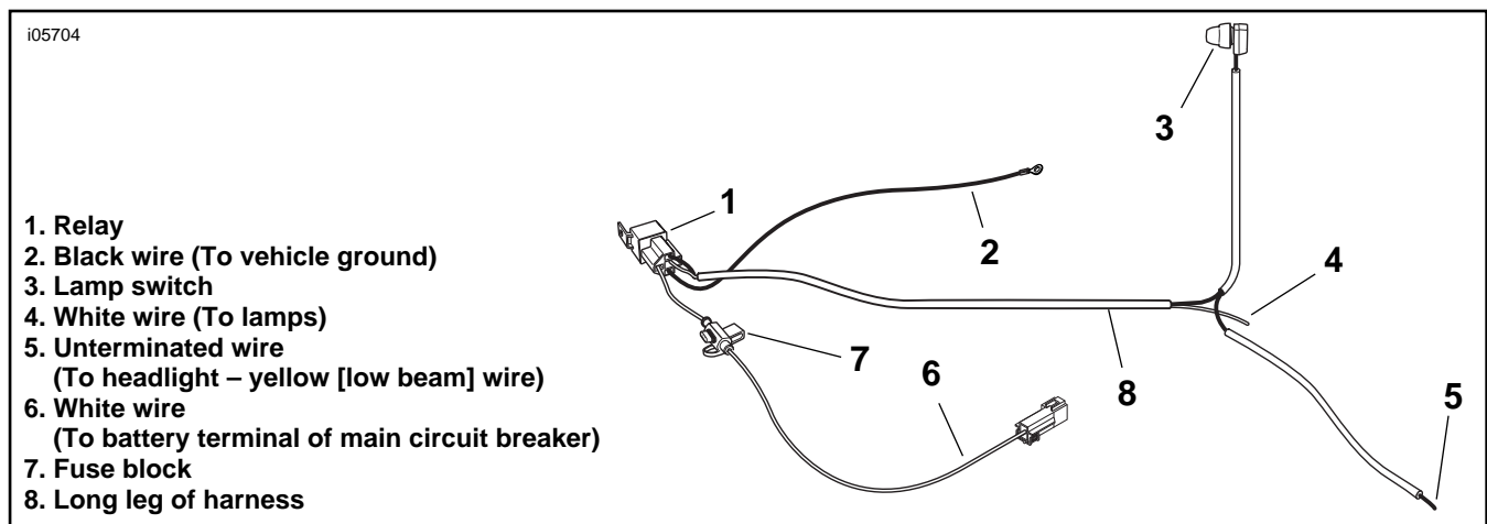
Figure 4. Wiring Harness Component Identification
