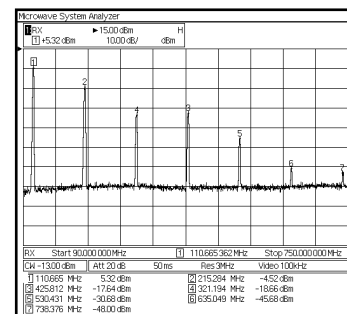
Harmonic measurement with dynamic marker table
