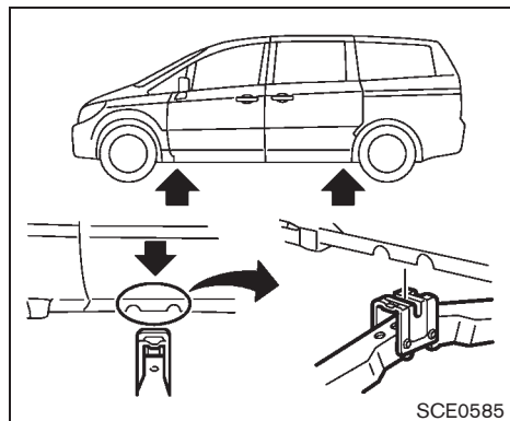
Jack-up point
