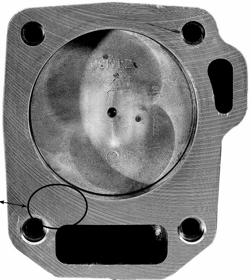
A typical deck face
