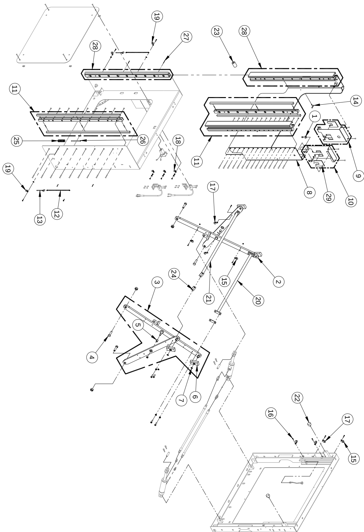
FIGURE 4-9: EXTEND/LIFT MECHANISM ASSEMBLY
