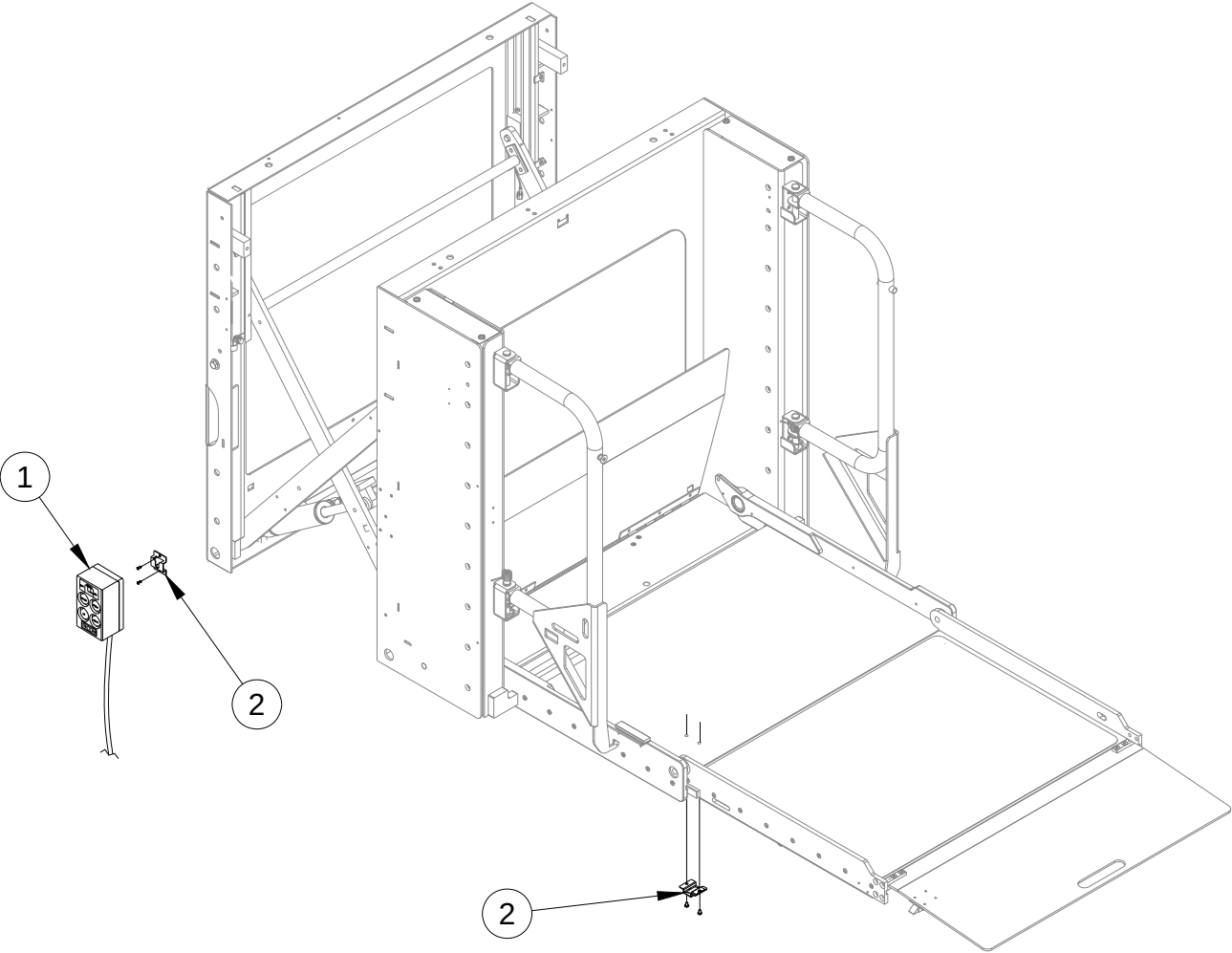
FIGURE 4-6: ELECTRICAL COMPONENTS
