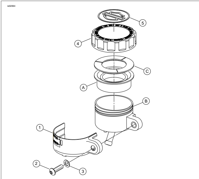
Figure 1. Service Parts: Chrome Rear Brake Reservoir Cover Kit
