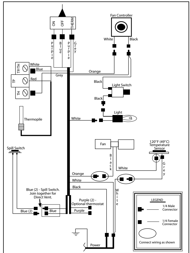
Figure 26: EG40 DV Wiring Diagram.
