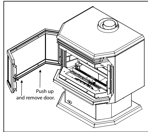
Figure 39: Removing the Door.
