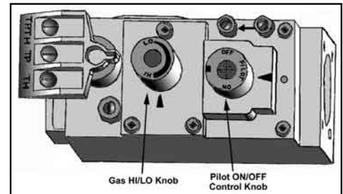
Figure 37: Gas Valve.
