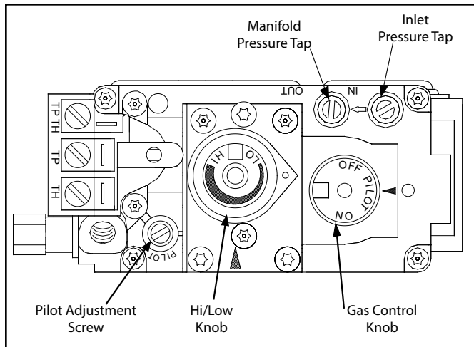
Figure 30: Fully Labeled Gas Valve.
