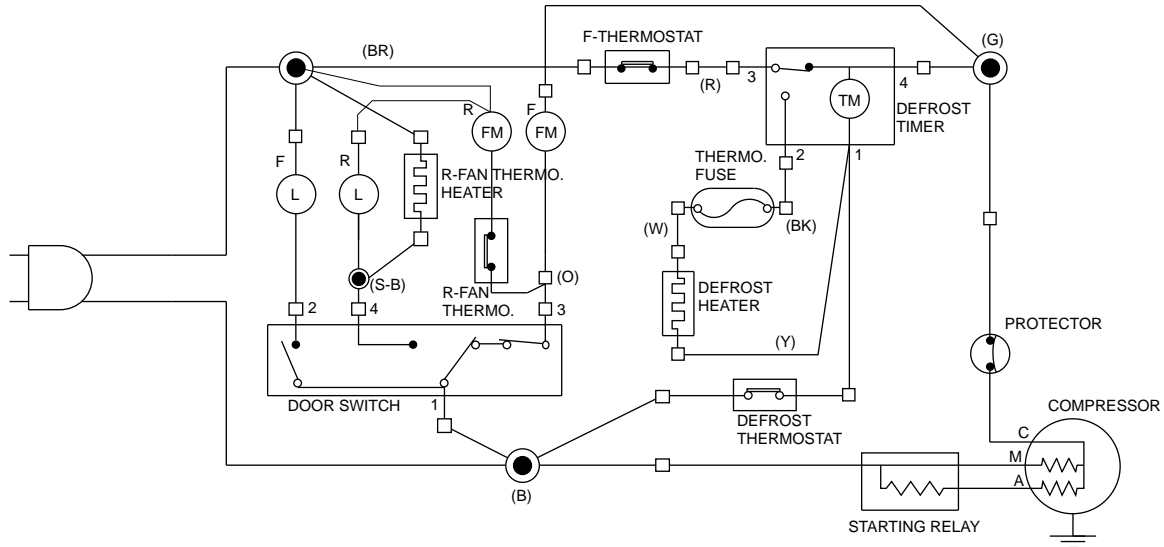
Figure W-1. Wiring Diagram (2 pin plug region)
