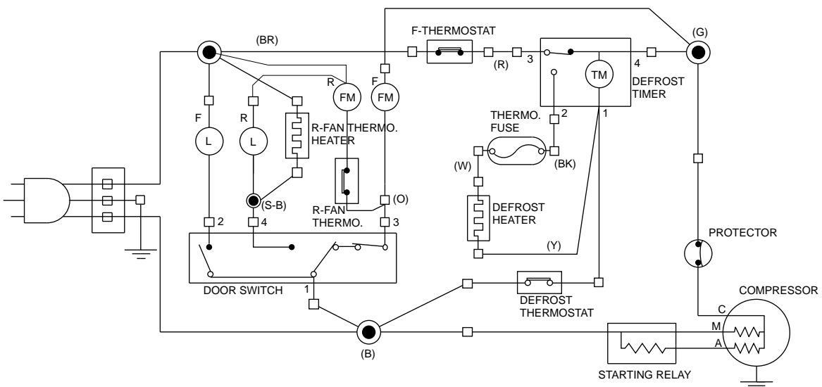
Figure W-2. Wiring Diagram (3 pin plug region)
