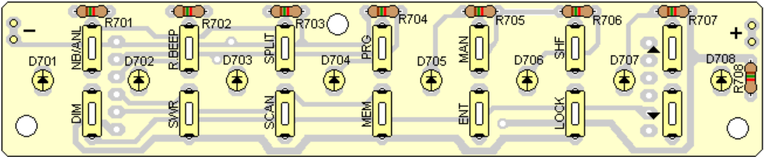
RCI-2950 Pushbutton Swith PCB EPT295031Z
