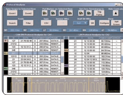
► CAN and LIN Timing and Protocol Decode.
