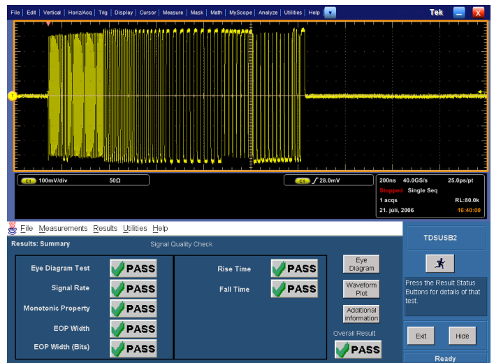
USB compliance testing
