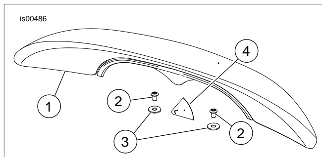
Figure 2. Service Parts for Dash Pad Kit
