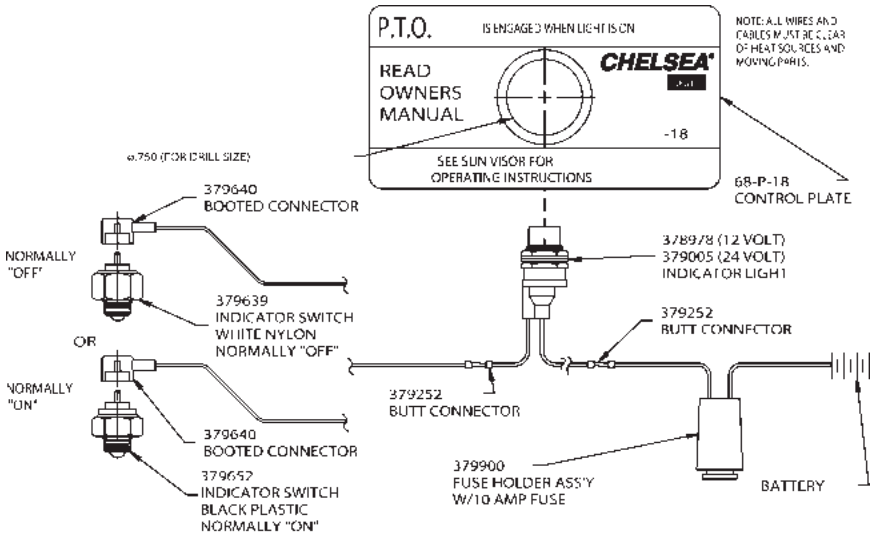
Indicator Light Installation Sketch (SK-286 Rev G)
