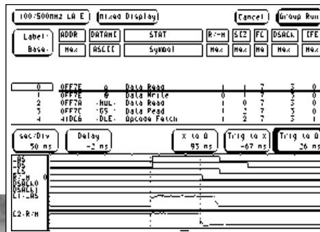
Figure 2. Viewing state, timing, and analog information together, time-correlated on the HP 16500C screen, makes it easy to find the cause of problems.
