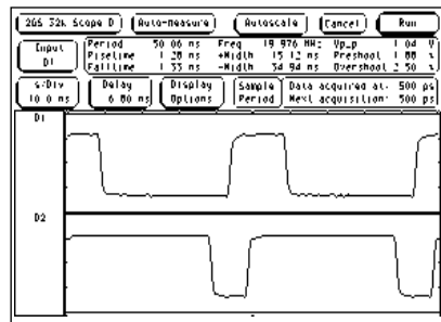
Figure 16. Oscilloscope
