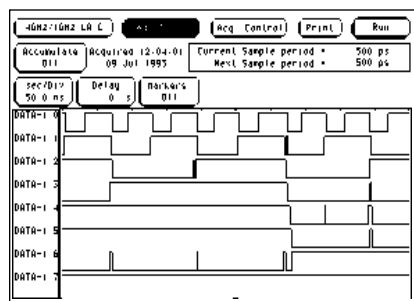
Figure 14. High-Speed Timing
