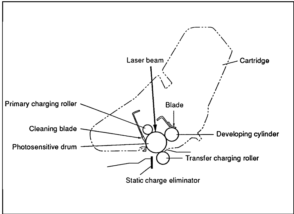
Drum Cleaning
