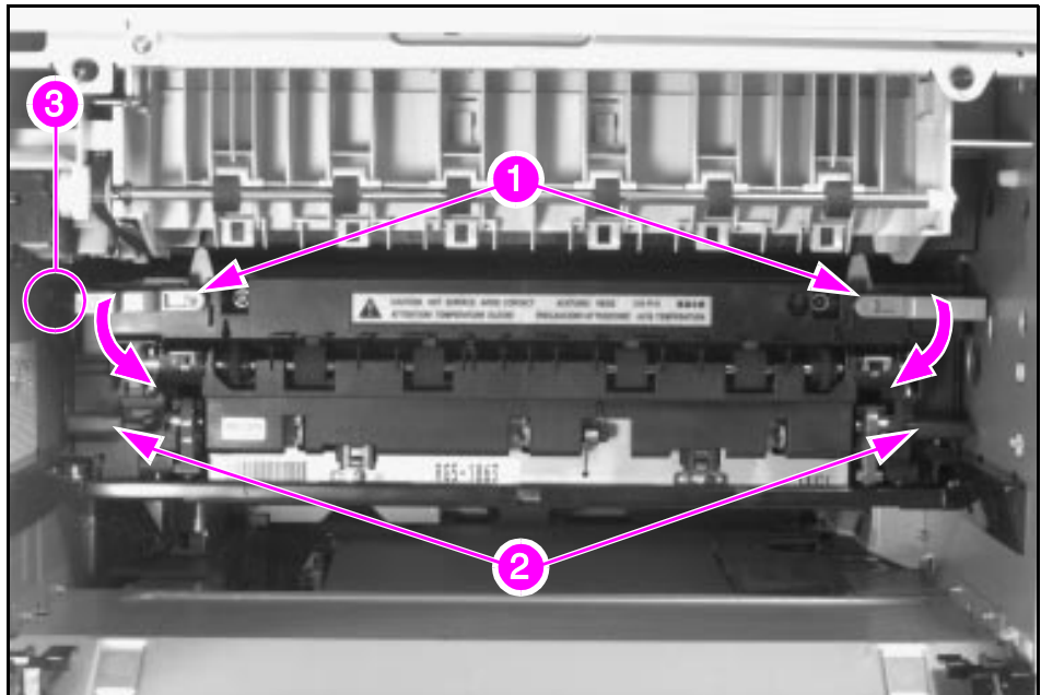
Fusing Assembly
