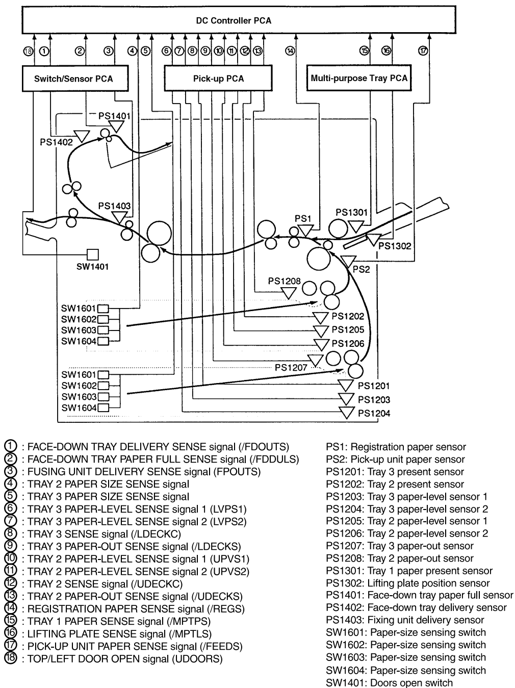
Figure 7-28 Printer Sensors and Switches (Print Engine Only)
