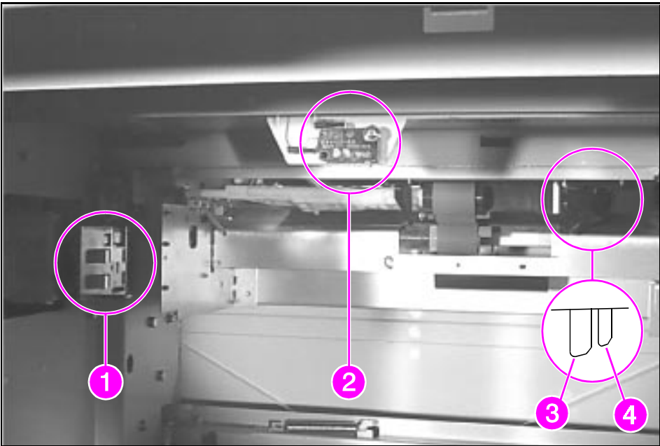
Tray 4 Cavity
