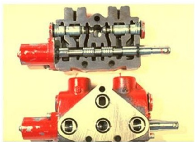
Return Port To Reservoir
