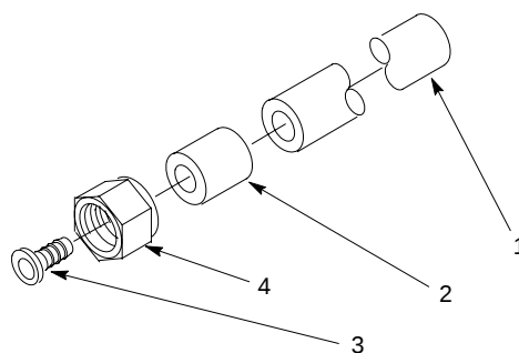
FIGURE 21. TUBE ASSEMBLY
