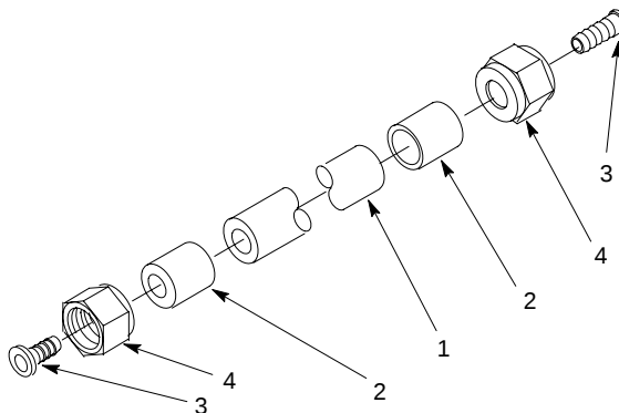
FIGURE 38. TUBING ASSEMBLY
