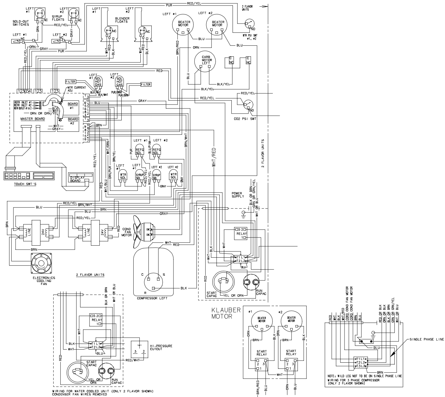
FIGURE 16. WIRING DIAGRAM
