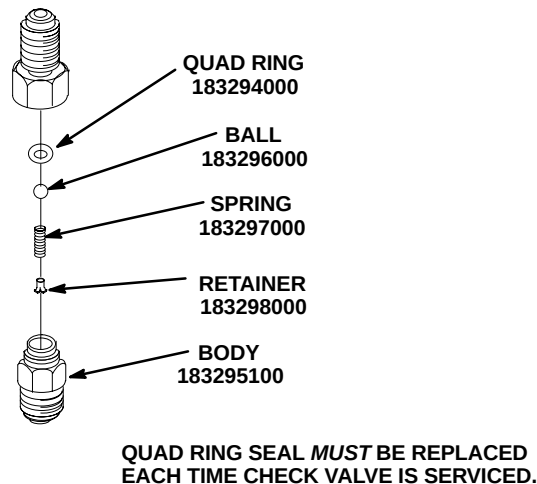
FIGURE 13. CO 2 GAS CHECK VALVE
