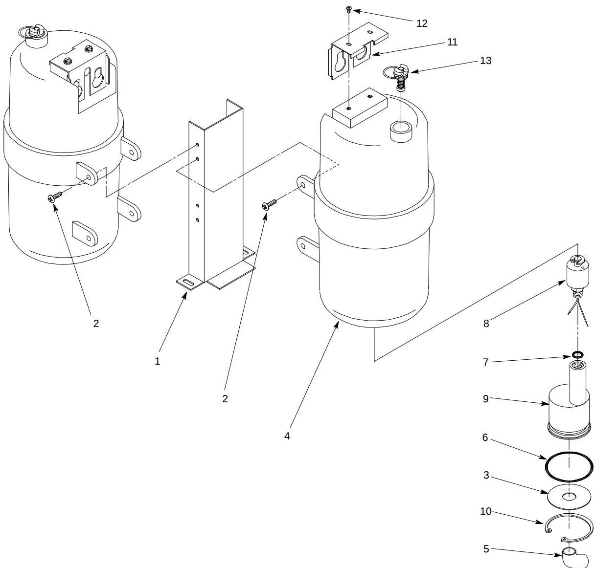
FIGURE 33. BLENDER COMPONENTS
