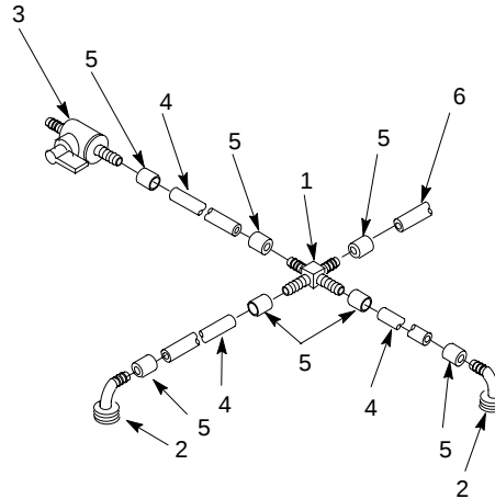
FIGURE 26. TUBING ASSEMBLY (CARB WATER)
