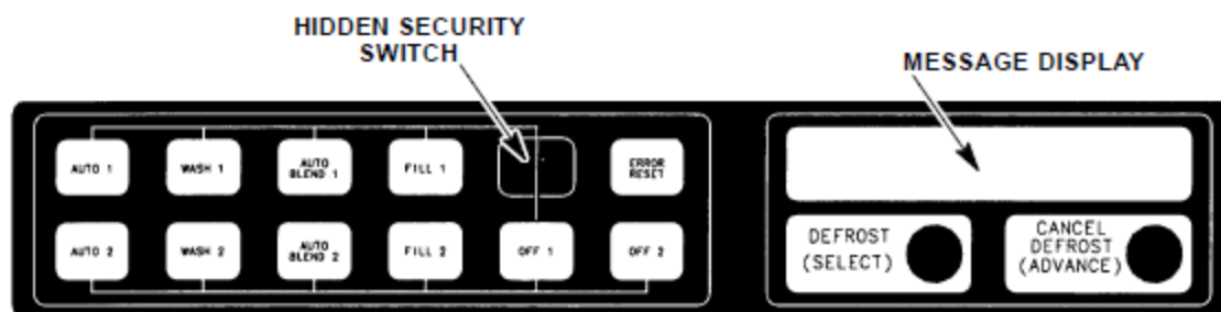
FIGURE 3. CONTROL PANEL ASS'Y
