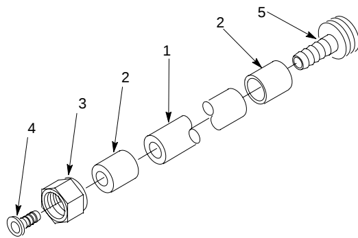
FIGURE 30. TUBING ASSEMBLY (REGULATOR TO BLENDER)
