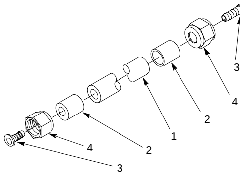
FIGURE 20. SECONDARY CO 2 REGULATOR ASS'Y
