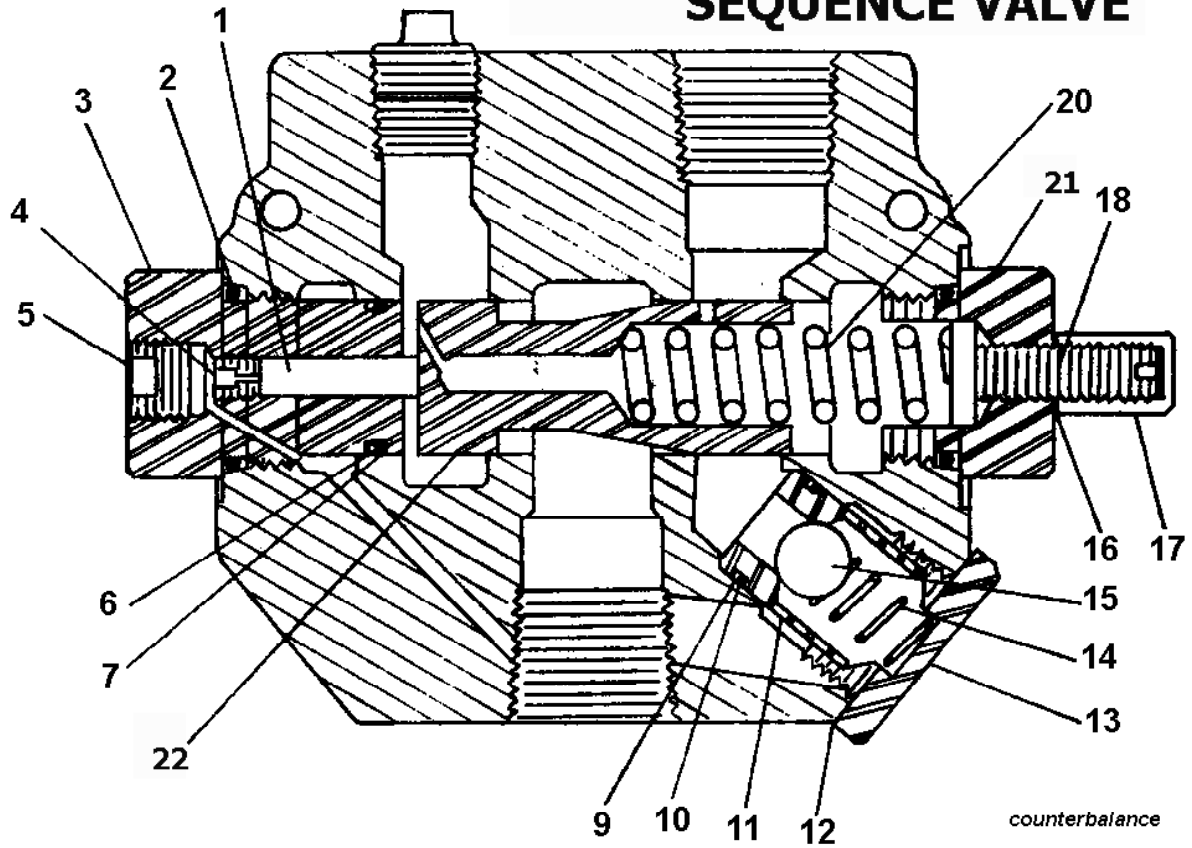
SEQUENCE VALVE PART #A101H47
