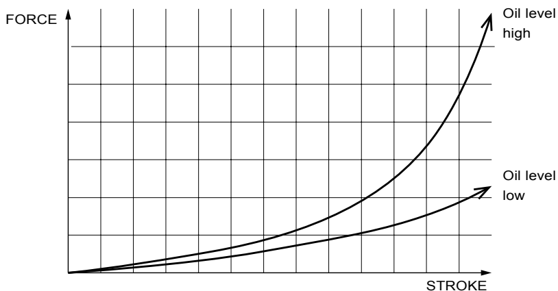
Oil Level Diagram
