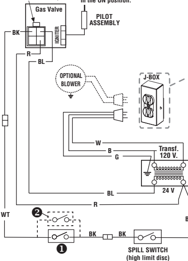
Figure 21 Electronic Wiring Diagram (Honeywell) Showing Blower Wiring for Optional FBK-100 & FBK-200 Kits
