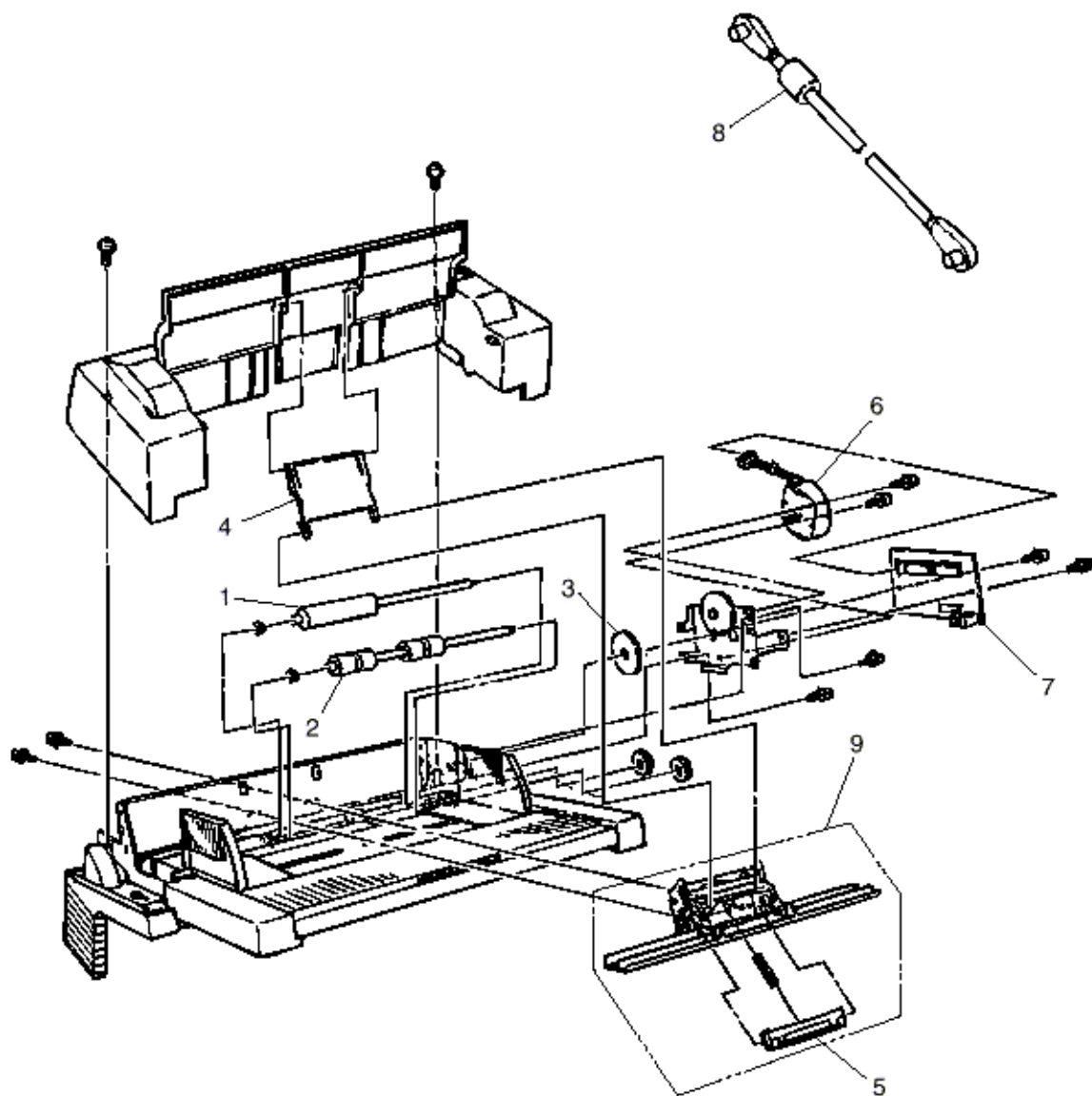
Figure 6-1 Multi-Purpose Feeder
