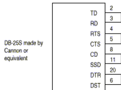
Test Connector Connection Diagram
