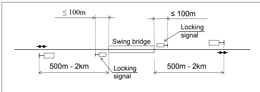
Figure 6.5:11 Main and locking signals of a swing bridge.
