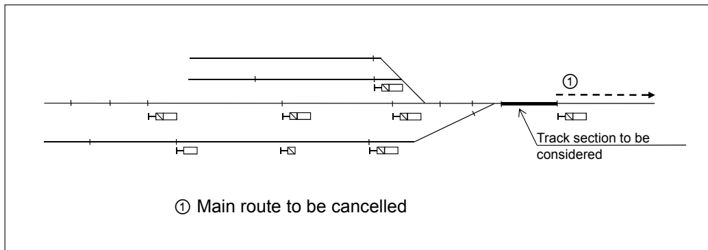
Figure 6.3:20 Track sections to be proved vacant as a condition for cancelling a set main route, if there is no set main route to the route entry signal of main route to be cancelled.
