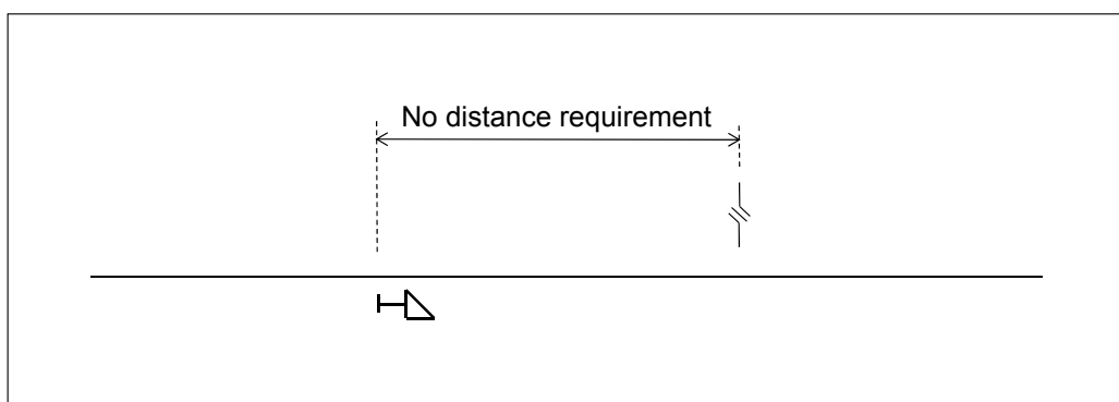
Figure 6.4:47 Positioning a shunting signal in rear of the neutral section, when the shunting signal cannot act as the main route entry or exit signal or shunting route entry signal.
