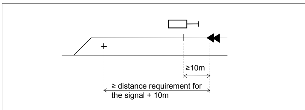
Figure 6.4:25 The effect of signal balises on main signal positioning.
