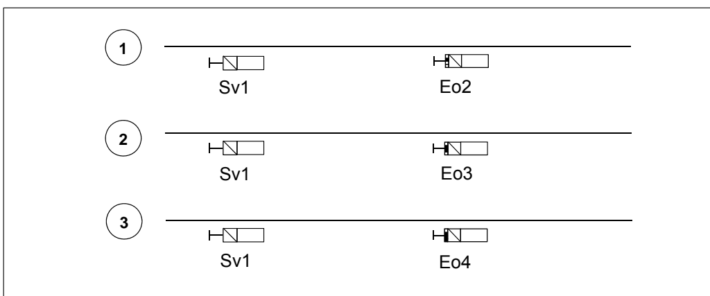
Figure 6.2:9 Examples of activation of control line 'Sv1'. The types of the signals may vary.
