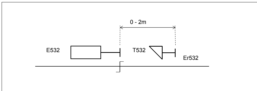
Figure 6.4:44 Shunting signal at the same place as the main signal in respect to track sections.
