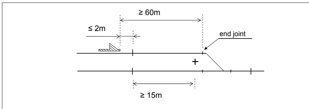
Figure 6.4:67 Positioning of a stopping device equipped with a hand lever in respect to a point and the border of the point track section
