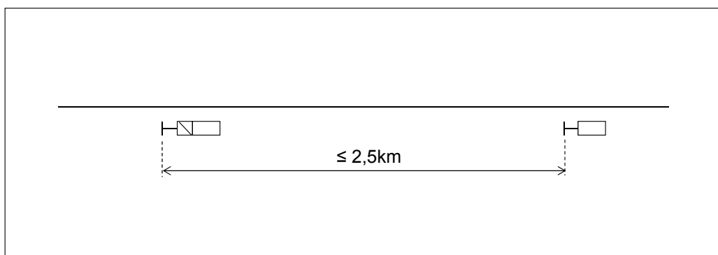
Figure 6.4:31 Presignalling distance
