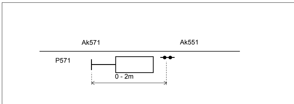
Figure 6.4:14 Positioning a main signal in respect to the axle counter.
