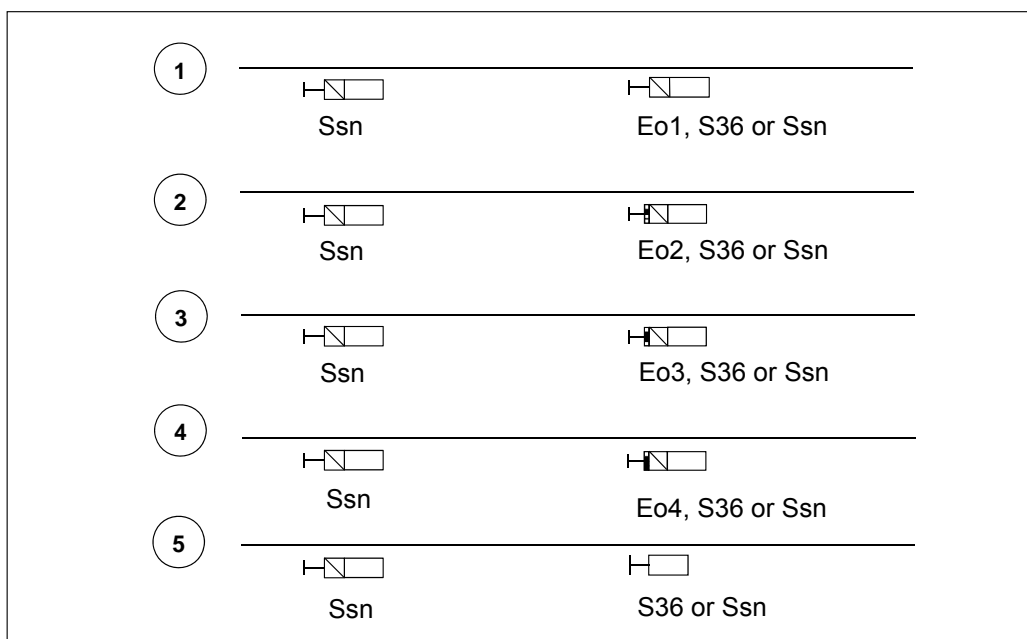
Figure 6.2:12 Examples of transmitting the fictive aspect 'Ssn' to ATP. The types of the signals may vary.
