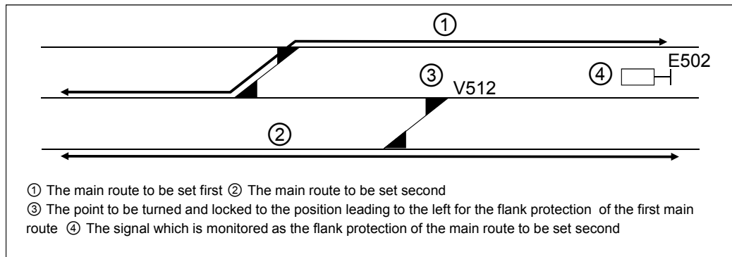
Figure 6.3:7 Monitoring of the flank protection, when the point providing the flank protection cannot be turned to the position required by the main route flank protection.
