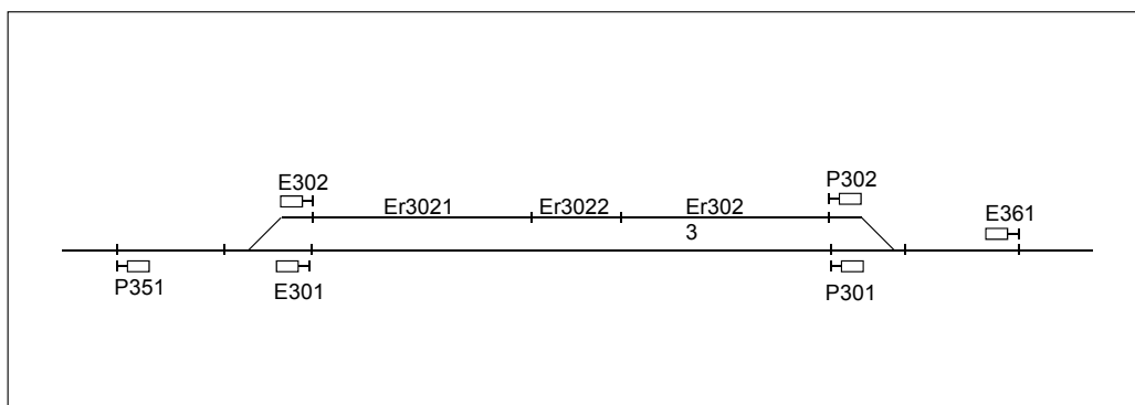
Figure 6.3:6 State of track sections on the main route to an occupied track.
