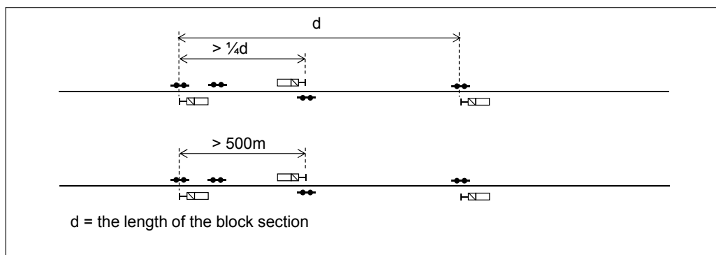
Figure 6.3:18 The situations, where a track section in advance of the signal, acting as an overlap, has to be built.
