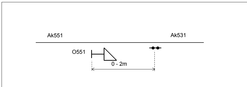
Figure 6.4:42 Positioning a shunting signal in respect to an axle counter.
