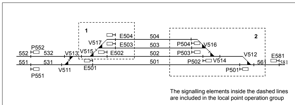
Figure 6.3:26 Protecting local point operation by a point and signal.
