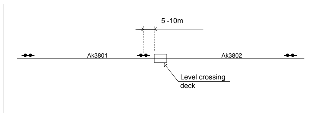
Figure 6.5:9 Level crossing light system without a road section.
