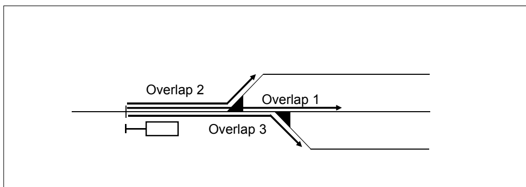
Figure 6.3:17 An example of the determining of the primary overlap and the secondary overlaps.
