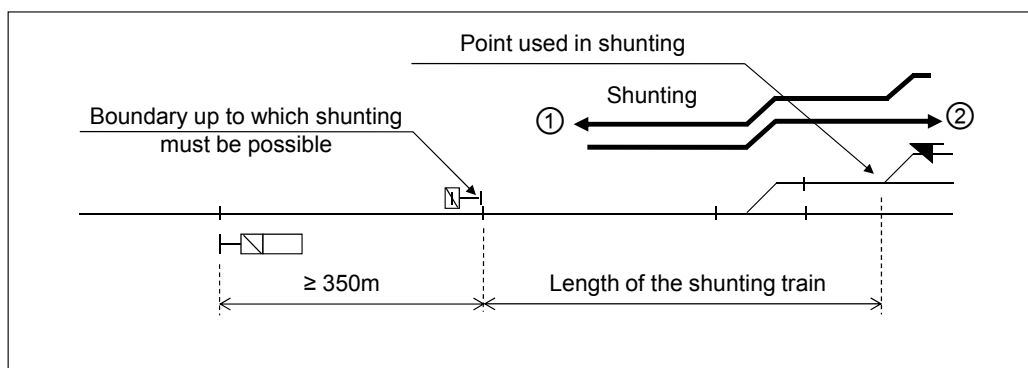
Figure 6.4:21 The effect of the shunting train length on positioning of a station entry signal.
