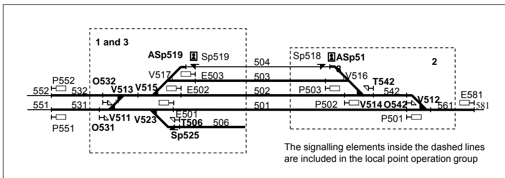
Figure 6.3:32 Local point operation group. The codes of the signalling elements included in the local point operation group, track sections associated with the local point operation group and the codes of the shunting signals displaying an 'No aspects' aspect are in boldface.
