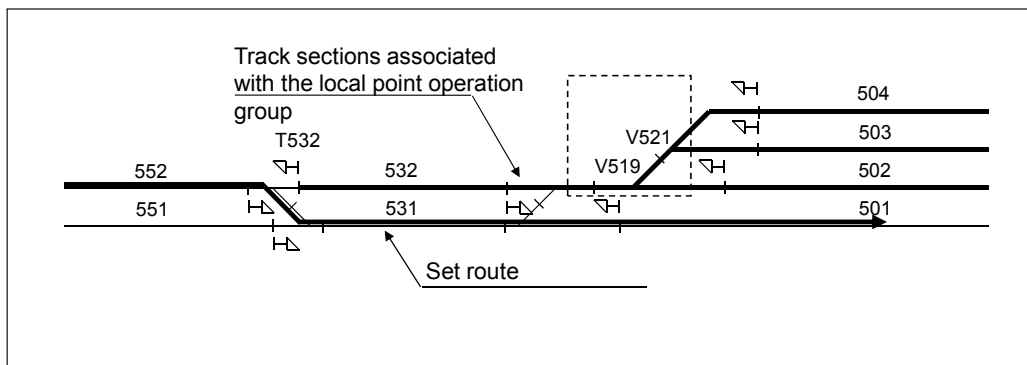
Figure 6.4:51 Shunting signals, which enable simultaneous shunting route and local point operation permission.
