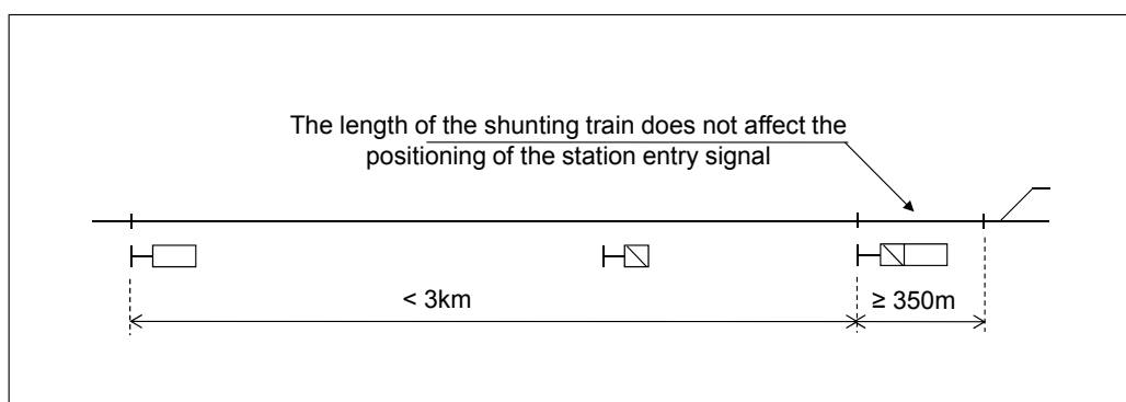
Figure 6.4:22 The effect of the line signal prior to the station entry signal on positioning the main signal.
