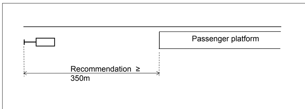
Figure 6.4.27 Positioning a main signal in such a way that the passenger platform is in advance of the main signal.
