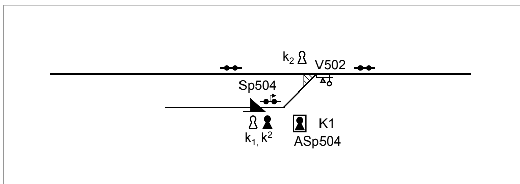
Figure 6.4:76 Concatenating the key lock operation keys.
