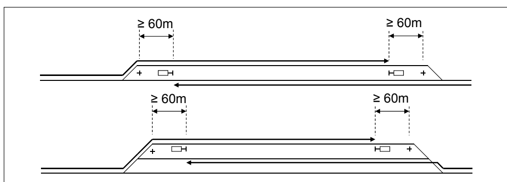
Figure 6.4:18 Setting simultaneous routes with overlap 0, when the danger point distance of the route exit signals are at least 60m.
