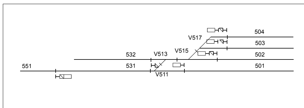
Figure 6.4:38 Equipping tracks with shunting signals.
