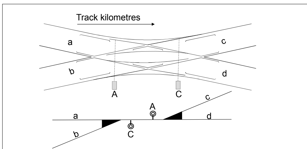
Figure 6.2:15 The point machines of a double diamond crossing with slips and the management of the point as two simple points in the signalling system logic.
