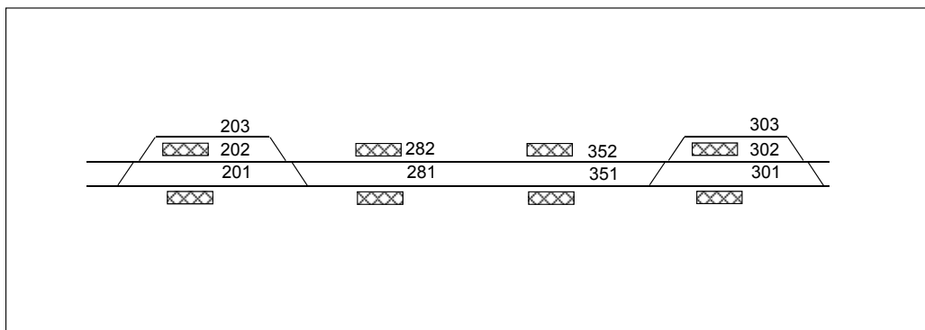
Figure 6.4:11 The numbering of through tracks of consecutive railway operating locations.
