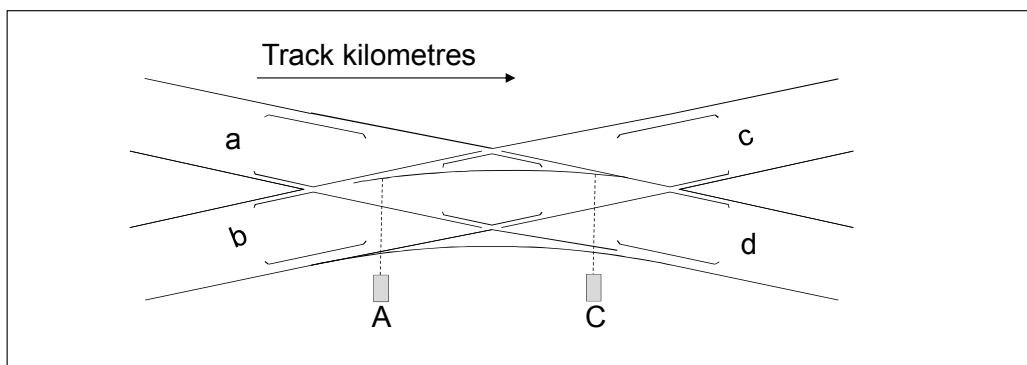
Figure 6.2:16 The point machines and route paths of a single diamond crossing with slips.
