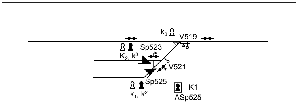
Figure 6.4:77 Concatenating the key lock operation keys, when two derailleurs protect the route track.
