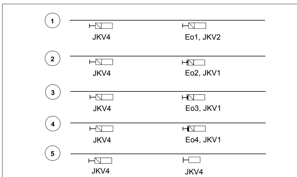
Figure 6.2:5 Examples of activation of control line 'JKV4'. The types of the signals may vary.
