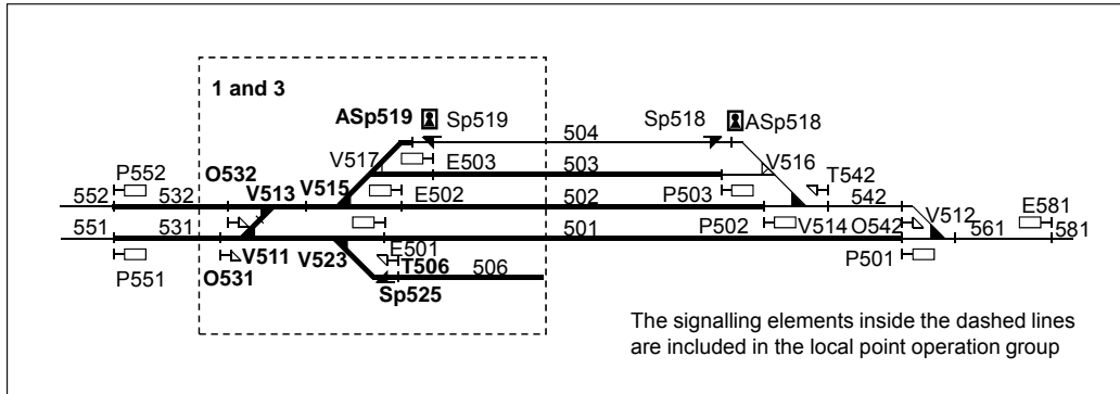
Figure 6.3:31 A local point operation group. The codes of the signalling elements included in local point operation group, track sections associated with local point operation group and the codes of the shunting signals displaying an 'No aspects' aspect are in boldface.
