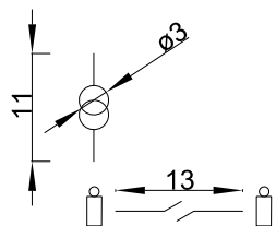
Draining transformer on the mast in an insulated overlap (also the insulated overlap and catenary supports must be presented with this symbol)
