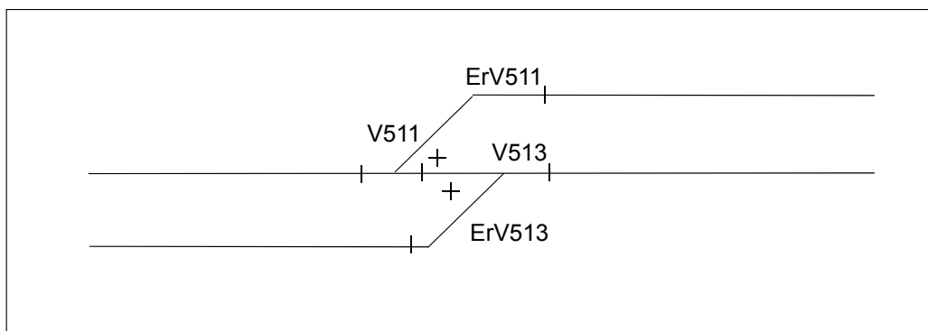
Figure 6.3:3 Track vacancy proving of a point, which is not free of fouling restrictions.
