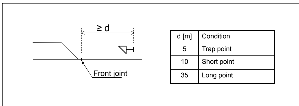
Figure 6.4:46 Positioning a shunting signal in respect to the front joint of a route point.
