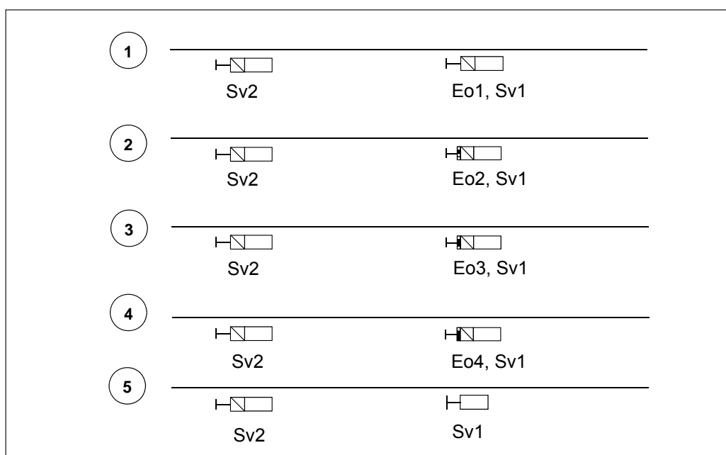
Figure 6.2:10 Examples of activation of control line 'Sv2'. The types of the signals may vary.
