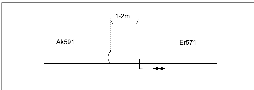
Figure 6.6:2 Short cut of the rails on the axle counting section, when the track vacancy proving realized with track circuits ends
