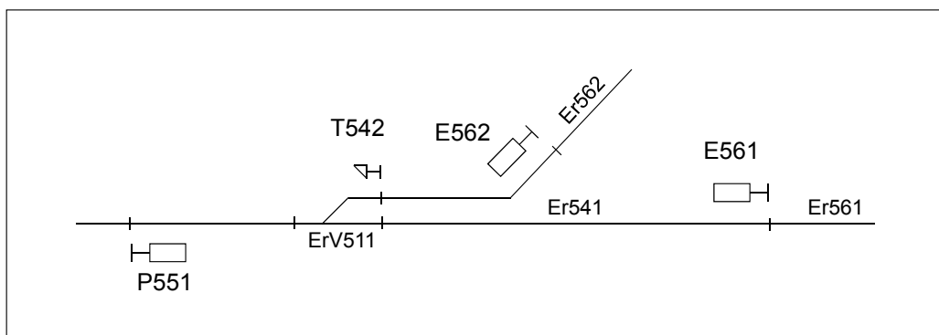
Figure 6.4:49 The effect of flank protection requirements on shunting signal positioning.
