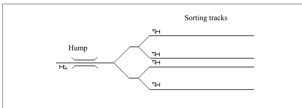
Figure 6.5:1 The shunting signals protecting the points between the hump and the sorting tracks.
