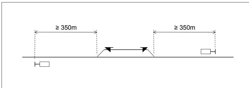
Figure 6.4:33 Positioning a line point protecting main signal in respect to the line point.
