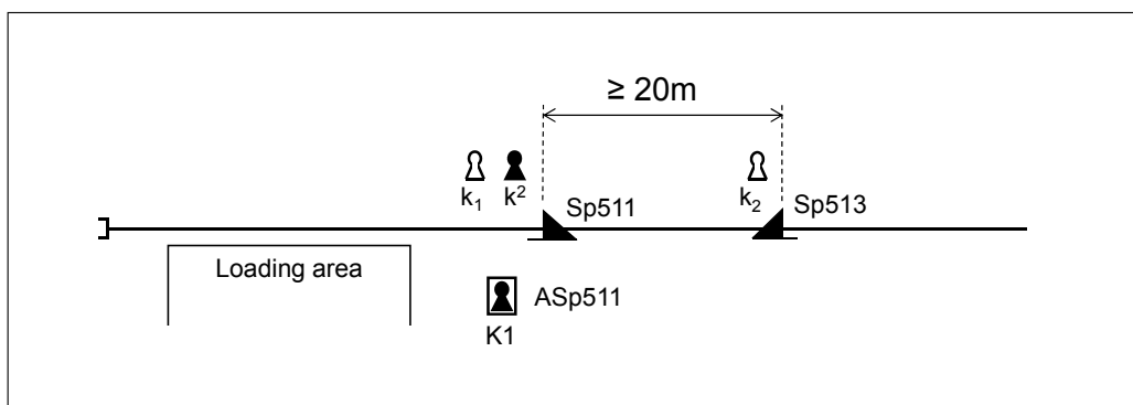
Figure 6.4:78 Protecting the loading area with derailleurs.
