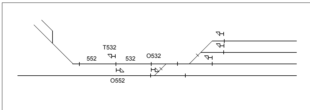
Figure 6.4:41 Positioning a shunting signal on a track leading away from the track layout, that is connected to the interlocking system.
