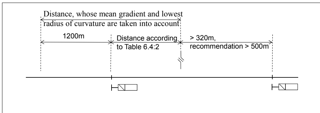
Figure 6.4:23 The effect of the neutral section on the main signal positioning.
