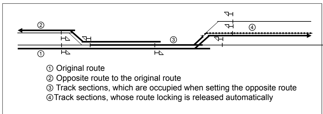
Figure 6.3:22 Automatic release of an unused shunting route.
