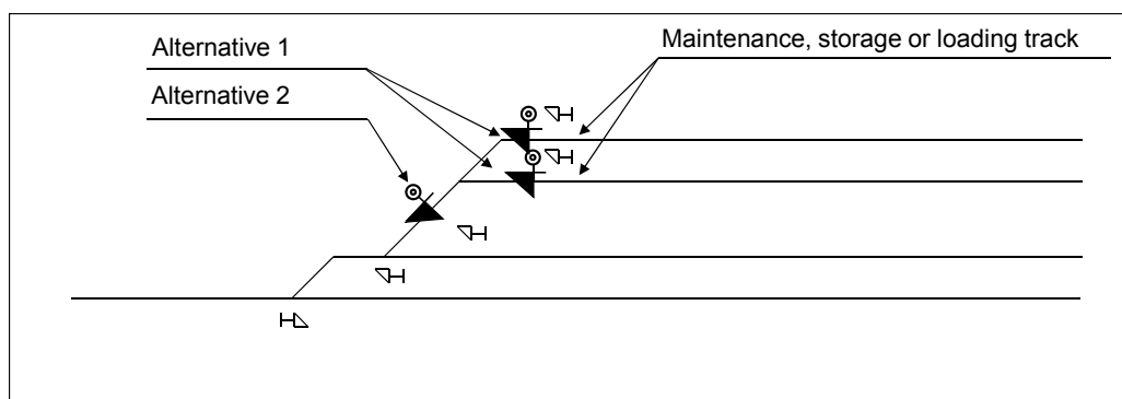
Figure 6.4:62 Equipping maintenance, storage or loading tracks with a derailer.
