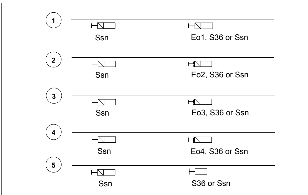
Figure 6.2:8 Examples of activation of control line 'Ssn'. The types of the signals may vary.
