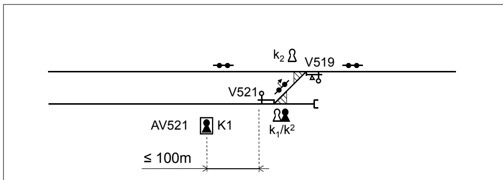
Figure 6.4:74 The distance from the key box to the object, whose key lock operation key is monitored by the key box.
