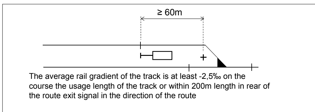
Figure 6.3:10 Only the primary overlap on the route.
