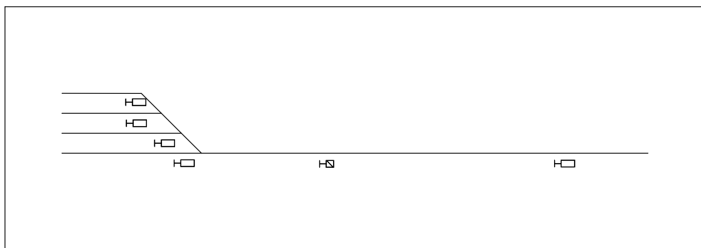
Figure 6.4:35 Positioning only one distant signal instead of four distant signals positioned together with main signals.
