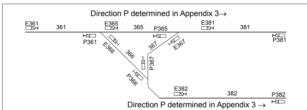
Figure 6.4:13 The letter of the signal code on a Y-track.
