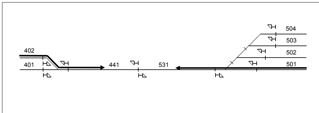
Figure 6.4:39 The shunting signals enabling simultaneous shunting routes.
