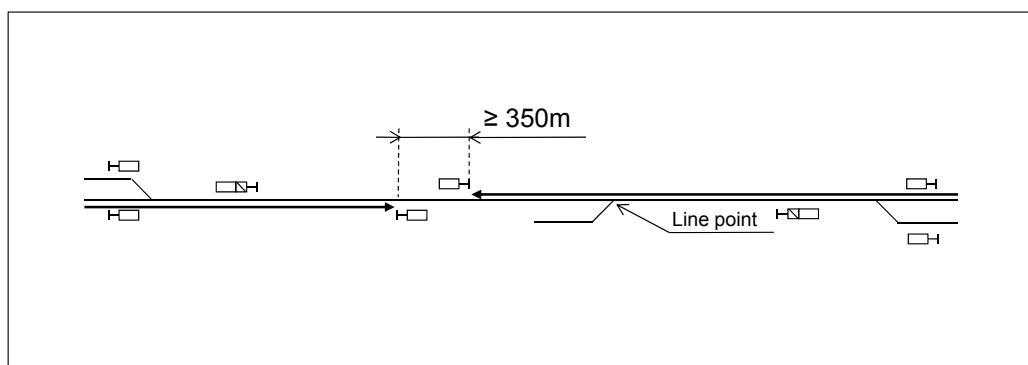
Figure 6.3:23 The main signals of the line simultaneously functioning as the route exit signals of opposing routes.
