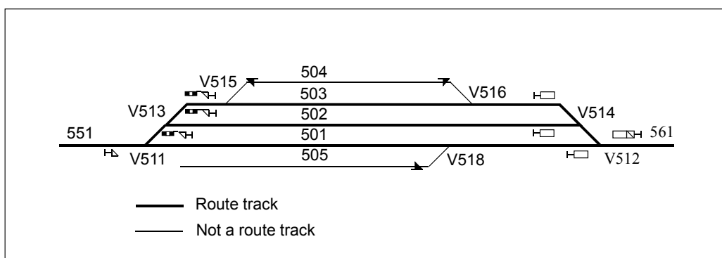
Figure 6.4:12 Protecting points with main signals.
