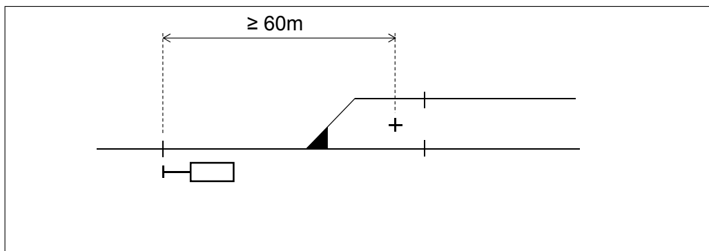
Figure 6.3:15 The route has the overlap 0, primary overlap and secondary overlap.
