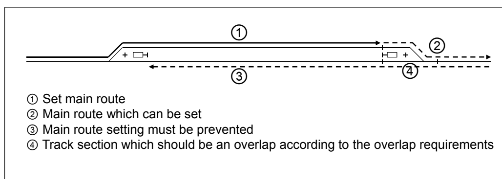
Figure 6.2:19 Preventing simultaneous setting of routes.
