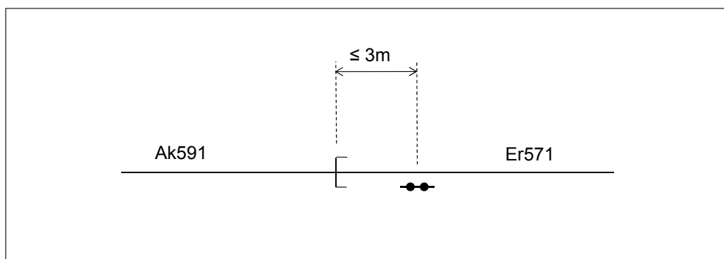
Figure 6.4:69 The location of track section boundaries at the interface of axle counter and track circuit systems.
