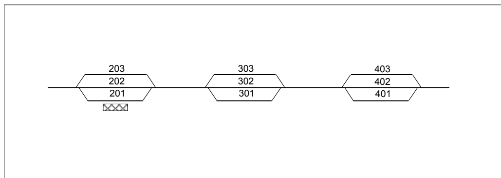
Figure 6.4:9 The numbering of track layout on consecutive railway operating locations.
