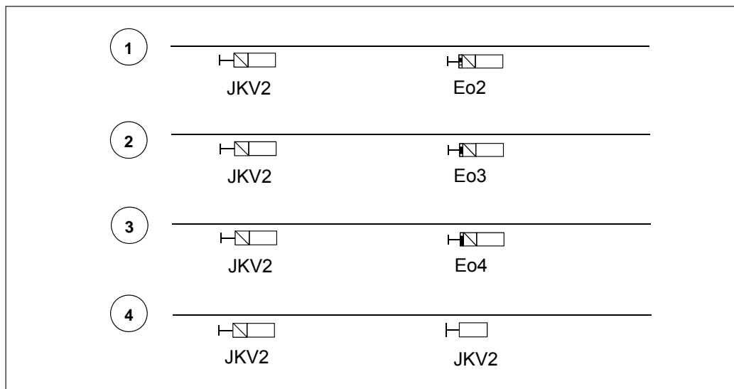
Figure 6.2:3 Examples of activation of control line 'JKV2'. The types of the signals may vary.
