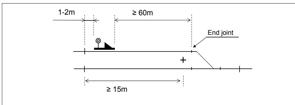
Figure 6.4:66 Positioning a powered stopping device in respect to a point and the border of the point track section
