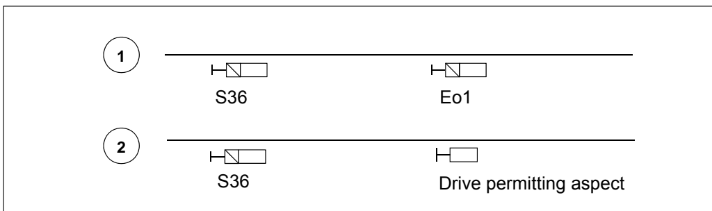
Figure 6.2:7 Examples of activation of control line 'S36'. The types of the signals may vary.
