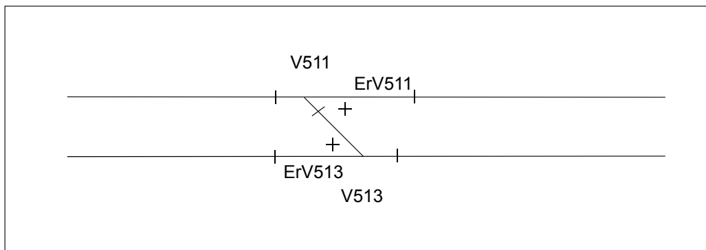
Figure 6.3:2 Track vacancy proving of points, one of which is not free of fouling restrictions. In Figure the point V511 is not free of fouling restrictions and the point V513 is free of fouling restrictions.
