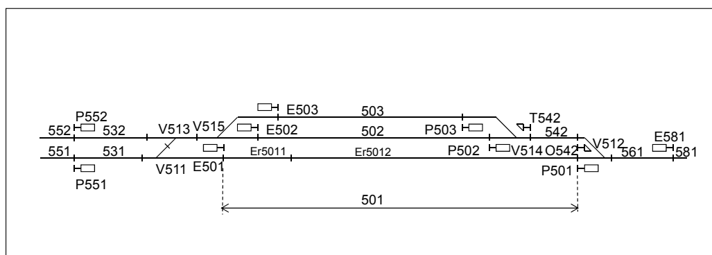
Figure 6.4.7 The numbering of tracks and points and signalling apparatus codes.
