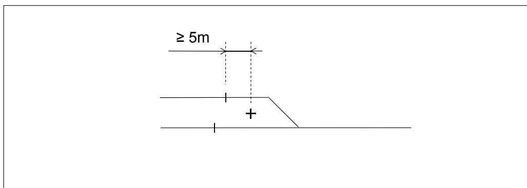
Figure 6.3:1 The location of the track section boundary in a point branch free of fouling restrictions.
