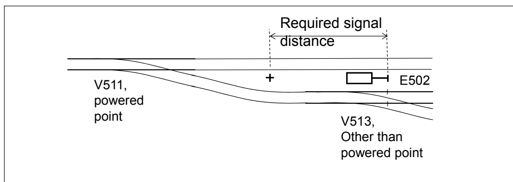
Figure 6.4:71 The effect of a point, other than a powered point, on positioning a track section boundary.
