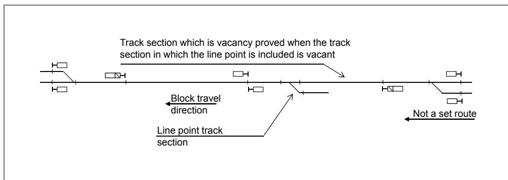
Figure 6.3:24 The conditions for the key box permission of the line point when the line point is located on the first block section with respect to the block travel direction.
