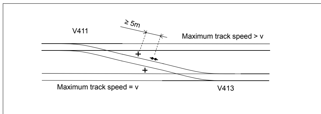
Figure 6.4:58 The effect of the maximum track speed on positioning a track section boundary.
