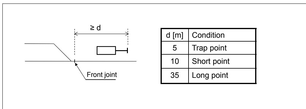
Figure 6.4:20 Positioning a main signal in respect to the axle counter.
