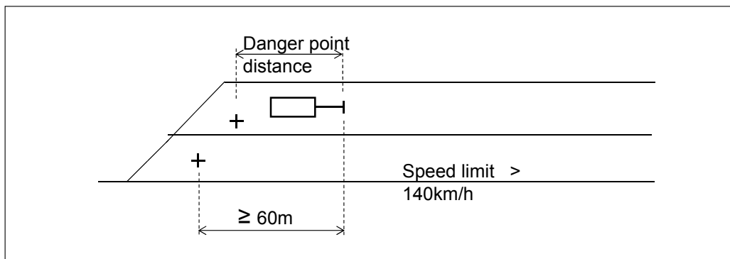
Figure 6.4:19 Main signal location dependence on the maximum track speed.
