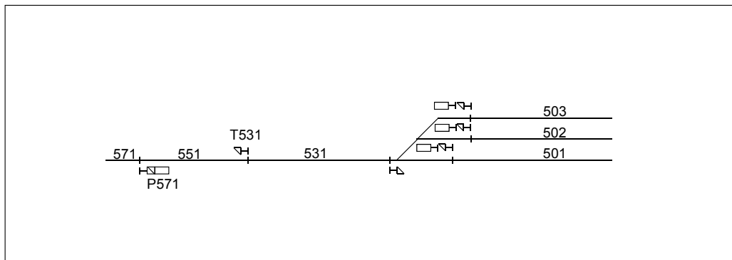
Figure 6.4:48 Using a shunting signal for protecting the track section that is functioning as overlap.
