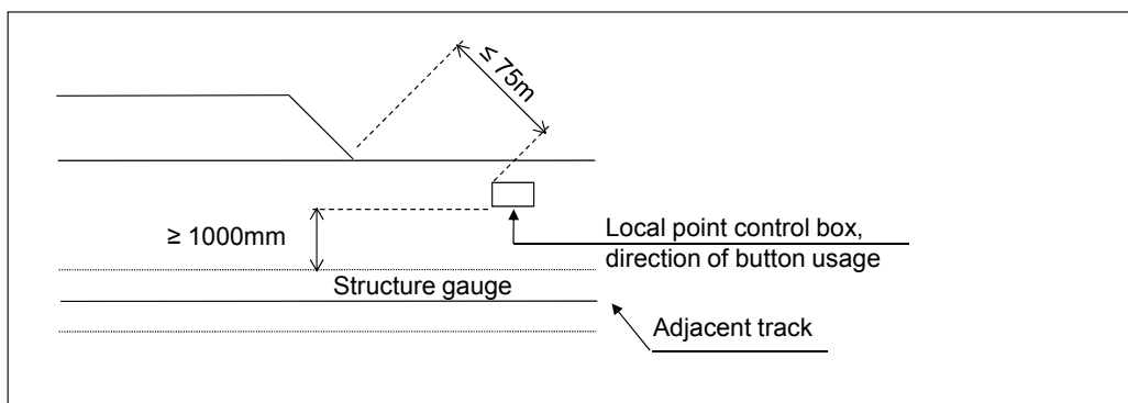
Figure 6.4:60 The location of the local point control box.
