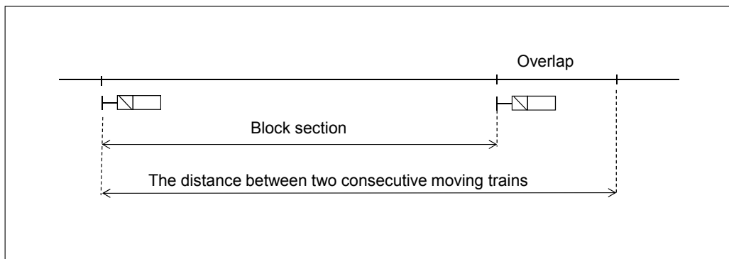
Figure 6.4:30 The effect of overlap on the distance of two consecutive moving trains.
