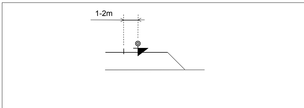
Figure 6.4:65 Positioning a derailer equipped with a point machine in respect to the track section of the point to be protected.
