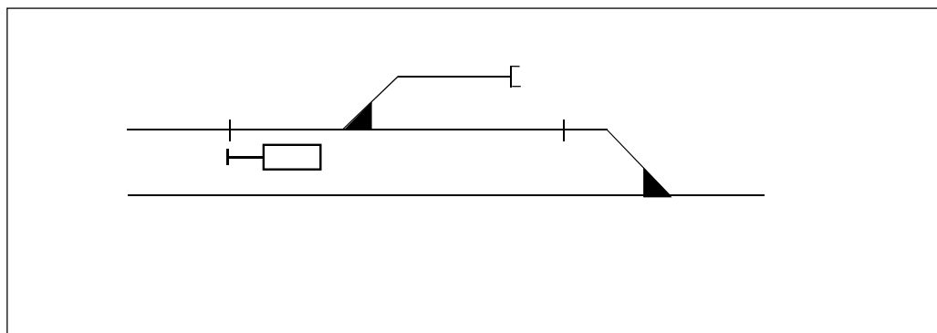
Figure 6.3:8 Only the overlap 0 on the route.
