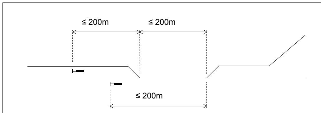
Figure 6.4:54 Positioning a radio signal in respect to points.
