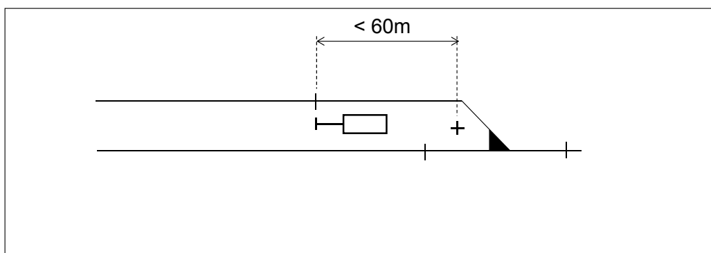
Figure 6.3:12 Only the primary overlap on the route.
