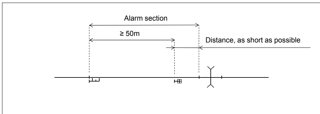
Figure 6.4:52 Positioning a level crossing signal.
