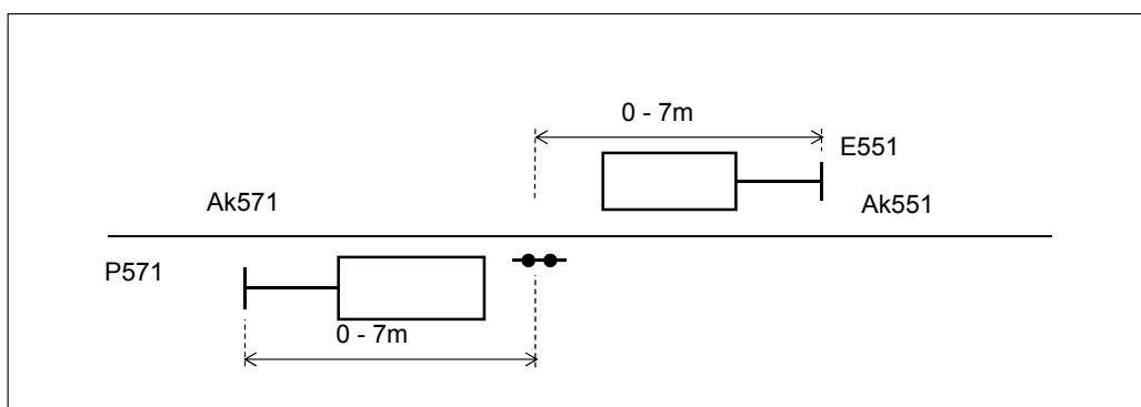
Figure 6.4:16 Positioning a main signal in respect to the track section boundary.
