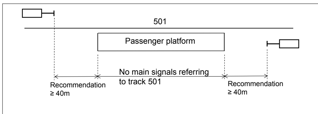
Figure 6.4.26 Positioning a main signal in such a way that the passenger platform is in rear of the main signal.
