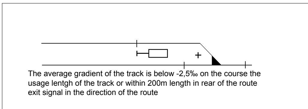
Figure 6.3:11 Only the primary overlap on the route.
