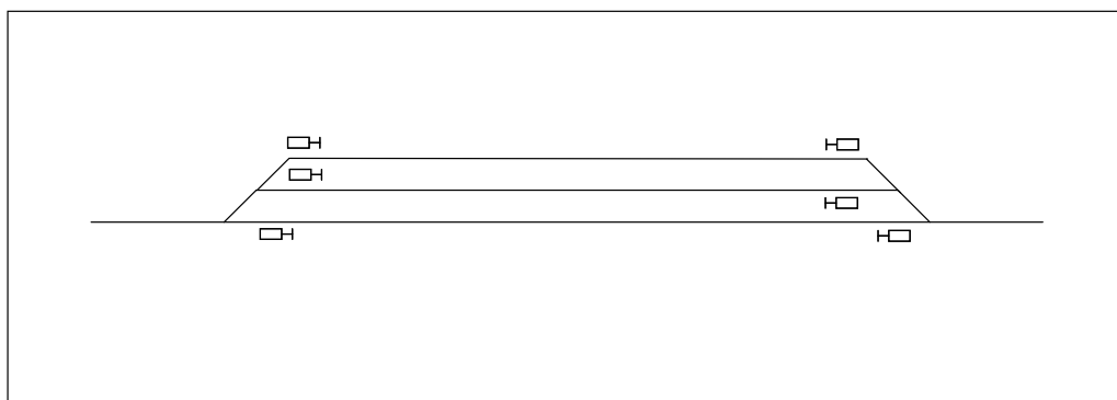
Figure 6.4:1 Positioning the signal of the leftmost track of a railway operating location to the left of the track.
