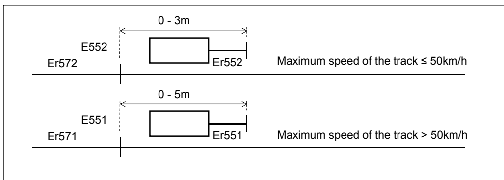
Figure 6.4:15 Positioning a main signal in respect to rail insulation.
