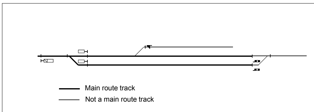
Figure 6.4:79 Replacing a main or shunting signal by an 'End of main route' indicator.
