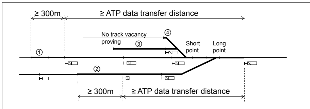
Figure 6.3:21 Signal approach zone. The numbers refer to the above-mentioned requirements.
