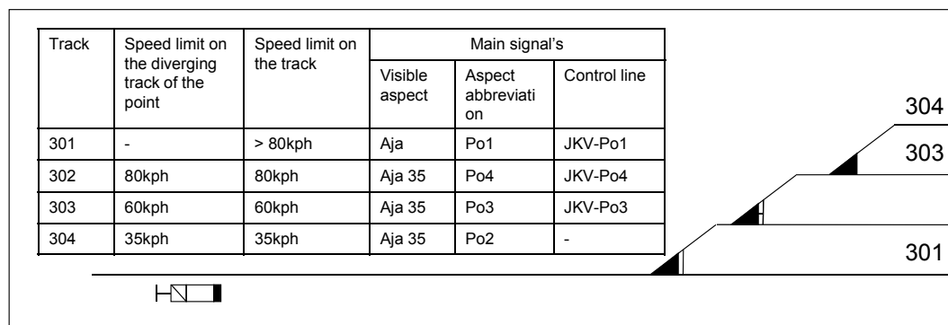
Figure 6.2:1 Example of using control lines 'JKV-Po1', 'JKV-Po3' and 'JKV-Po4'.
