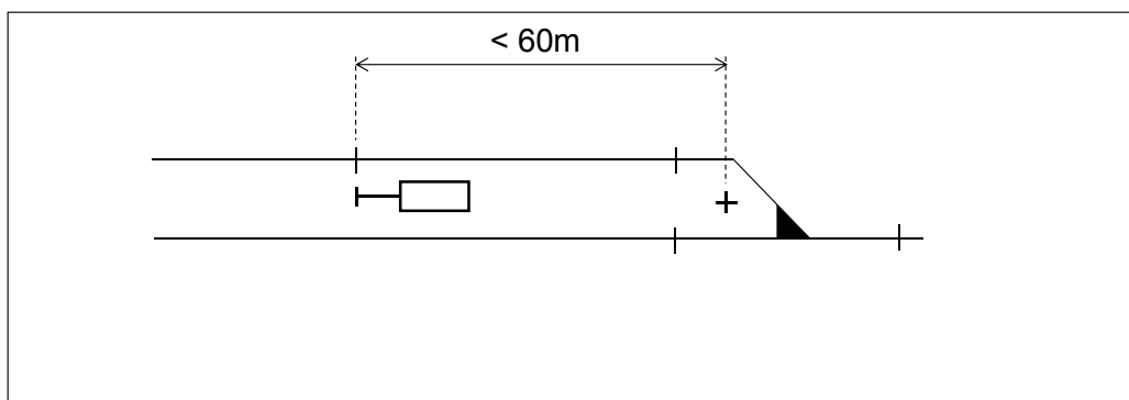
Figure 6.3:14 Only the primary overlap on the route.
