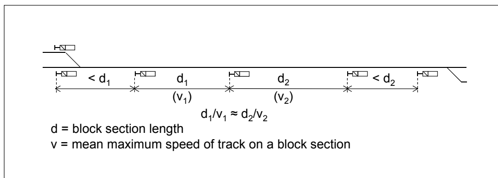
Figure 6.4:29 The length of consecutive block sections on the line.
