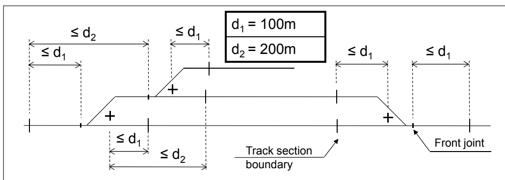
Figure 6.4:55 The location of the powered point and the track section boundary of the point in question in respect to the point.
