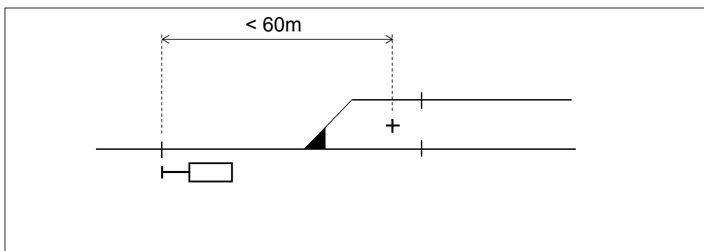
Figure 6.3:16 The route has the primary overlap and the secondary overlap.
