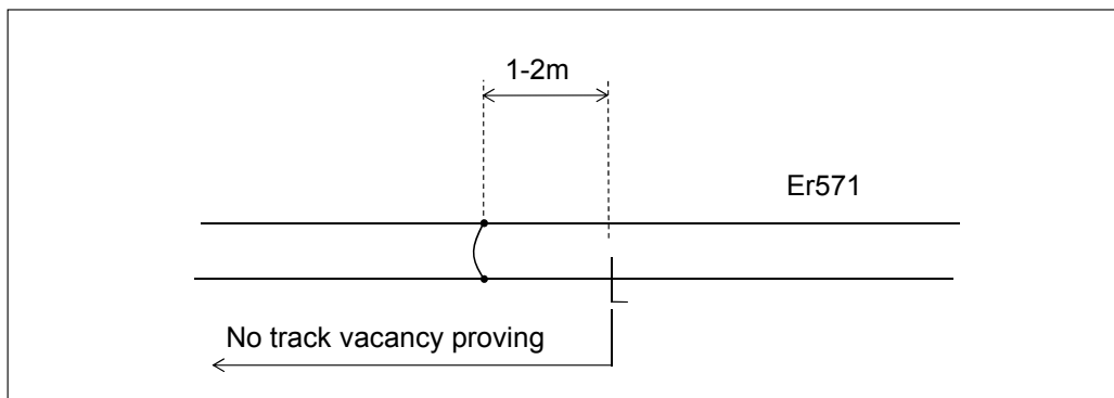
Figure 6.6:3 Short cut of the rails outside the track vacancy proving, when the track vacancy proving realized with track circuits ends.
