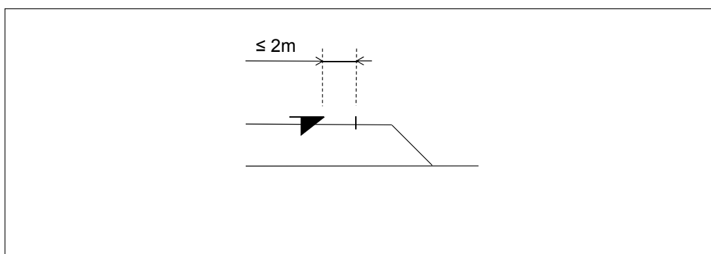
Figure 6.4:64 Positioning a derailer equipped with a hand lever in respect to the track section of the point to be protected.
