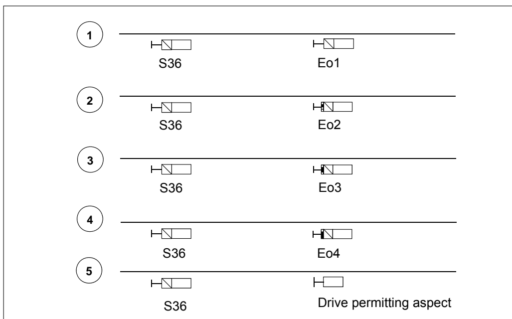
Figure 6.2:11 Examples of transmitting the fictive aspect 'S36' to ATP. The types of the signals may vary.
