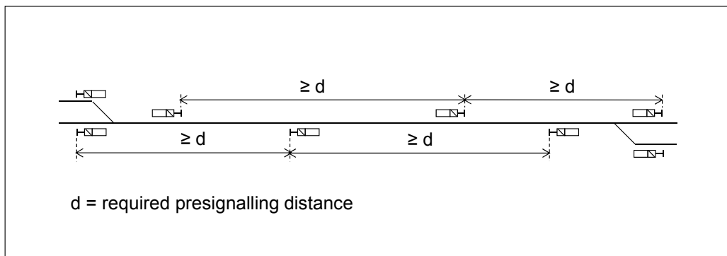
Figure 6.4:28 Dividing the track into sections between route point protecting main signals.
