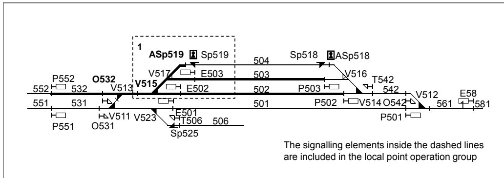
Figure 6.3:28 A local point operation group. The codes of the signalling element included in local point operation group and the code of the shunting signal displaying an 'No aspects' aspect are in boldface.
