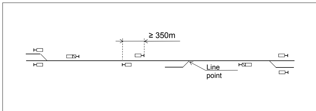
Figure 6.4:34 The distance between main signals of different directions on the line, when there is a line point on the block section started by one or both main signals.
