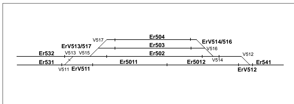
Figure 6.4:70 Determining track section codes.
