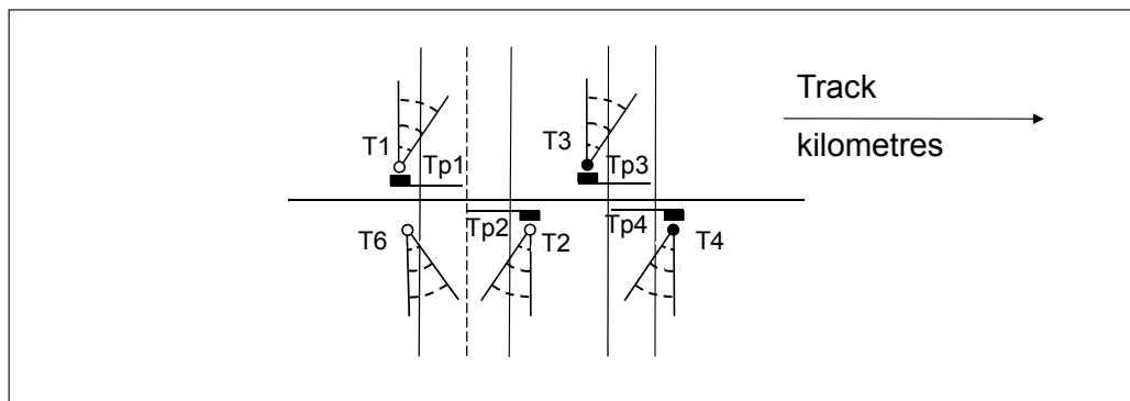
Figure 6.5:7 Barrier codes.
