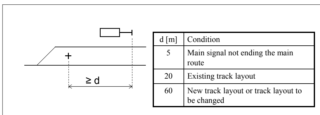
Figure 6.4:17 The main signal distance from the fouling sign point of a route point in advance of the signal.
