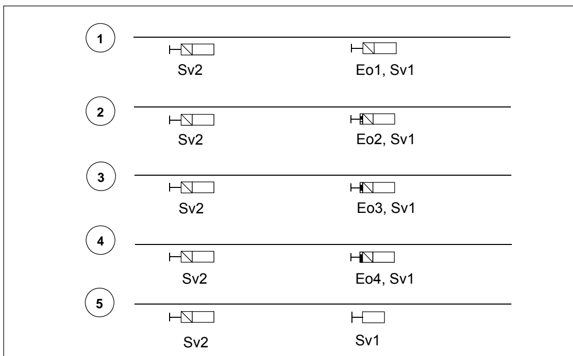
Figure 6.2:14 Examples of transmitting the fictive signal 'Sv2' to ATP. The types of the signals may vary.
