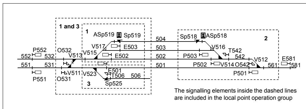
Figure 6.3:27 Forming a local point operation group.
