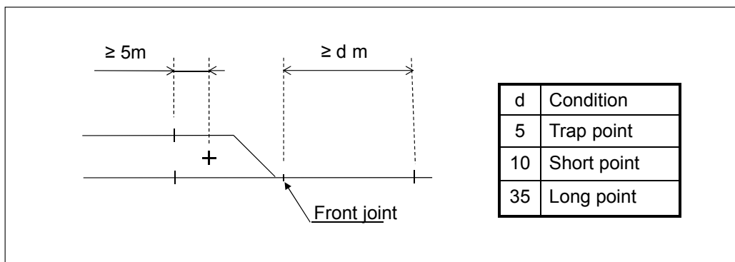
Figure 6.4:56 The distance between the point and the track section boundary of a powered point.
