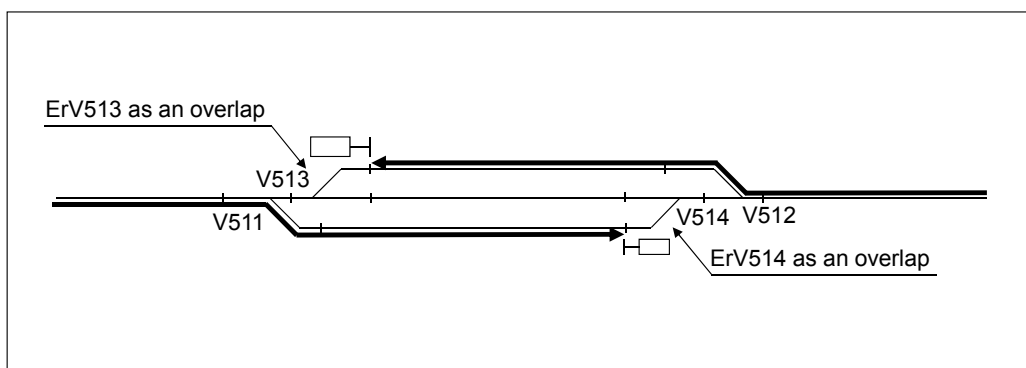
Figure 6.4:59 Taking simultaneous routes into account in positioning point track sections.
