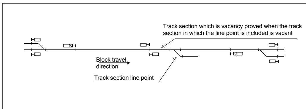
Figure 6.3:25 The conditions for the key box permission of the line point when the line point is located elsewhere than on the first block section with respect to the block travel direction.
