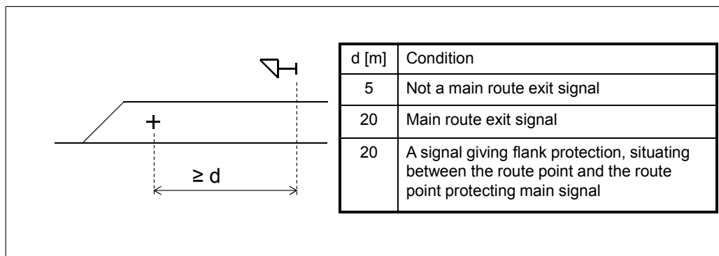
Figure 6.4:45 Positioning a shunting signal in respect to the fouling sign point of the route point.
