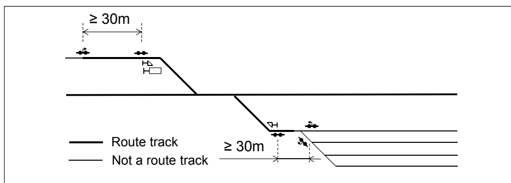
Figure 6.2:18 Track vacancy proving of a track associated with route point.
