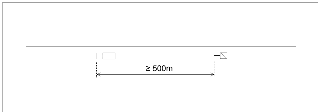
Figure 6.4:32 The main signal distance from the separate distant signal in advance of the main signal.
