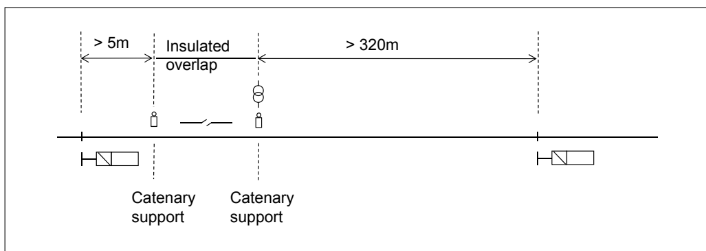
Figure 6.4:24 Positioning a main signal in the vicinity of an insulated overlap.
