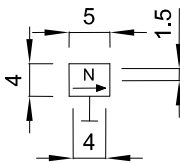
Border sign for state railway net
