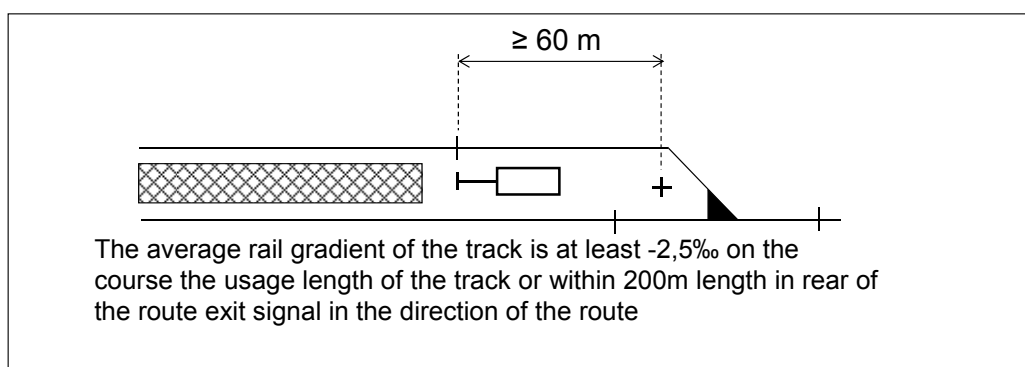
Figure 6.3:9 Overlap 0 and primary overlap on the route.
