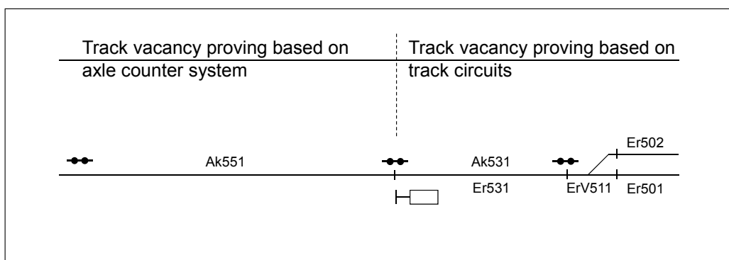
Figure 6.4:68 Track vacancy proving at the train control system's interface.
