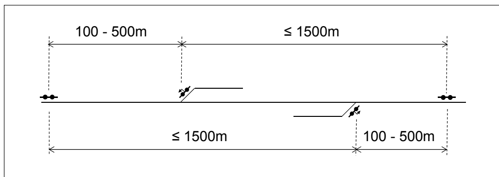
Figure 6.4:72 The line point track section location in respect to the line point.
