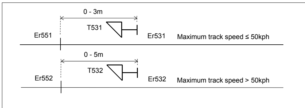
Figure 6.4:43 Positioning a shunting signal in respect to rail insulation.
