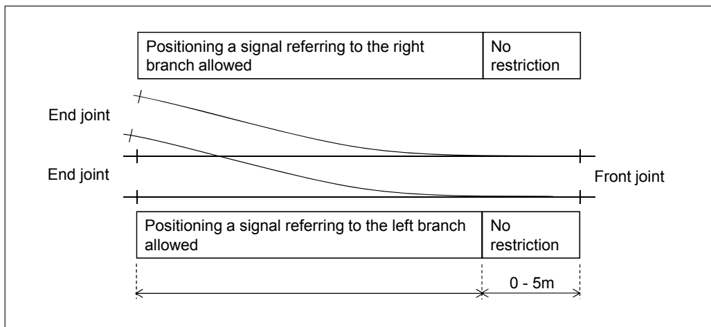
Figure 6.4:5 Positioning a signal at a point other than a route point.
