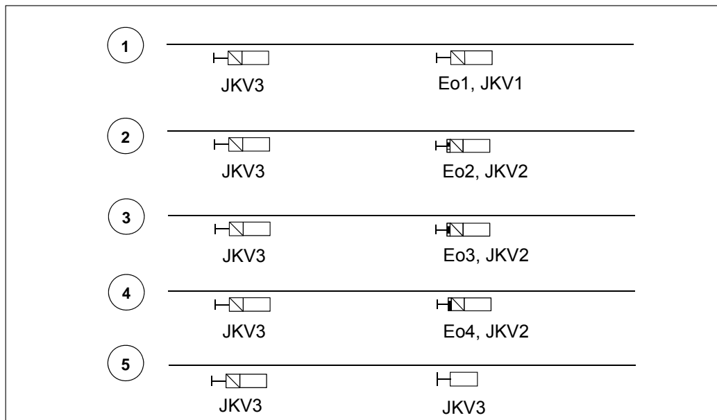
Figure 6.2:4 Examples of activation of control line 'JKV3'. The types of the signals may vary.
