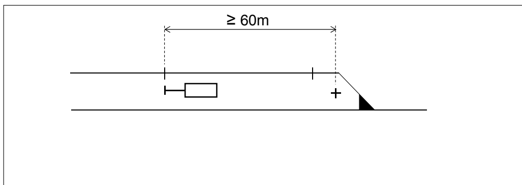
Figure 6.3:13 Only the primary overlap on the route.
