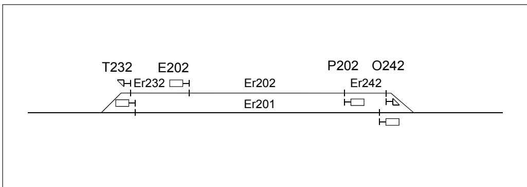
Figure 6.4:50 Using the shunting signal to extend the working length.
