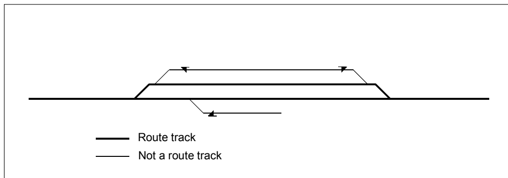
Figure 6.4:61 Protecting a route track with a derailer.
