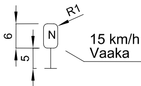
Speed limit -sign for special object (speed and reason for limit shall be stated with text on the index line)
