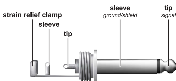
Fig. 4.3: 1/4" TS connector
