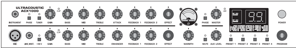
Fig. 2.1: The front panel of the ULTRACOUSTIC
