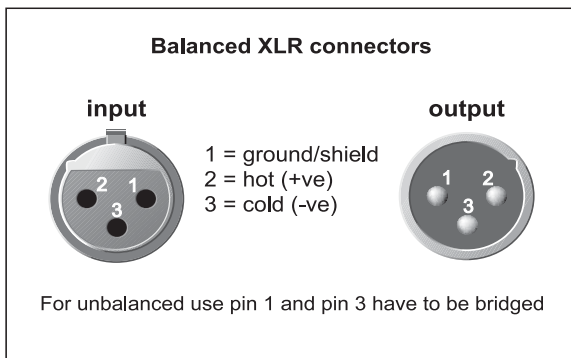
Fig. 4.1: XLR connections
