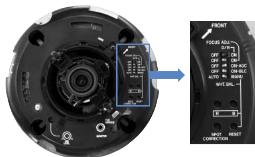
Cover inside
