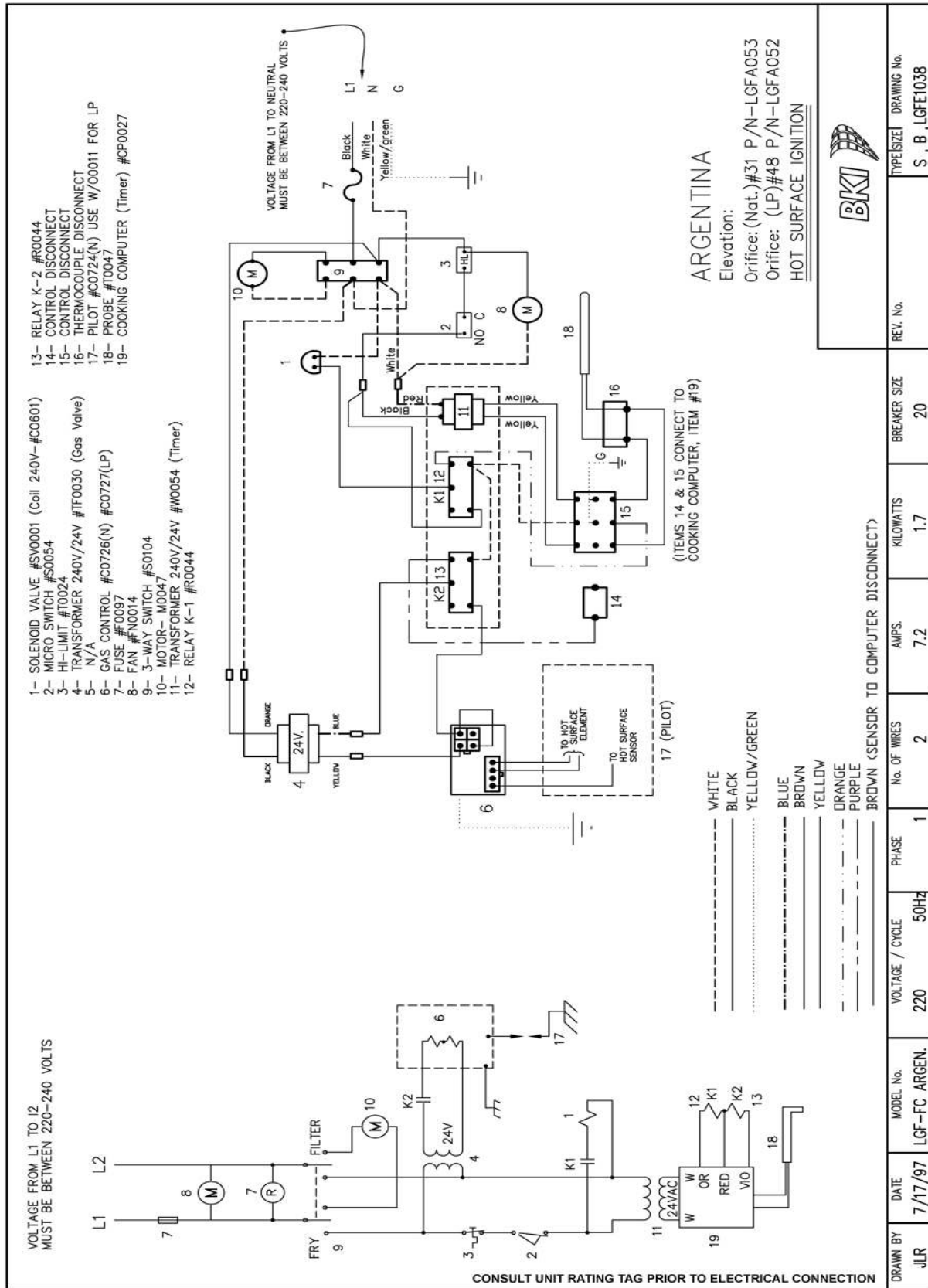
Figure 19. LGF-FC 220V/50HZ/1Ph
