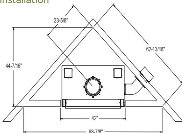
Top View Corner Installation
