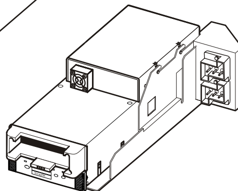
Tray Assembly for Libraries L180/L700/L1400
