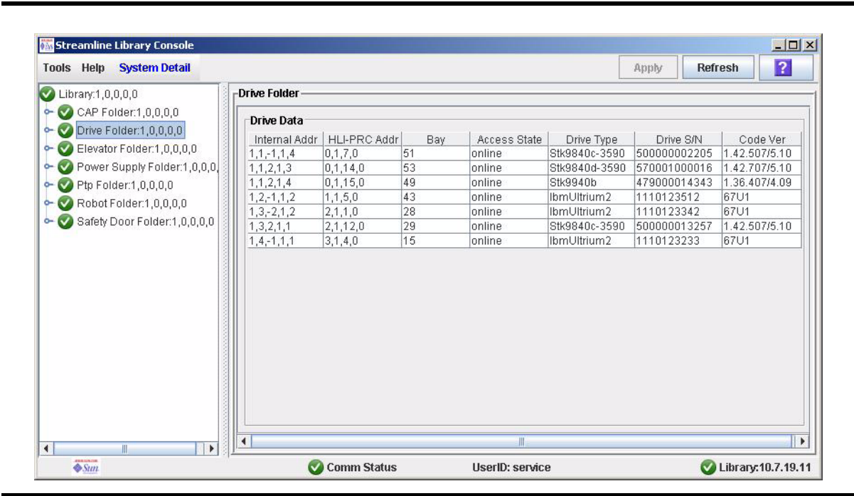
FIGURE 2-5 SL8500 SLC Drive Folder Display
