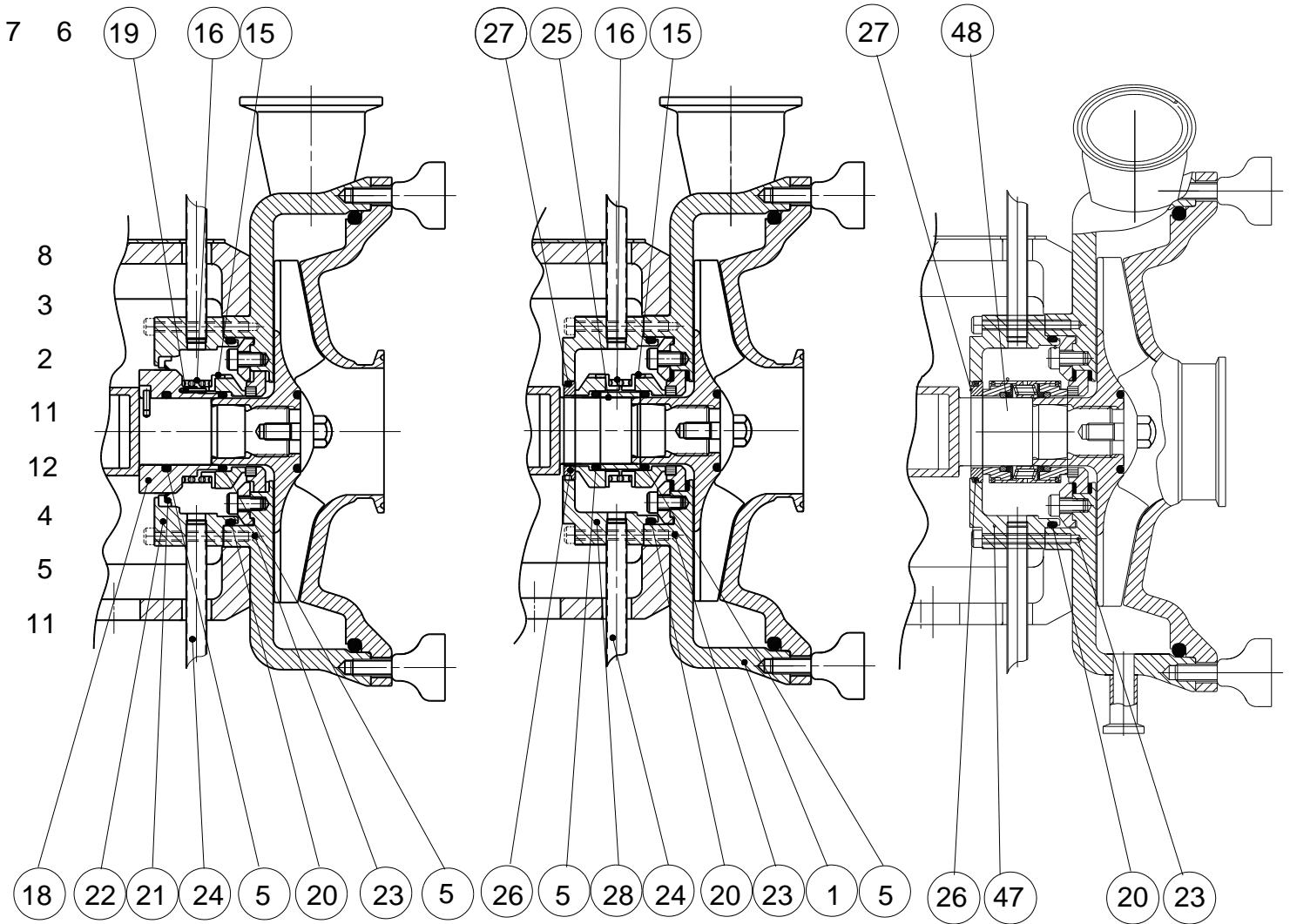
TYPE FG-WATER COOLED SINGLE SEAL
