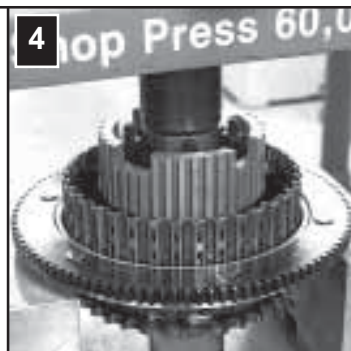
Carefully align the Pro-Clutch™ hub.
