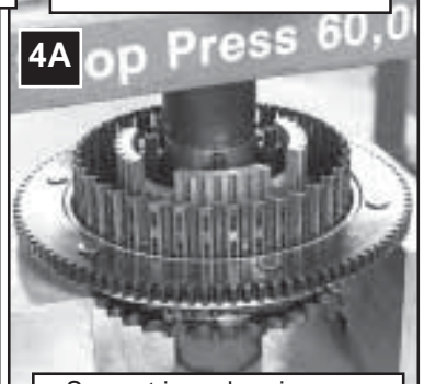
Support inner bearing race
