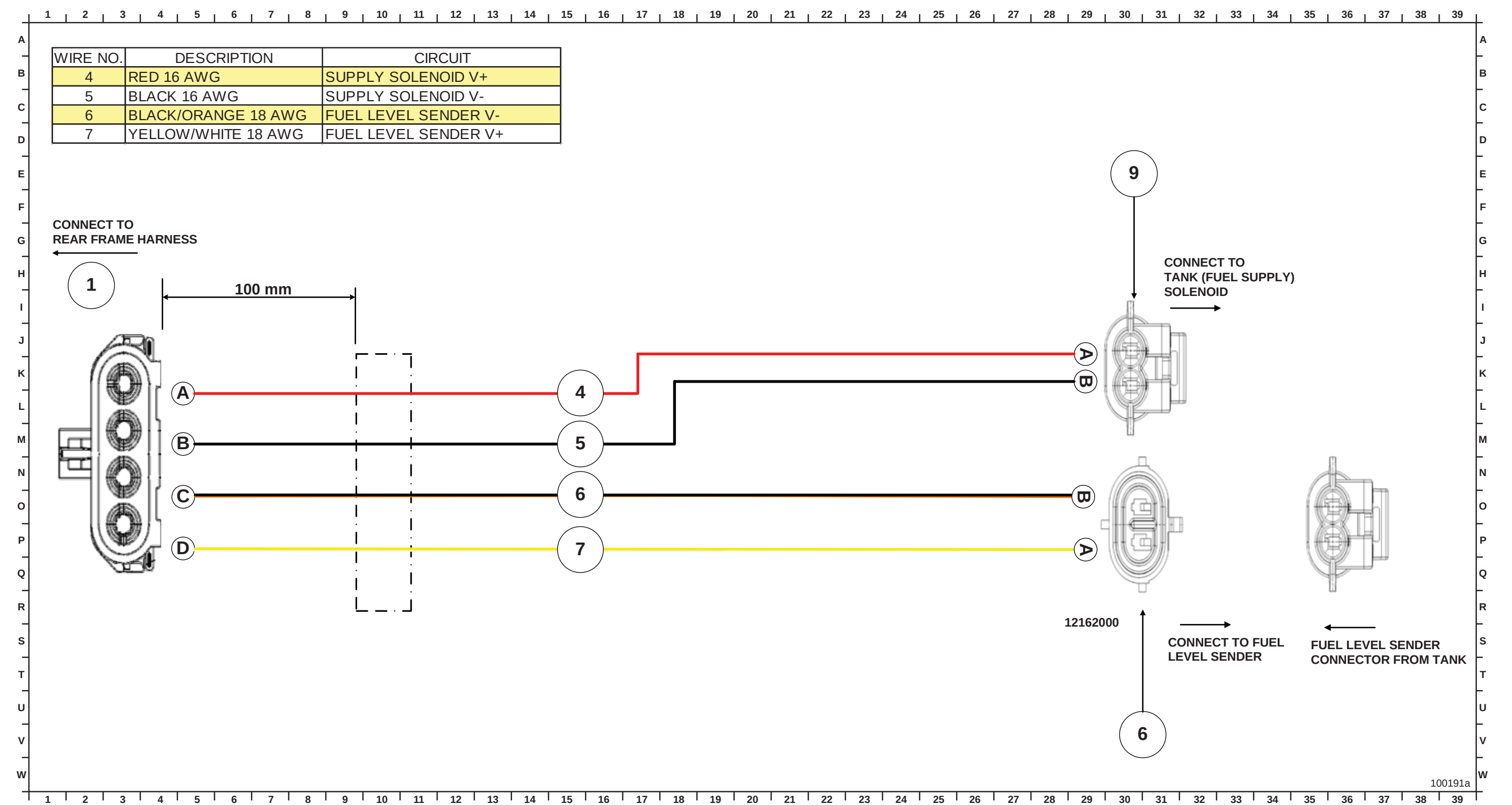
F-250/350 Pickup, F-450/550 and F-650, Tank Solenoid Harness Electrical Schematic
