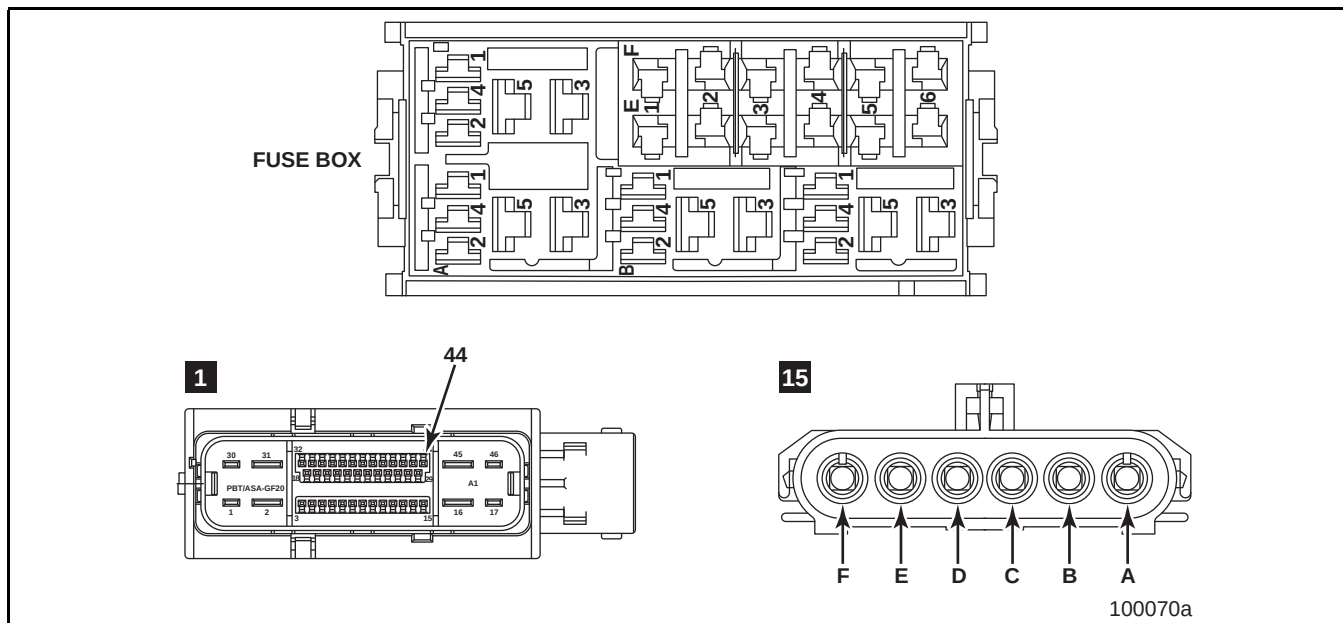
Figure 1 — Underhood Harness Connectors
