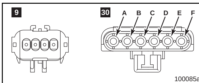
Figure 16 — Rear Frame Harness Connectors
