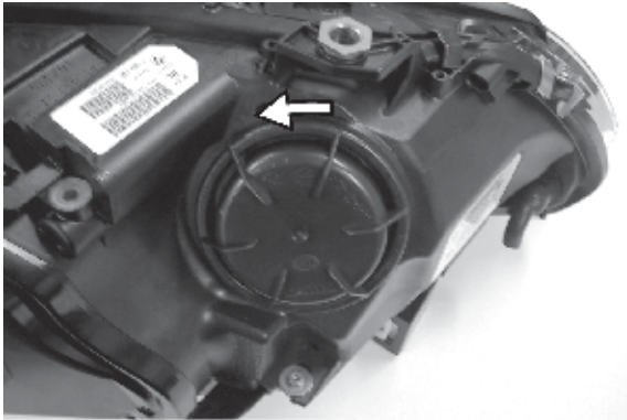
1. Remove back side cover of headlamp unit.
