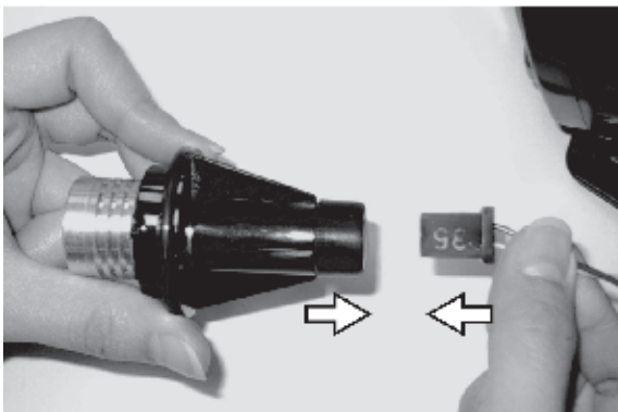
5. Connect vehicle harness connector to L.E.D. bulb.
