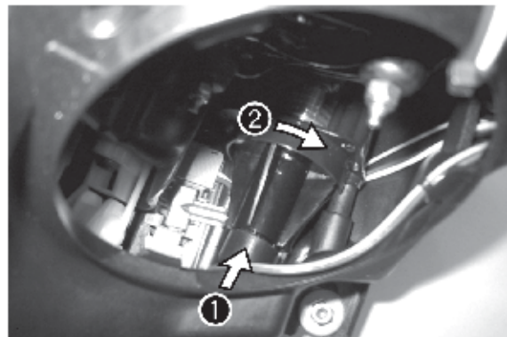
6. Install L.E.D. bulb in the original position bulb location.
