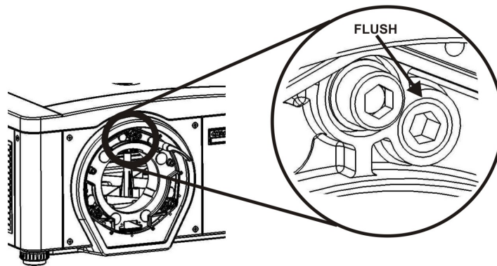
FIGURE 2-20 POSITION SETSCREW FLUSH
