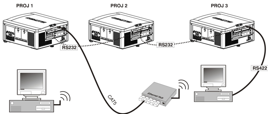
FIGURE 2-27 COMMUNICATING TO ALL PORTS
