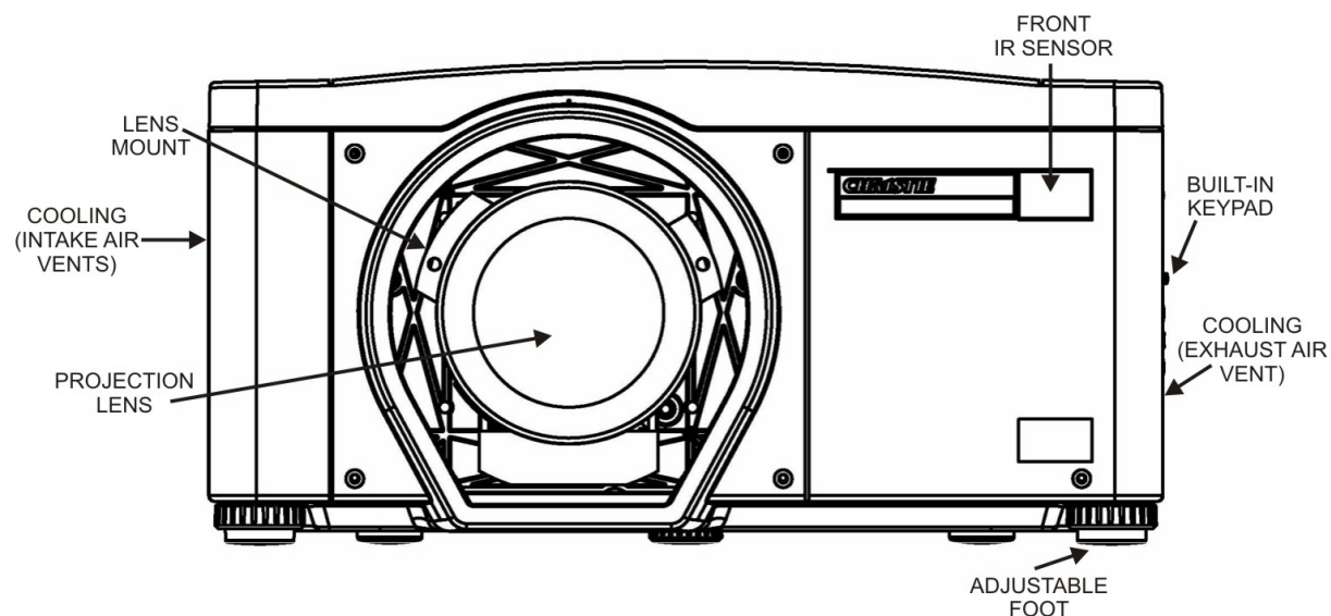
FIGURE 2-8 ABOUT THE PROJECTOR - FRONT VIEW
