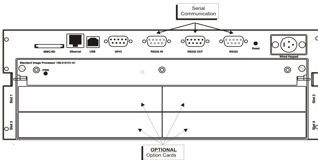
FIGURE 2-28 INPUT PANEL
