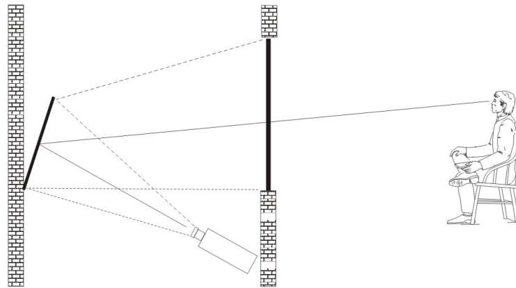
FIGURE 2-16 FOLDED OPTICAL PATH
