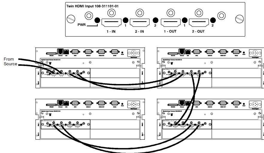
FIGURE 2-31 2x2 WIRING SOLUTION
