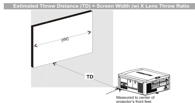
FIGURE 2-11 THROW DISTANCE
