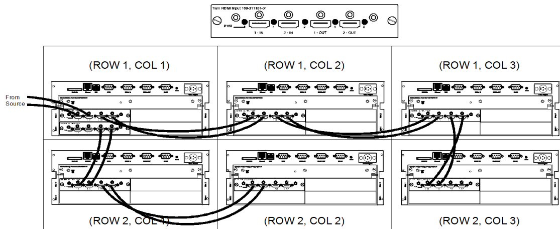
FIGURE 2-32 2x3 LOOP-THROUGH WIRING SOLUTION
