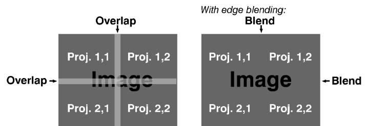
FIGURE 3-37 EDGE BLENDING CONCEPT
