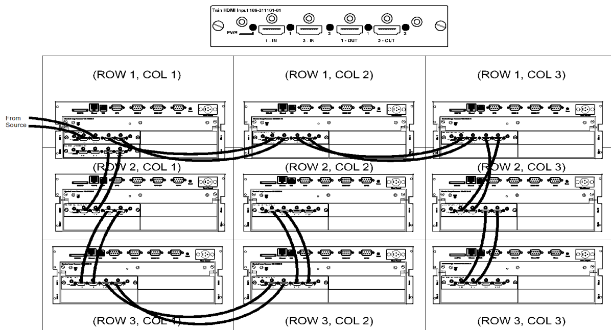
FIGURE 2-34 3X3 LOOP-THROUGH WIRING SOLUTION
