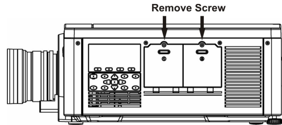
FIGURE 5-2 REPLACE LAMP
