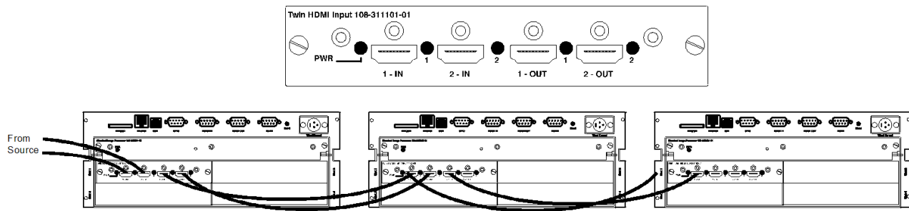
FIGURE 2-30 1x3 WIRING SOLUTION
