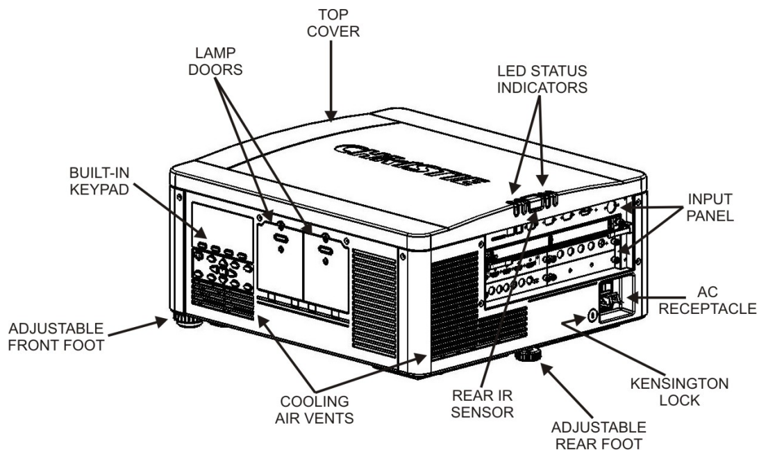
FIGURE 2-7 ABOUT THE PROJECTOR - REAR/SIDE VIEW
