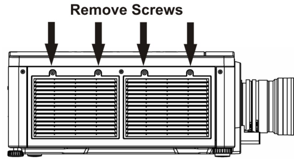
FIGURE 5-1 REPLACE FILTER
