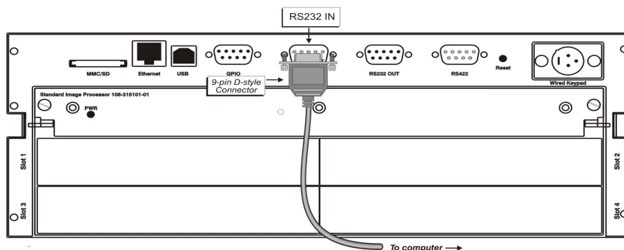
FIGURE 2-22 CONNECTING RS-232
