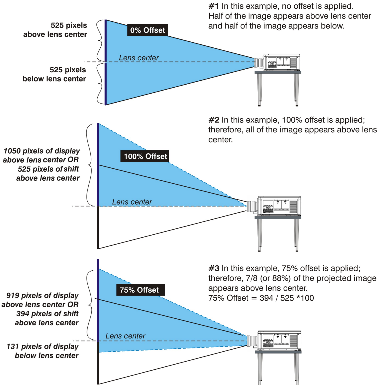
FIGURE 2-12 VERTICAL OFFSET EXAMPLES
