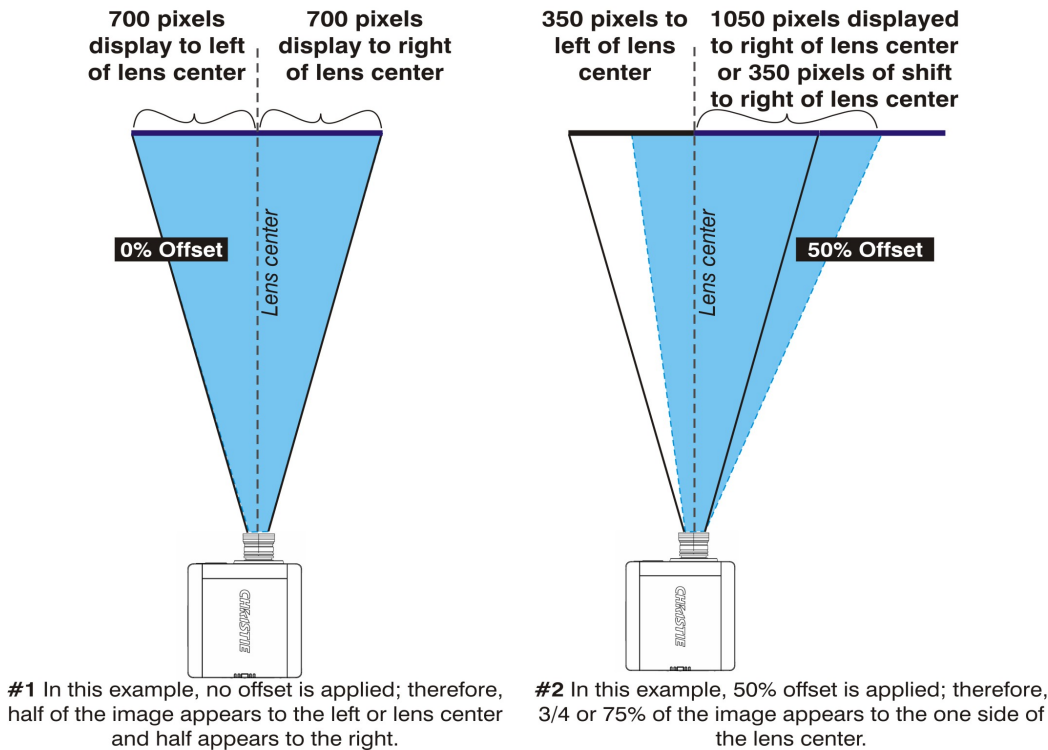
FIGURE 2-13 HORIZONTAL OFFSET EXAMPLES
