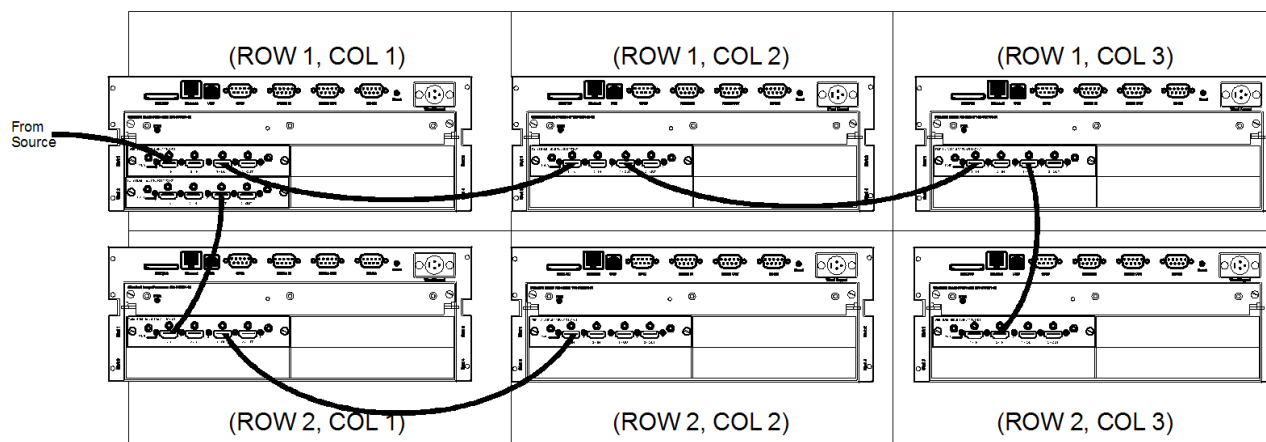
FIGURE 2-33 2X3 SINGLE WIRING LOOP-THROUGH - NO PIP IS SUPPORTED
