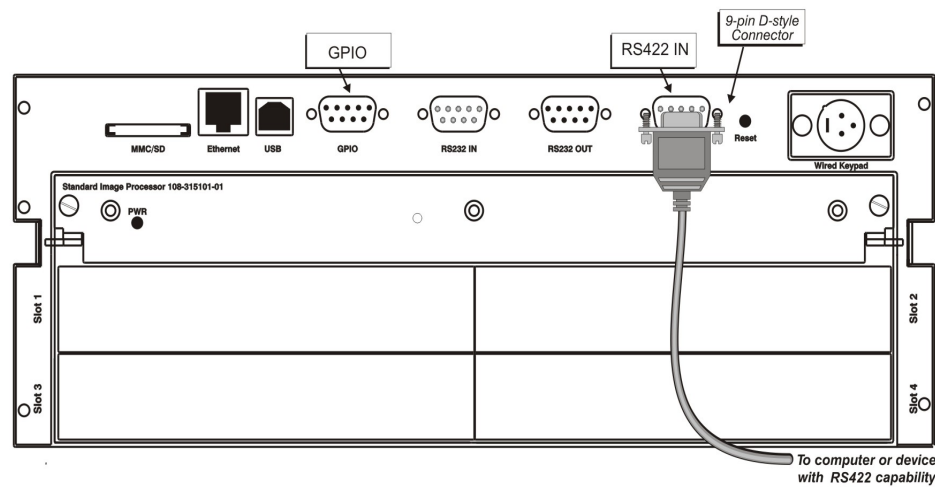
FIGURE 2-23 CONNECTING RS-422
