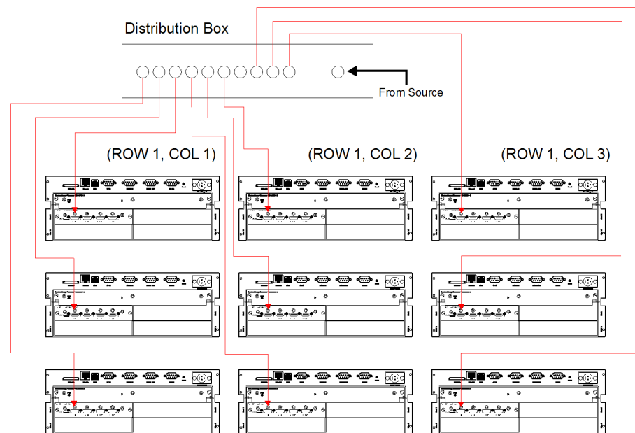
FIGURE 2-29 USE OF DISTRIBUTION BOX
