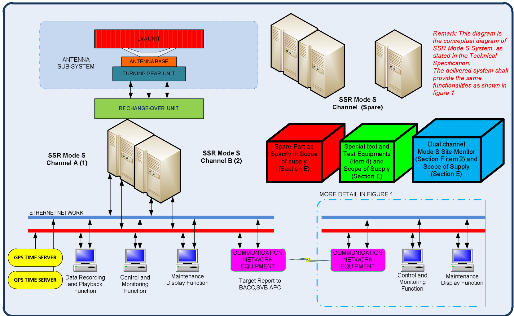
Figure 2 SSR Mode S Project Configuration.
