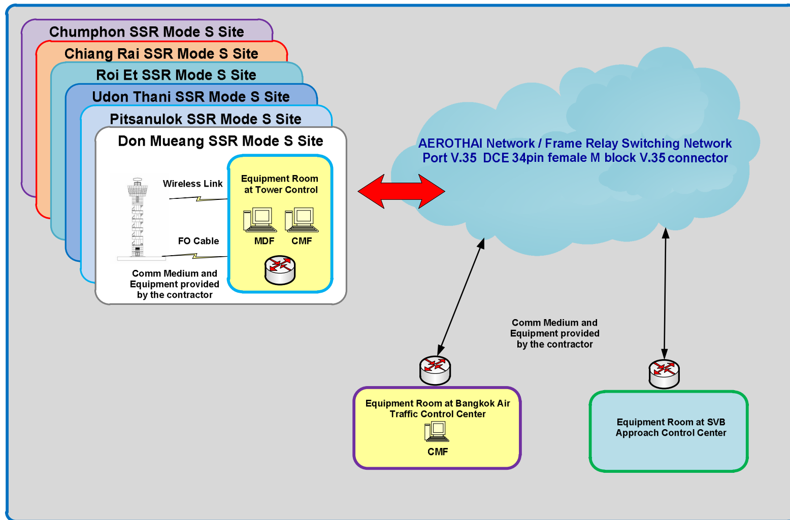
Figure 1 SSR Mode S Project Overview.
