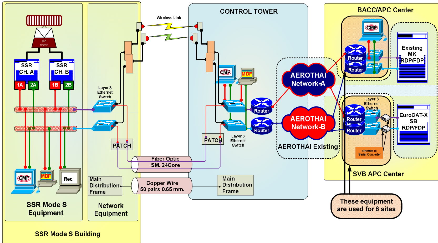
Figure 3 Network Configuration for SSR Mode S Project.
