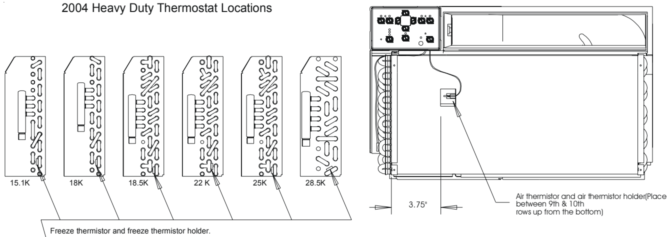
2004 Heavy Duty Thermostat Locations
