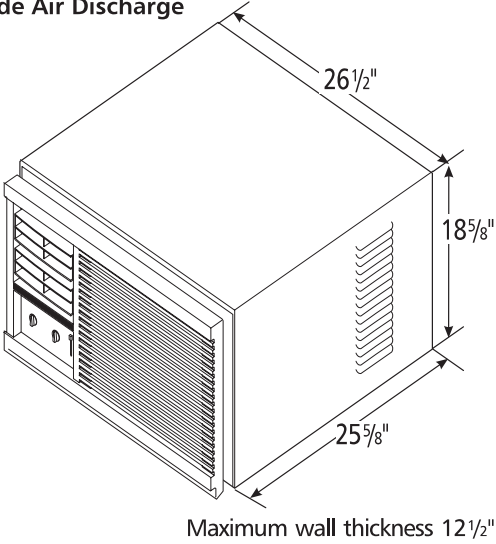
Heavy Duty Slide Out Side Air Discharge
