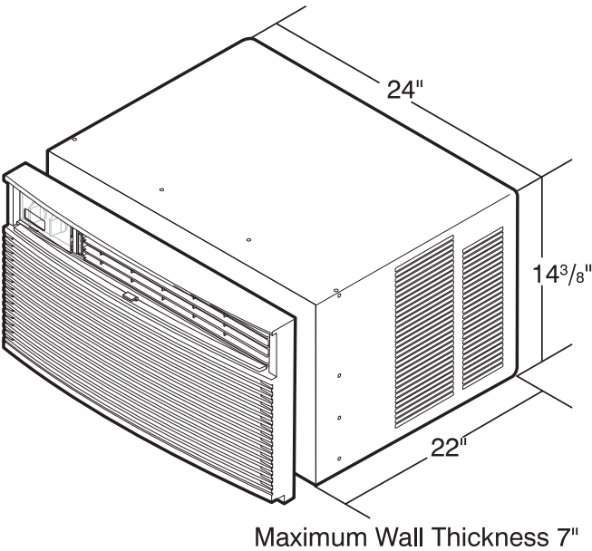
22" Top Control Intermediate
