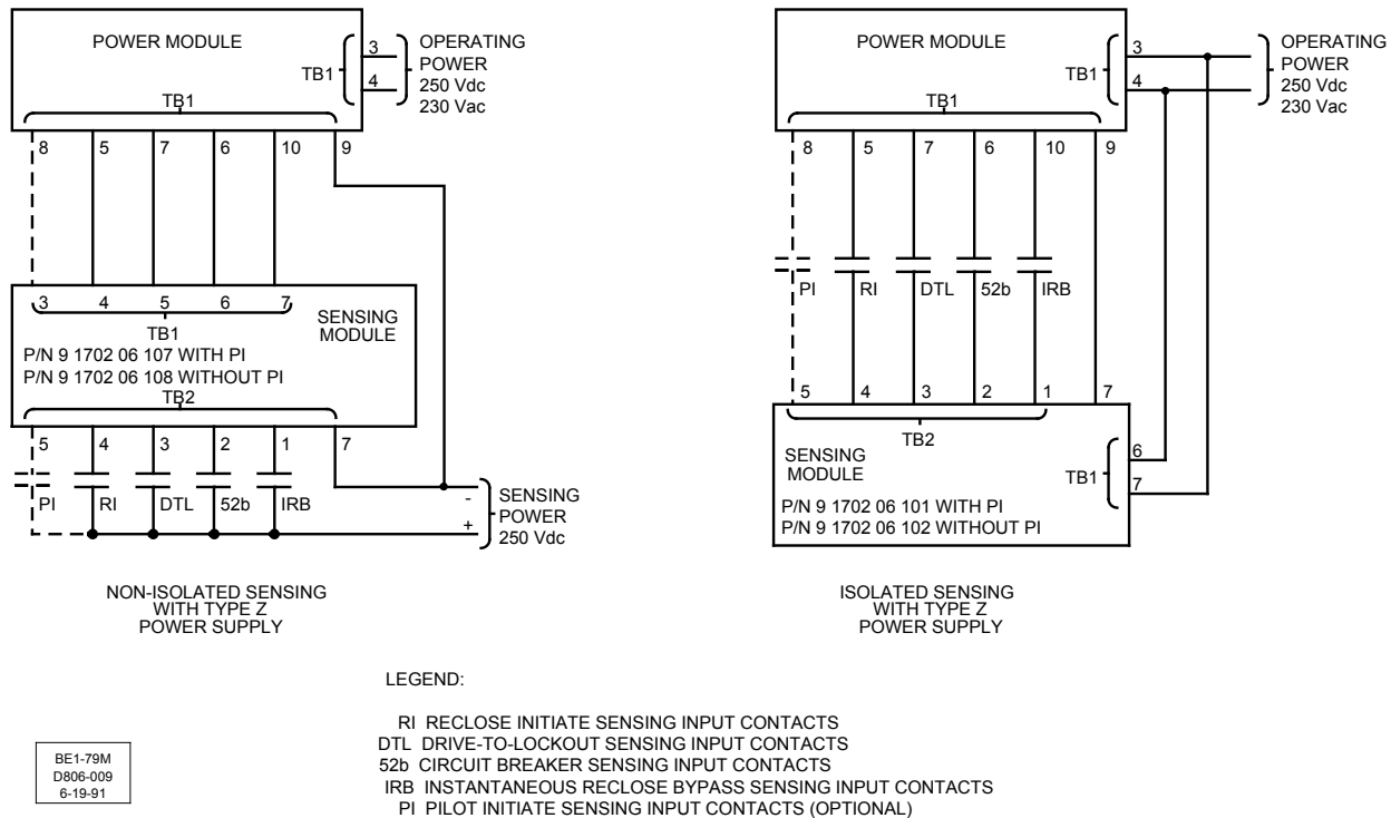
Figure 7-2. Sensing Input Connections
