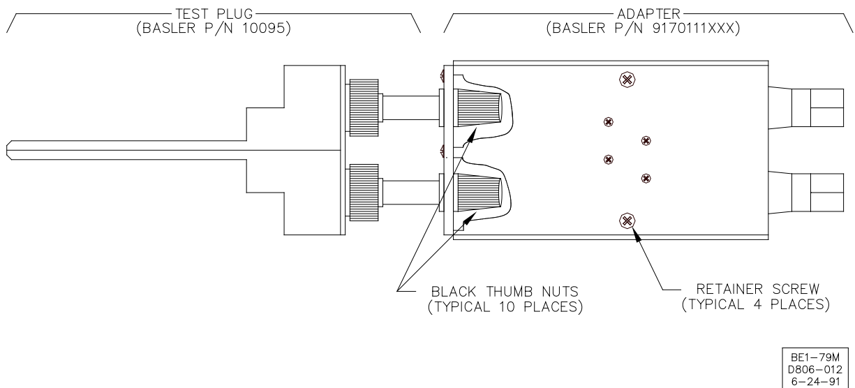
Figure 7-3. Test Plug and Adapter
