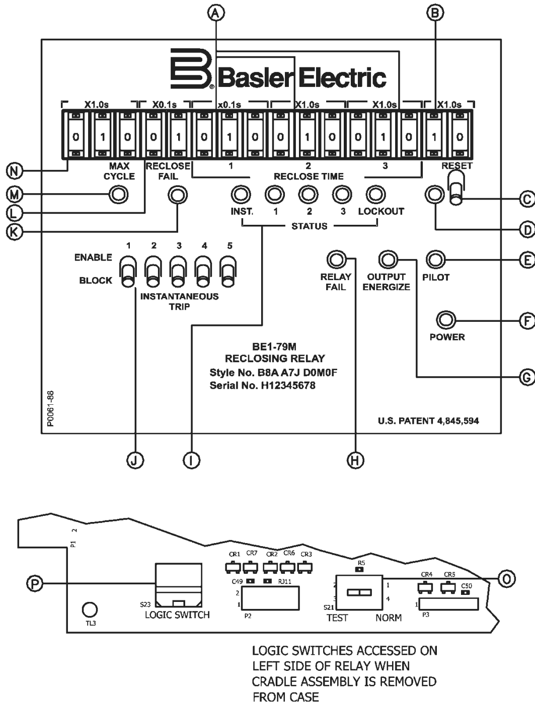
Figure 2-1. Location of Controls and Indicators
