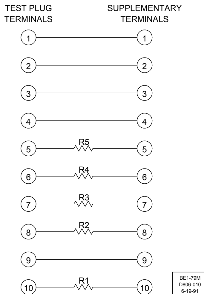
Figure 7-4. Improvised Test Setup
