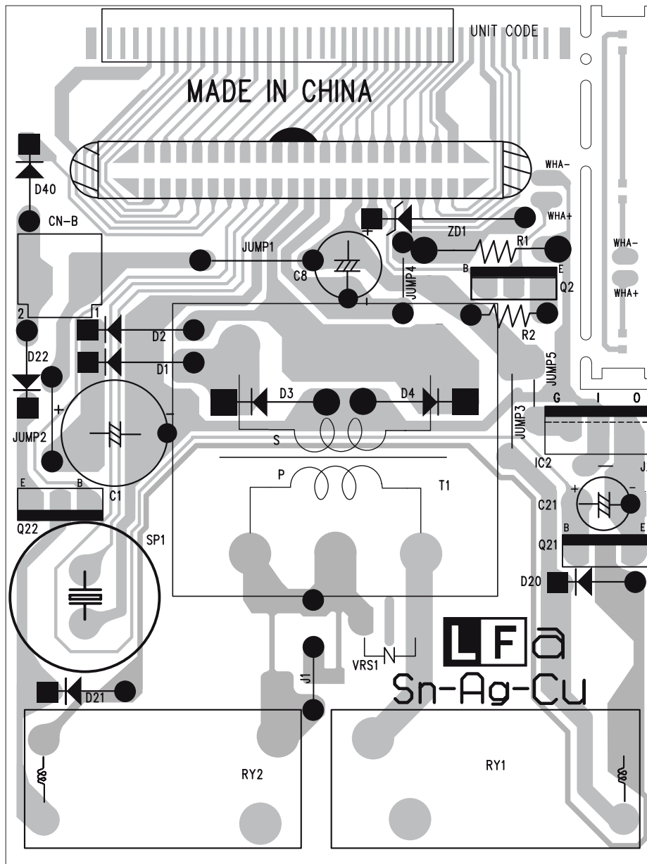
Figure S-3. Printed Wiring Board of Power Unit
