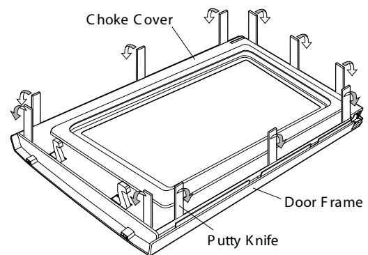
Figure C-5. Door Disassembly
