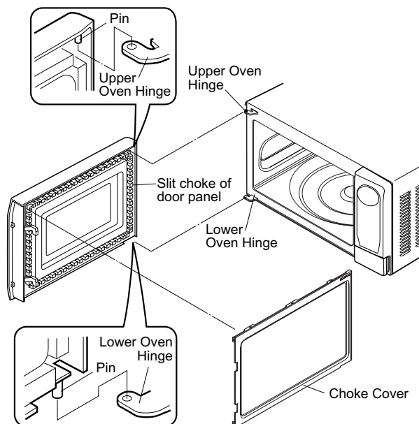
Figure C-6. Door Replacement
