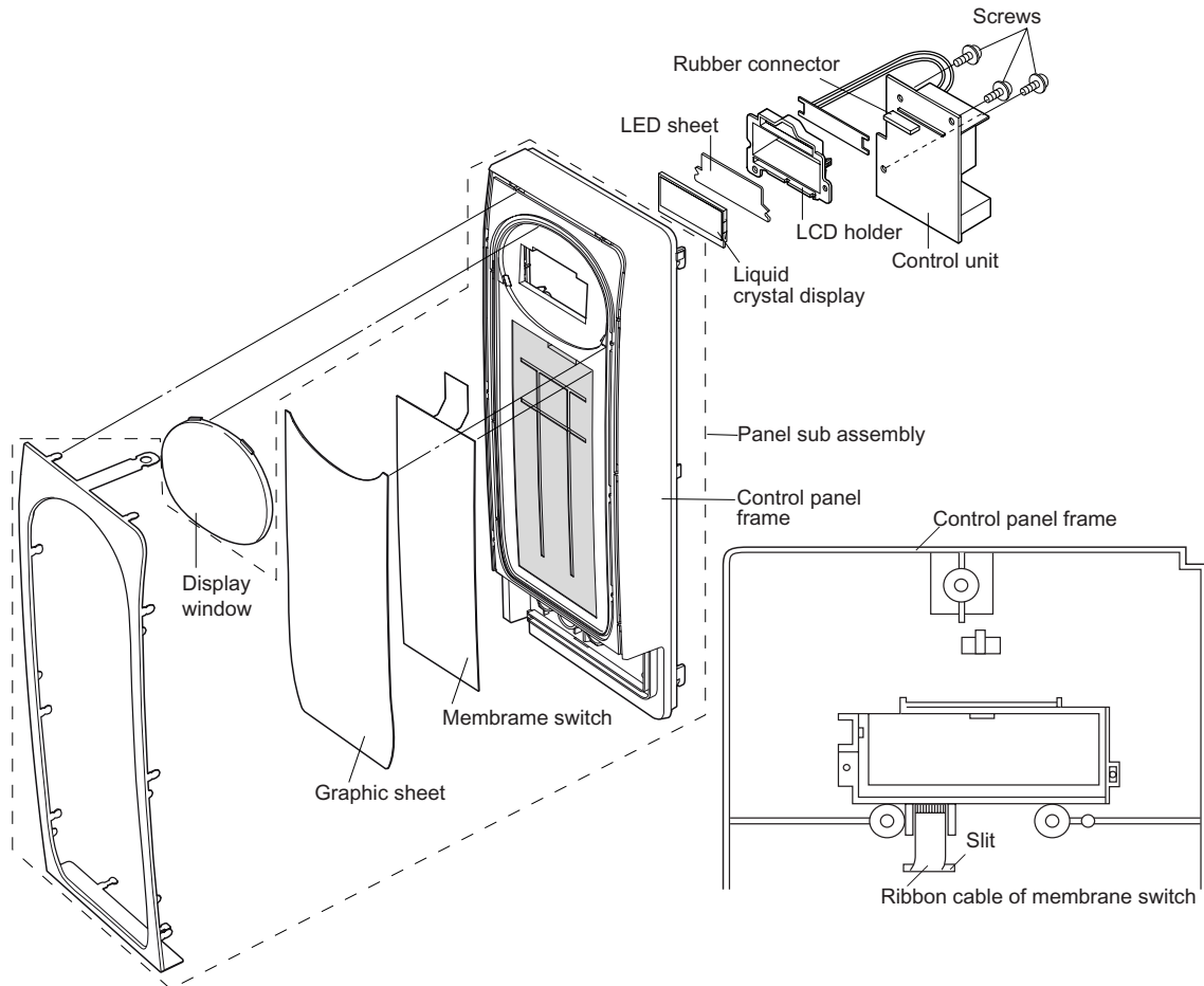
Figure C-2a Graphic Sheet and Membrane Switch Replacement
