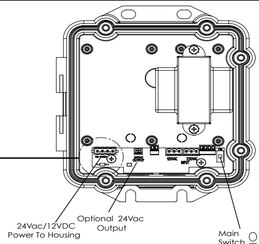
HEATERS CAMERA
