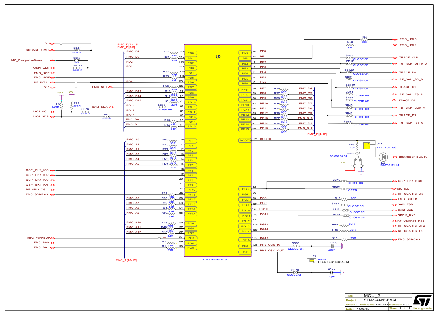
Figure 15. MCU 2
