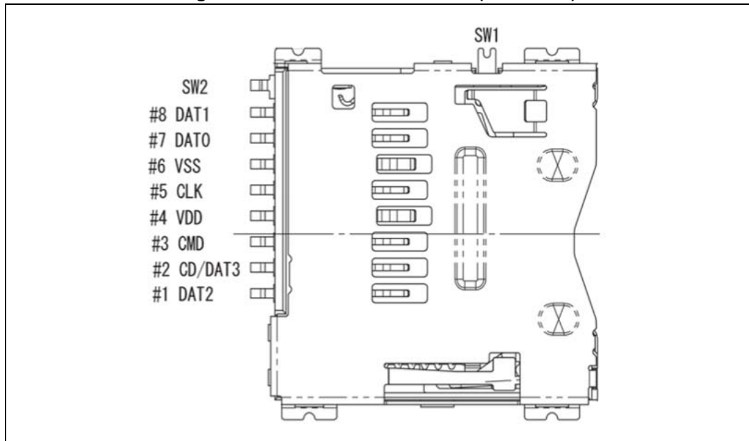
Figure 9. MicroSD connector CN4 (front view)
