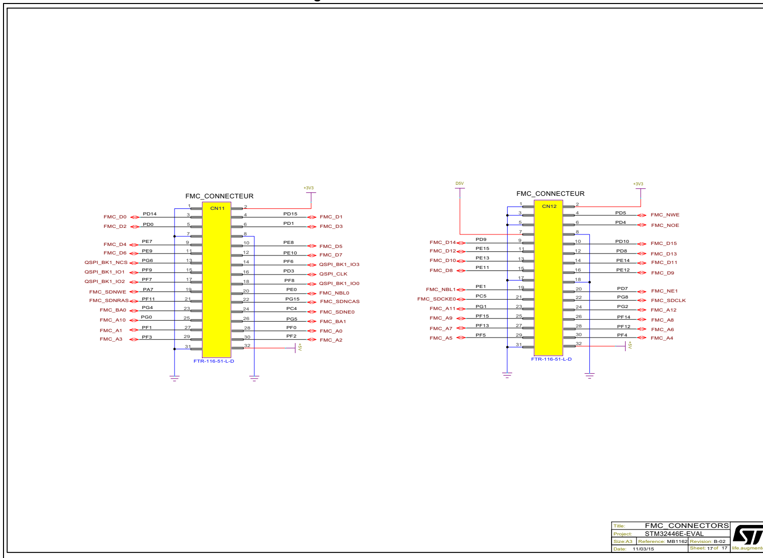
Figure 30. FMC connectors
