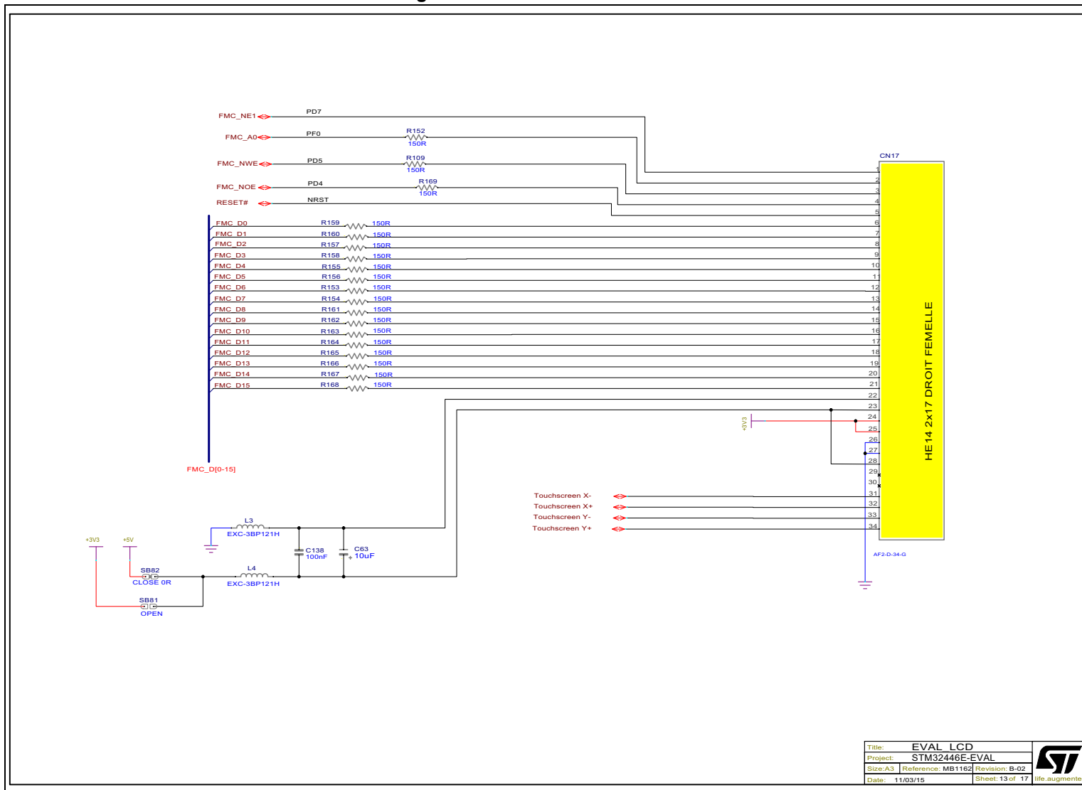
Figure 26. STM32446E-EVAL LCD
