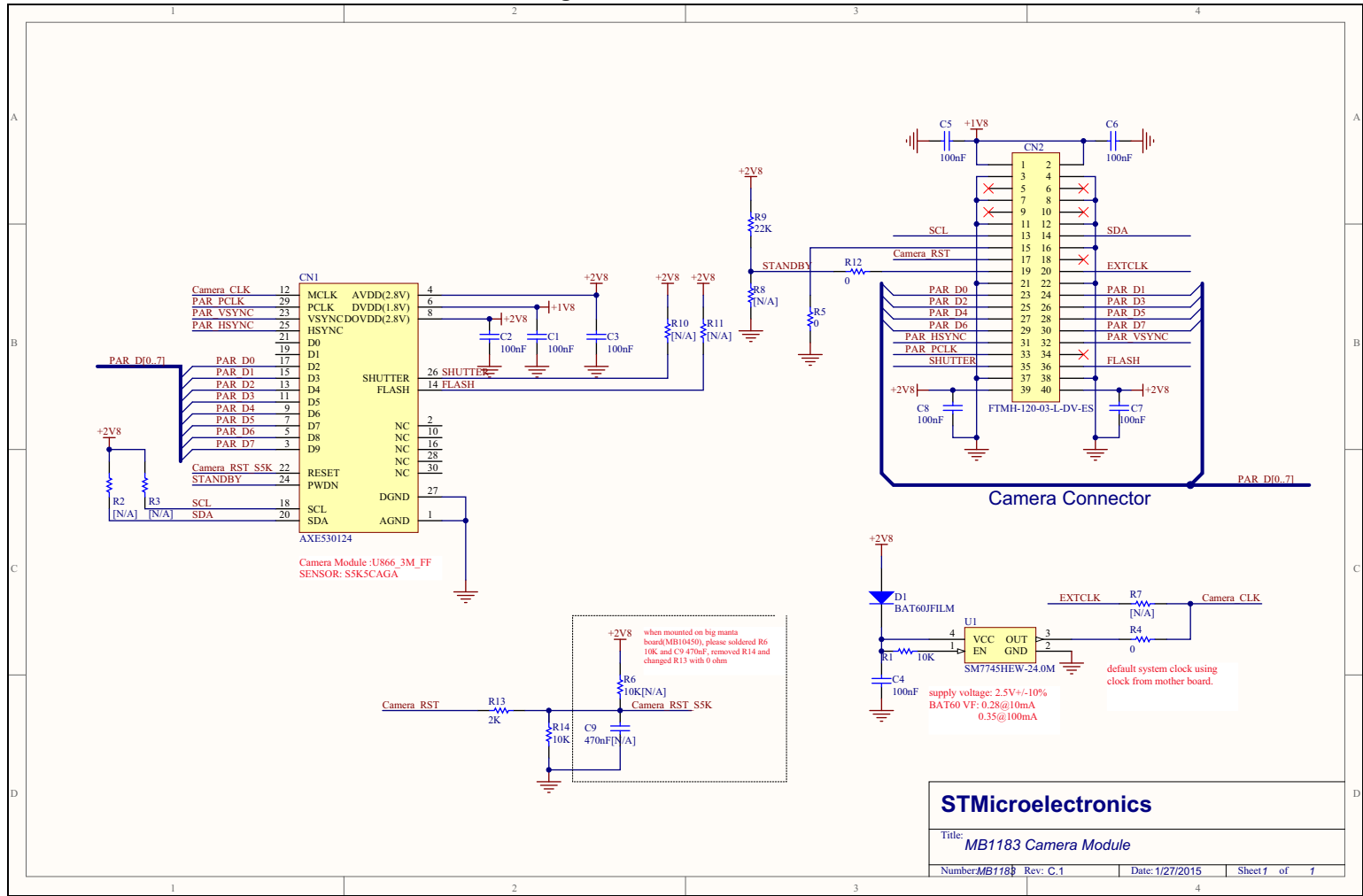
Figure 32. Camera module
