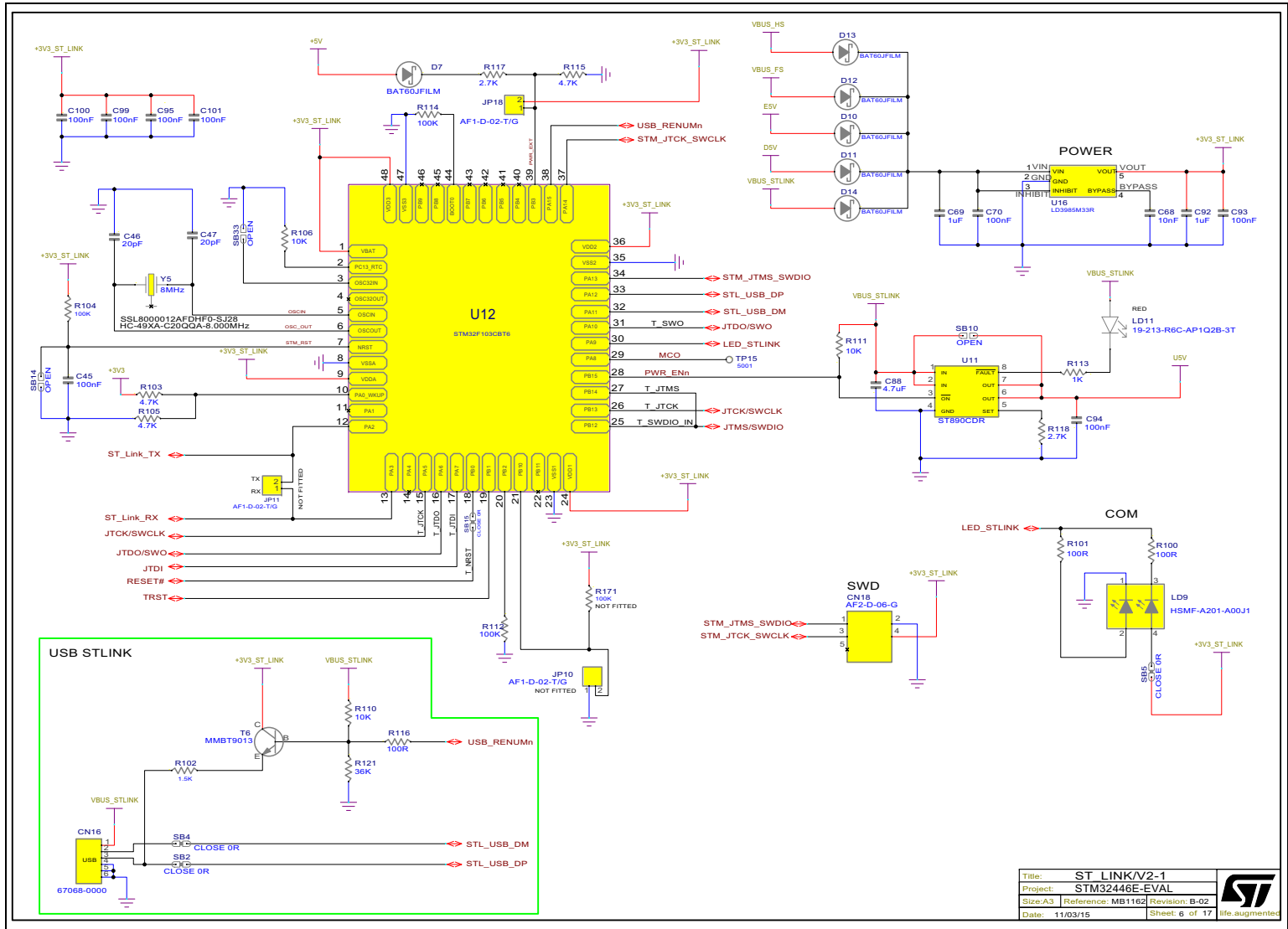
Figure 19. ST-LINK/V2-1
