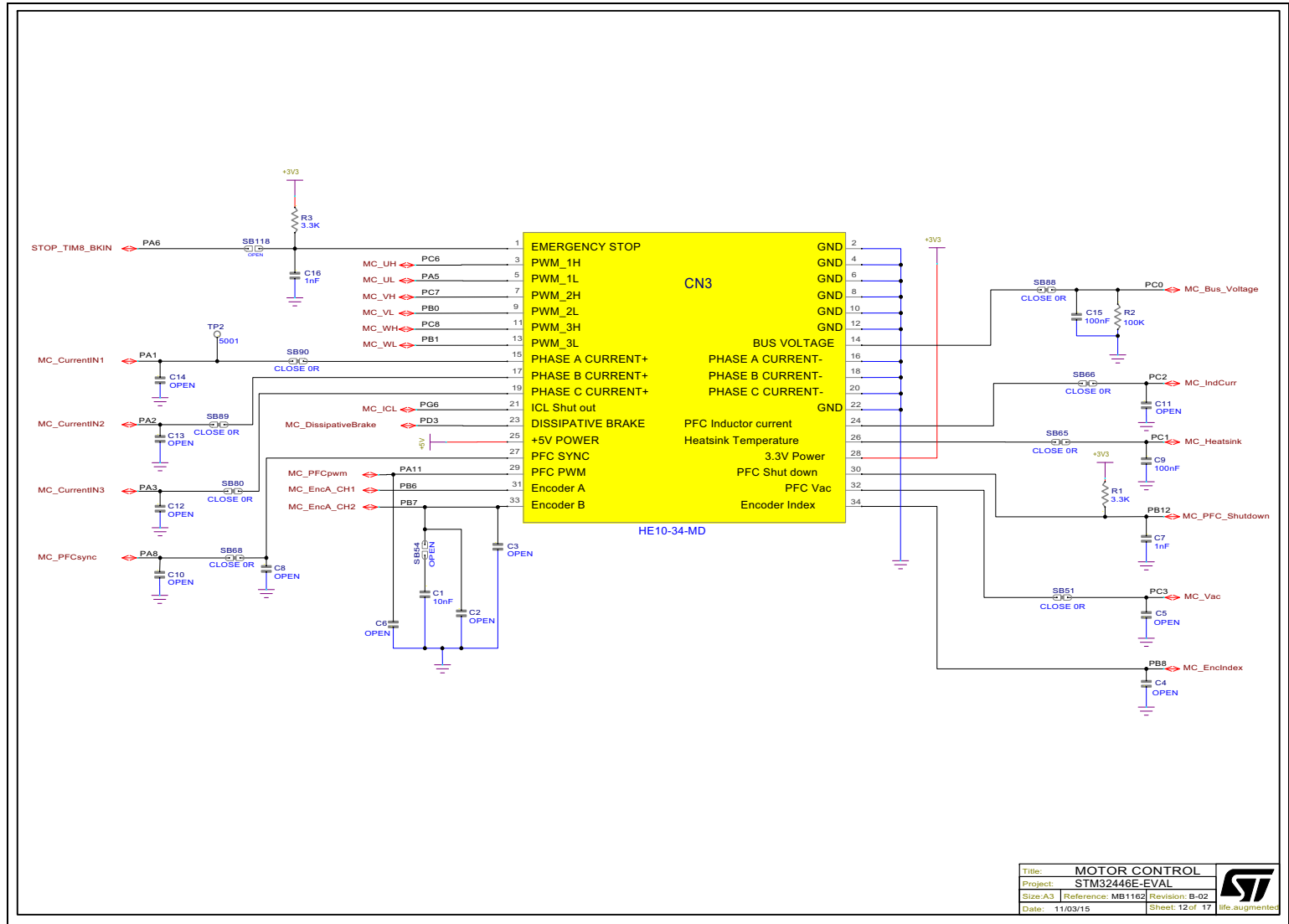
Figure 25. Motor Control
