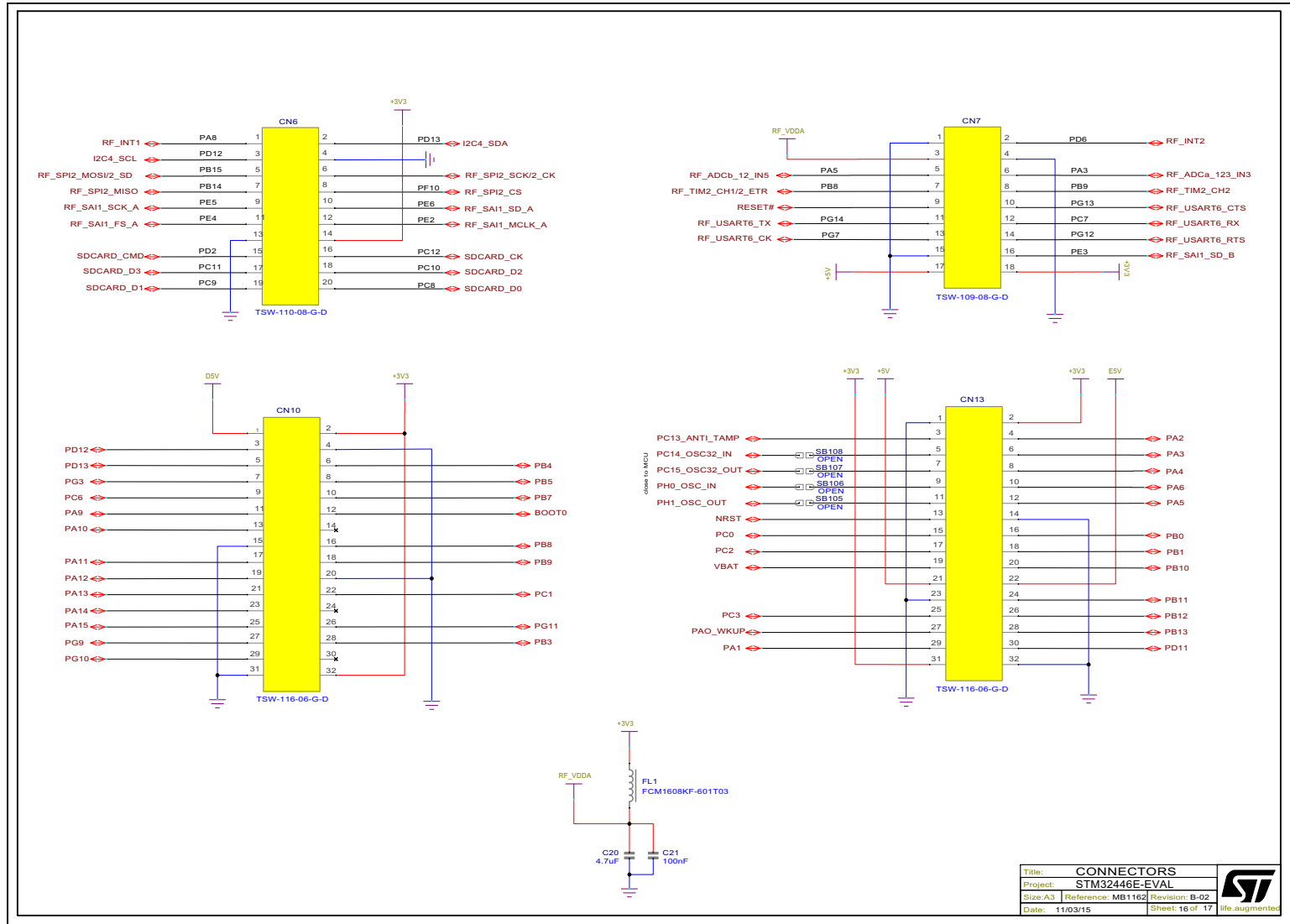
Figure 29. Connectors
