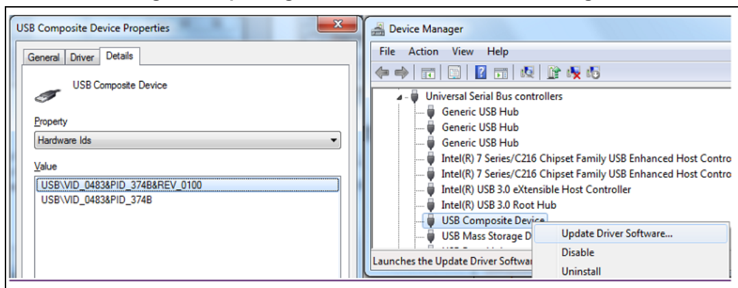
Figure 4. Updating the list of drivers in device manager
